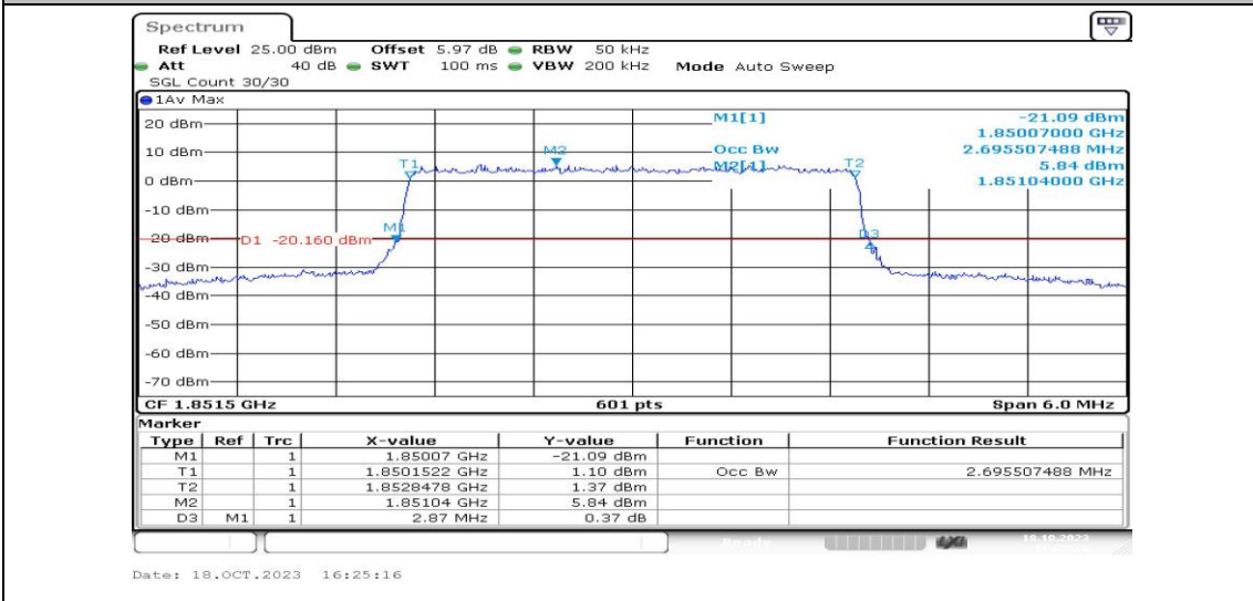
Band25-3MHz-16QAM-26055-15RB#0-PASS
