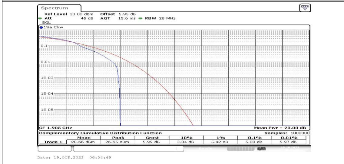
Band25-20MHz-16QAM-26590-1RB#0-PASS
