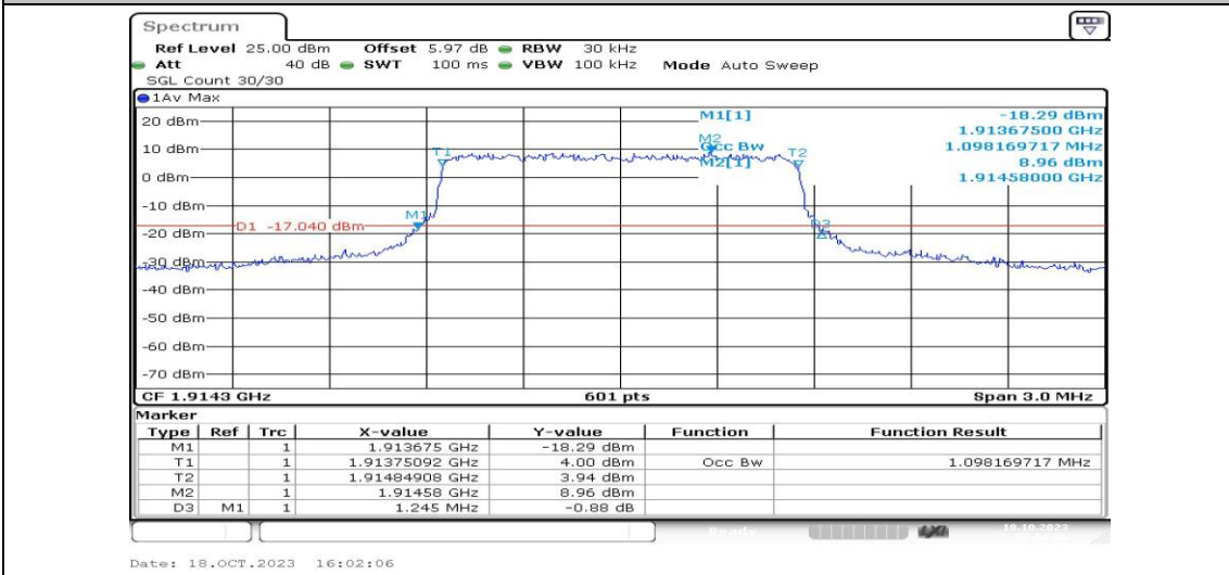
Band25-1.4MHz-QPSK-26683-6RB#0-PASS
