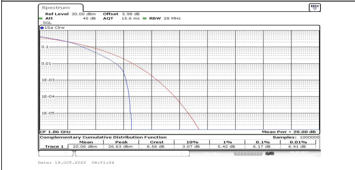
Band25-20MHz-16QAM-26140-25RB#0-PASS
