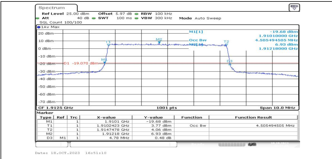
Band25-5MHz-16QAM-26665-25RB#0-PASS
