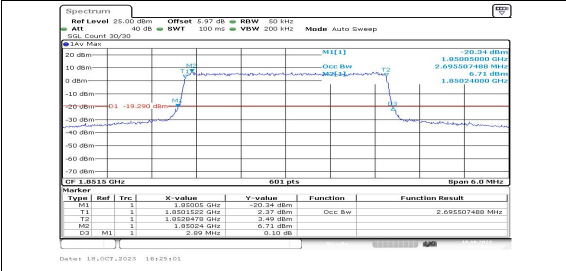
Band25-3MHz-QPSK-26055-15RB#0-PASS
