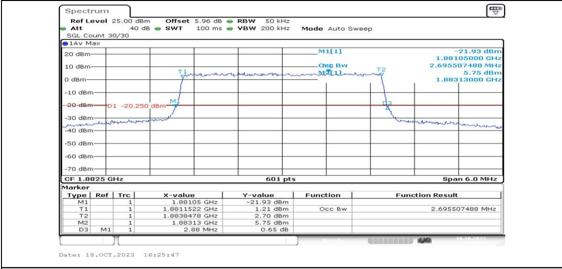
Band25-3MHz-16QAM-26365-15RB#0-PASS
