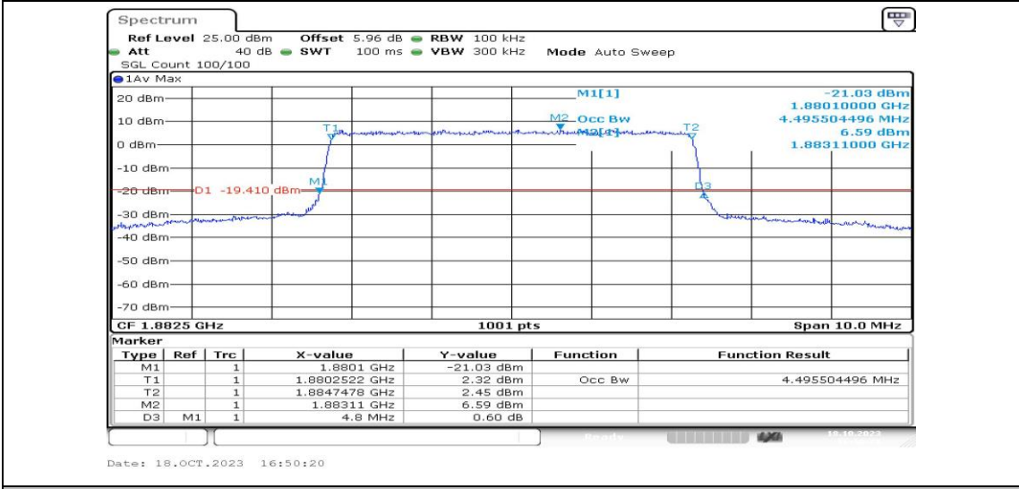
Band25-5MHz-16QAM-26365-25RB#0-PASS
