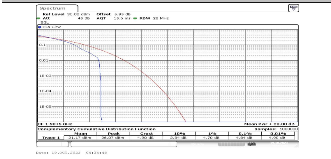
Band25-15MHz-QPSK-26615-1RB#0-PASS
