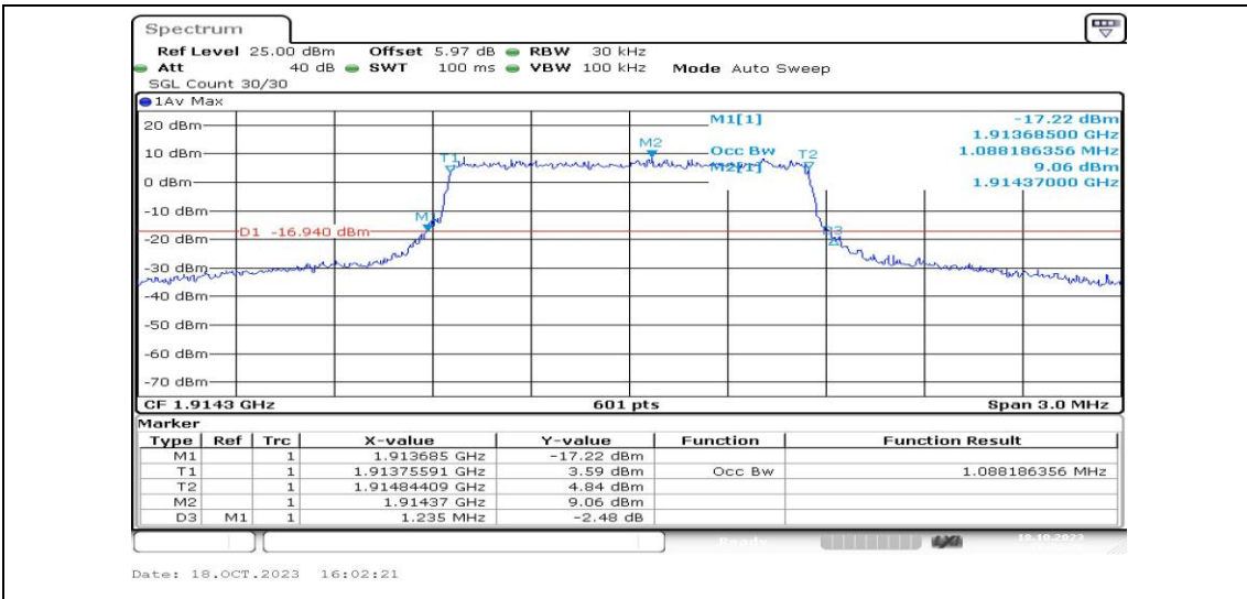
Band25-1.4MHz-16QAM-26683-6RB#0-PASS
