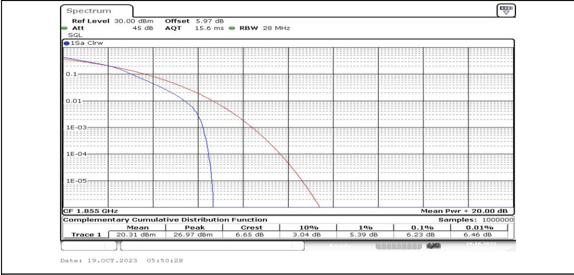
Band25-10MHz-16QAM-26090-25RB#0-PASS
