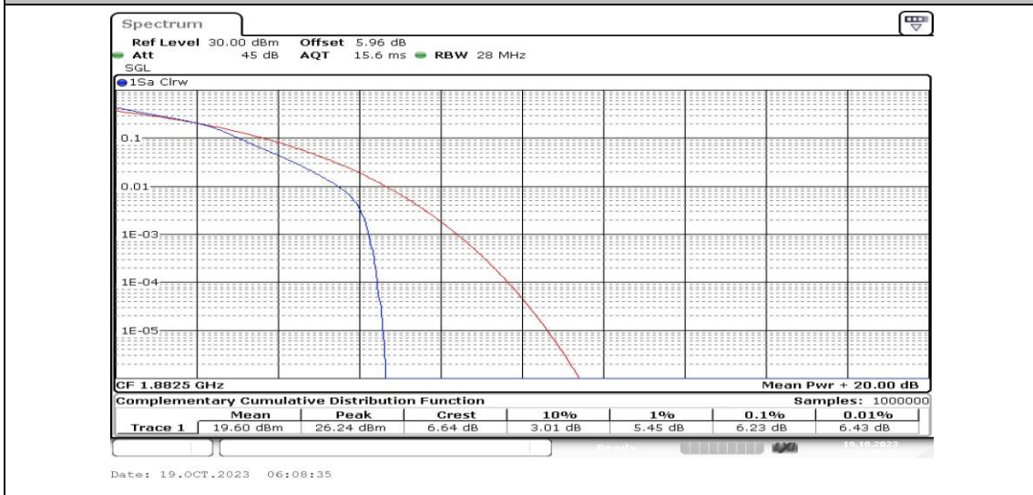
Band25-15MHz-16QAM-26365-25RB#0-PASS
