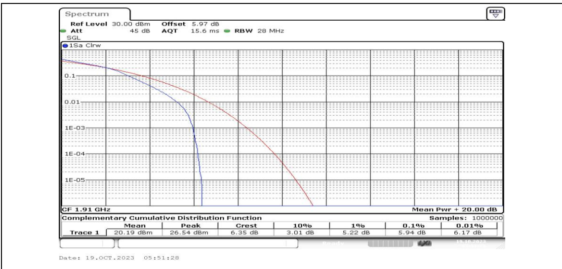
Band25-10MHz-16QAM-26640-25RB#0-PASS
