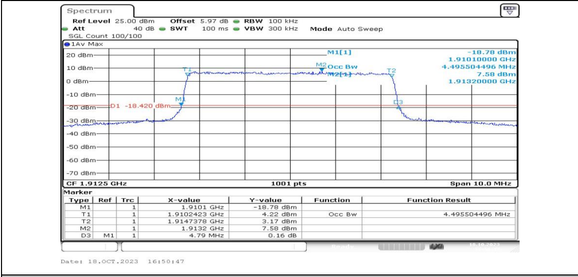
Band25-5MHz-QPSK-26665-25RB#0-PASS
