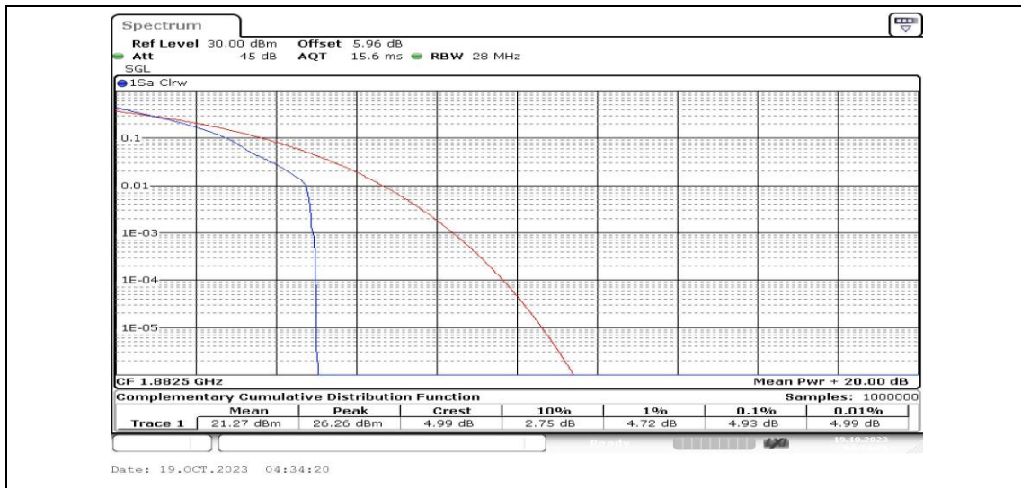
Band25-15MHz-QPSK-26365-1RB#0-PASS
