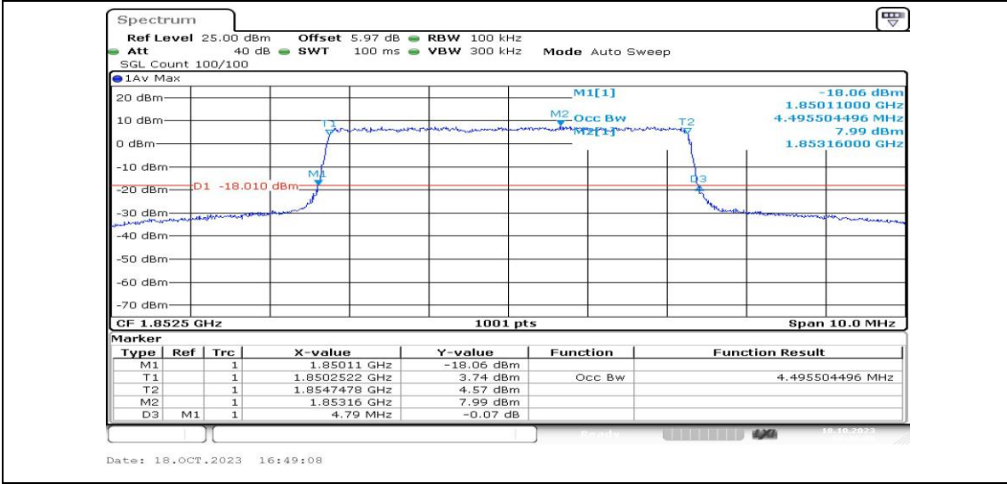
Band25-5MHz-QPSK-26065-25RB#0-PASS
