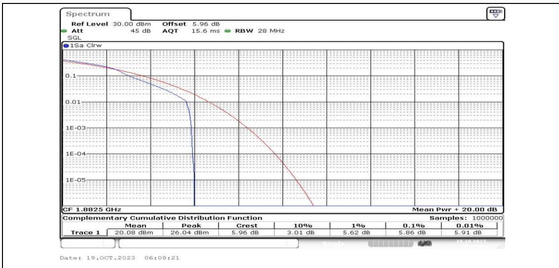
Band25-15MHz-16QAM-26365-1RB#0-PASS
