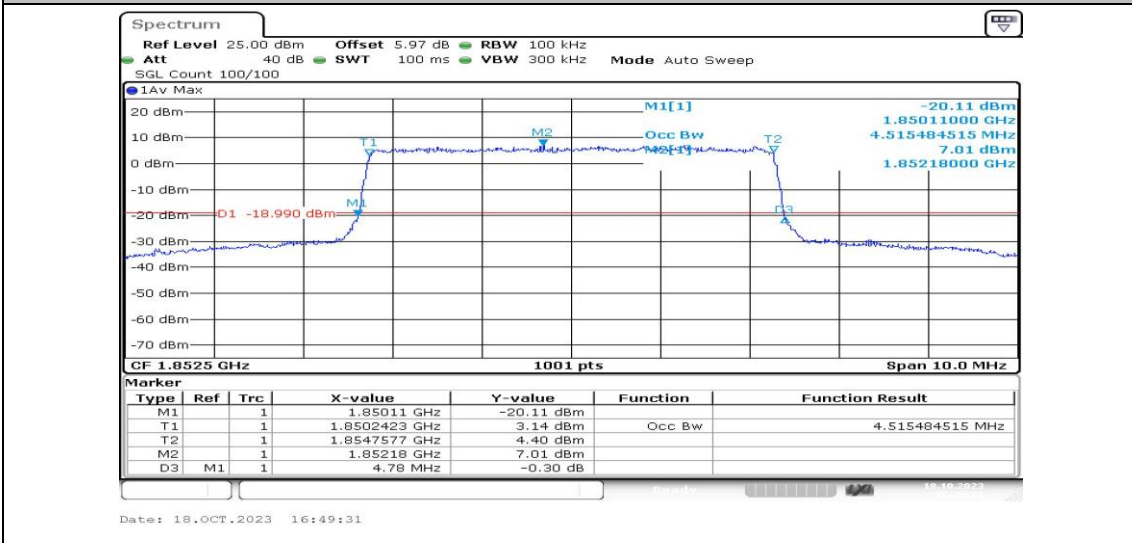
Band25-5MHz-16QAM-26065-25RB#0-PASS
