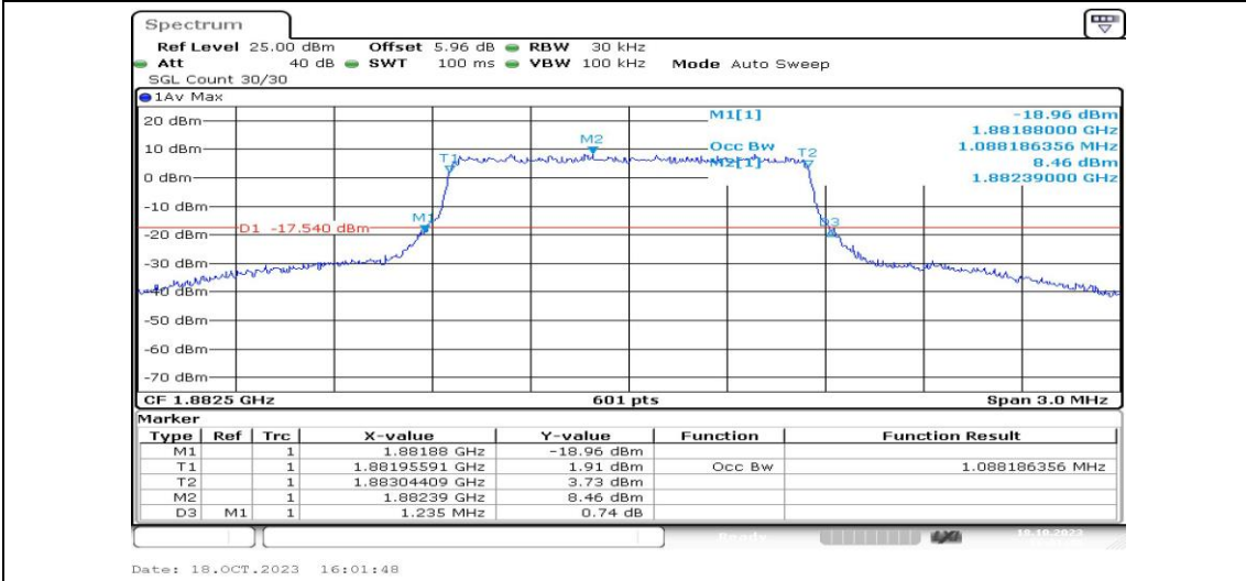
Band25-1.4MHz-16QAM-26365-6RB#0-PASS
