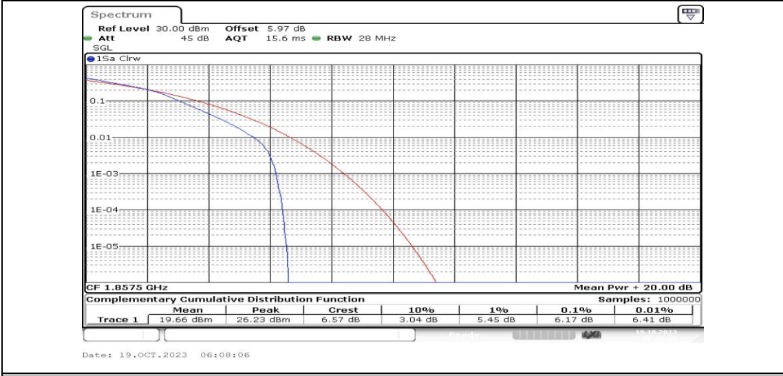
Band25-15MHz-16QAM-26115-25RB#0-PASS
