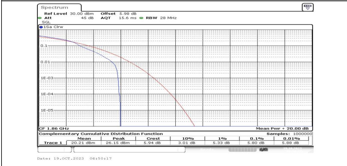
Band25-20MHz-16QAM-26140-1RB#0-PASS
