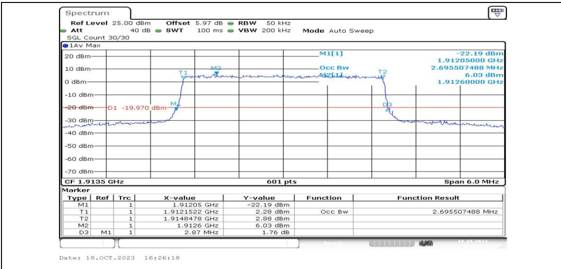
Band25-3MHz-16QAM-26675-15RB#0-PASS
