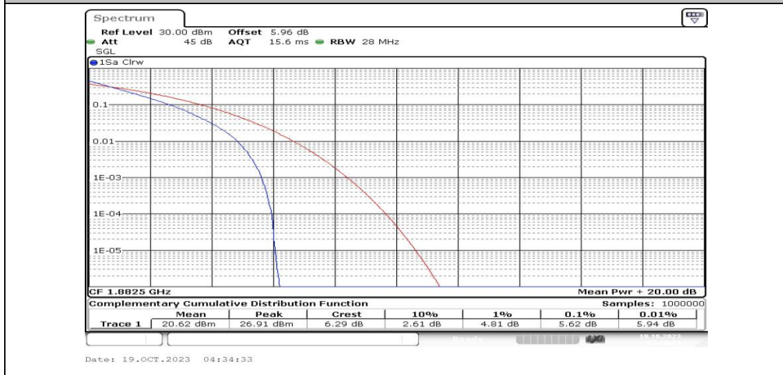
Band25-15MHz-QPSK-26365-75RB#0-PASS
