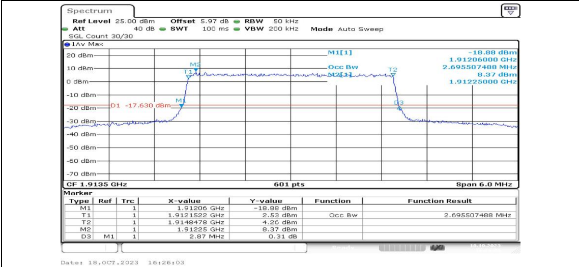
Band25-3MHz-QPSK-26675-15RB#0-PASS
