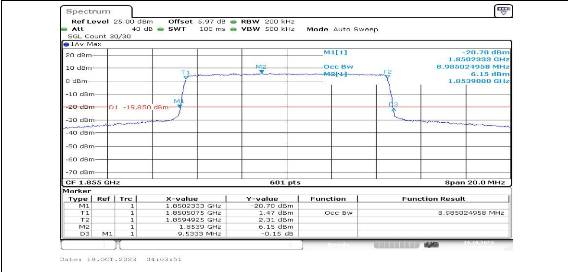
Band25-10MHz-QPSK-26090-50RB#0-PASS
