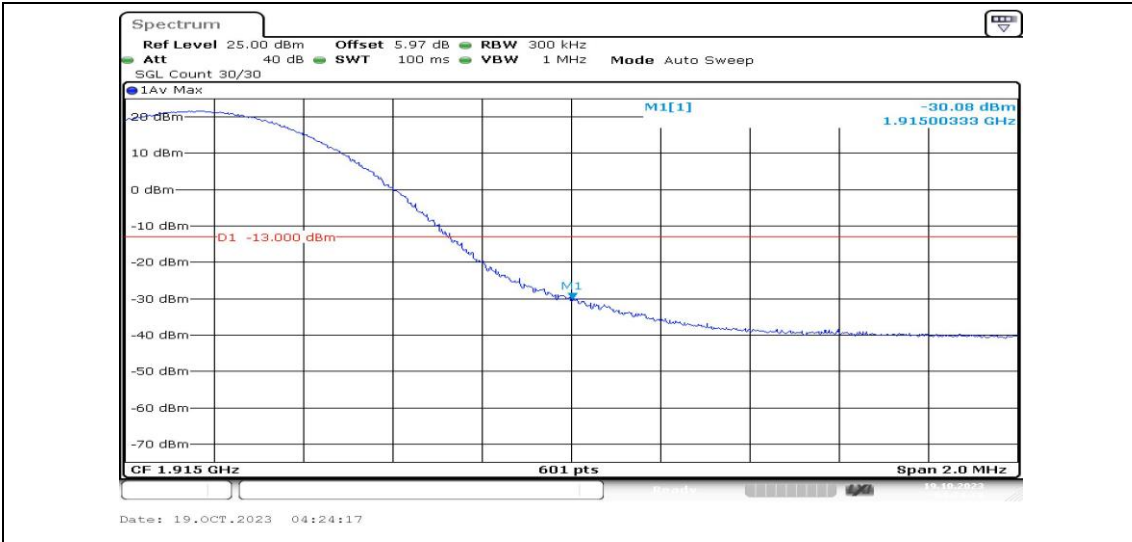
Band25-15MHz-QPSK-26615-1RB#74-PASS
