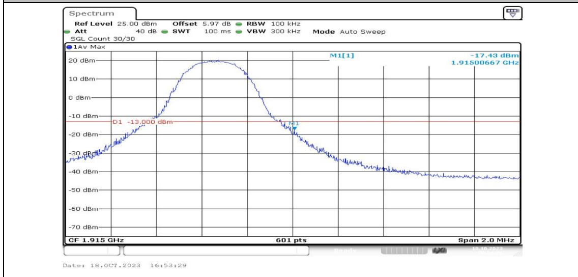
Band25-5MHz-QPSK-26665-1RB#24-PASS
