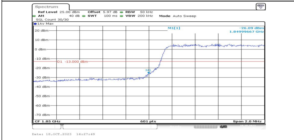
Band25-3MHz-16QAM-26055-15RB#0-PASS
