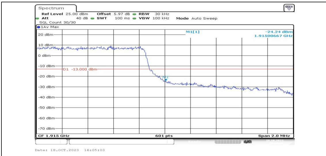
Band25-1.4MHz-QPSK-26683-6RB#0-PASS
