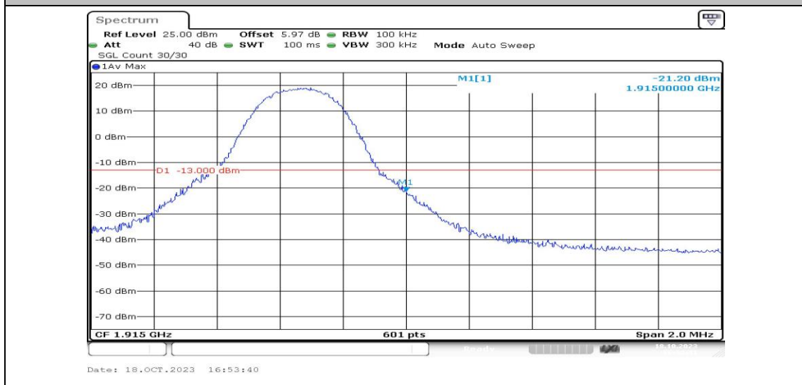
Band25-5MHz-16QAM-26665-1RB#24-PASS
