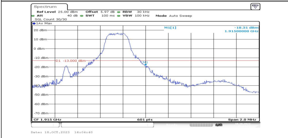
Band25-1.4MHz-QPSK-26683-1RB#5-PASS
