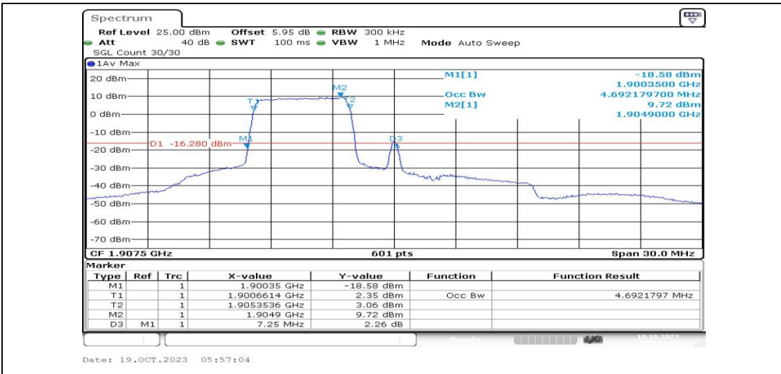
Band25-15MHz-16QAM-26615-25RB#0-PASS
