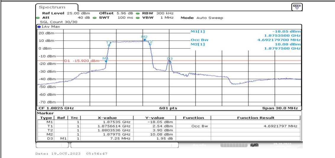
Band25-15MHz-16QAM-26365-25RB#0-PASS
