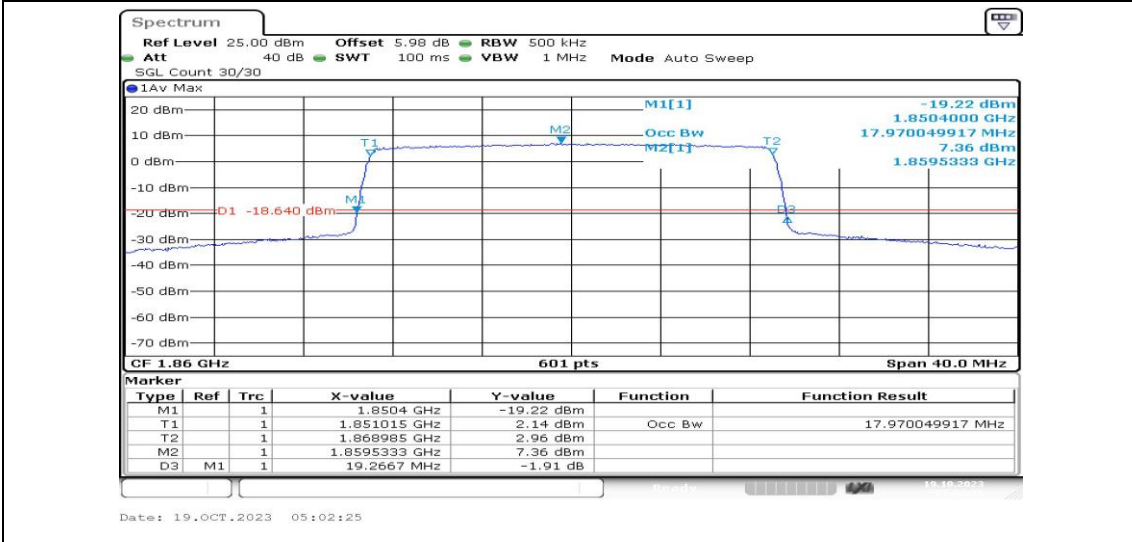
Band25-20MHz-QPSK-26140-100RB#0-PASS
