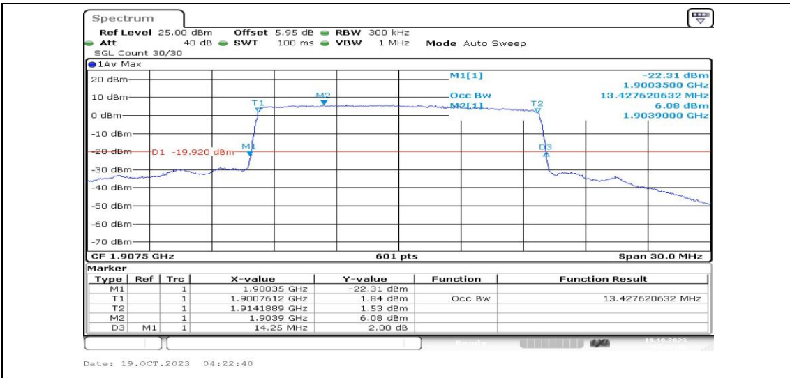
Band25-15MHz-QPSK-26615-75RB#0-PASS
