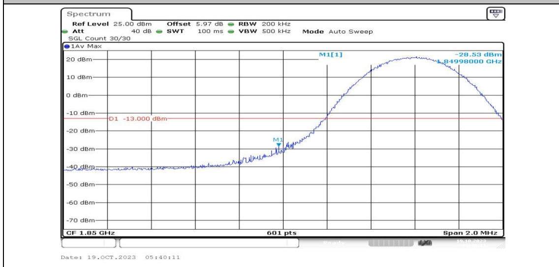
Band25-10MHz-16QAM-26090-1RB#0-PASS
