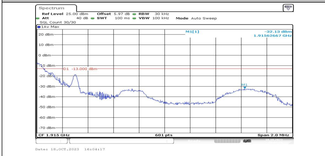
Band25-1.4MHz-QPSK-26683-1RB#0-PASS
