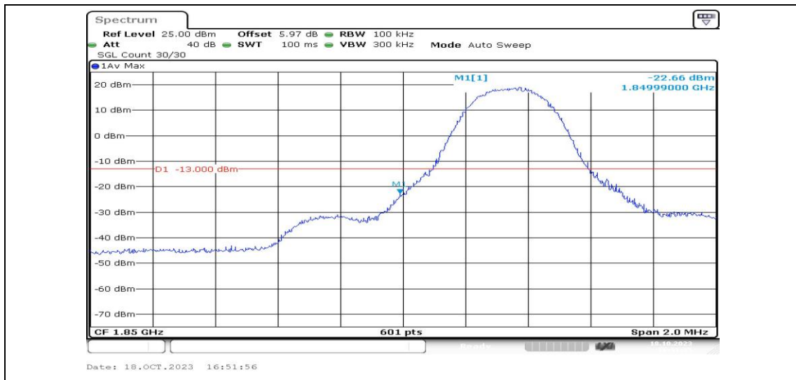
Band25-5MHz-16QAM-26065-1RB#0-PASS
