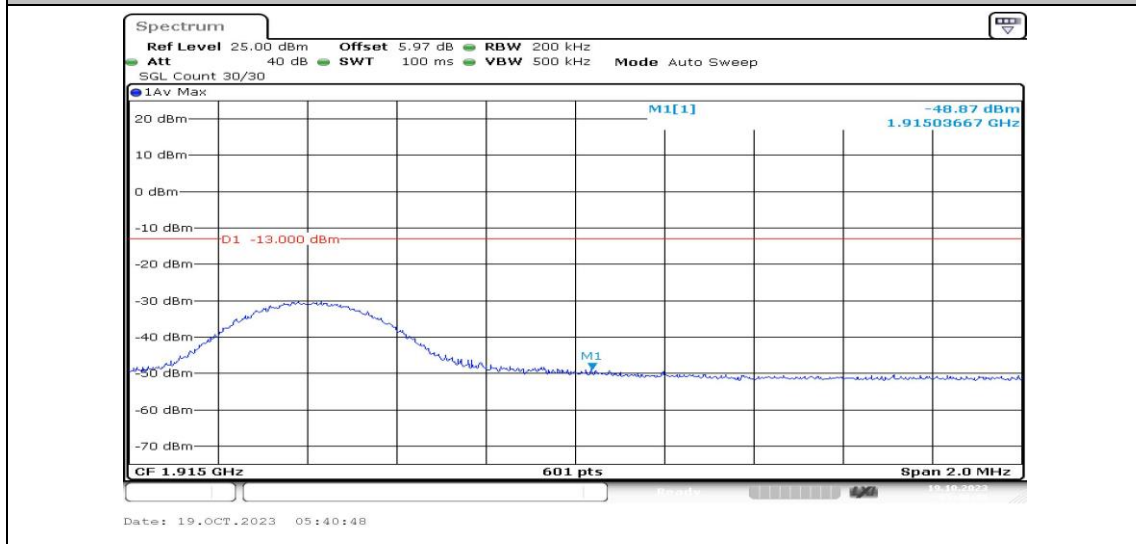
Band25-10MHz-16QAM-26640-1RB#0-PASS
