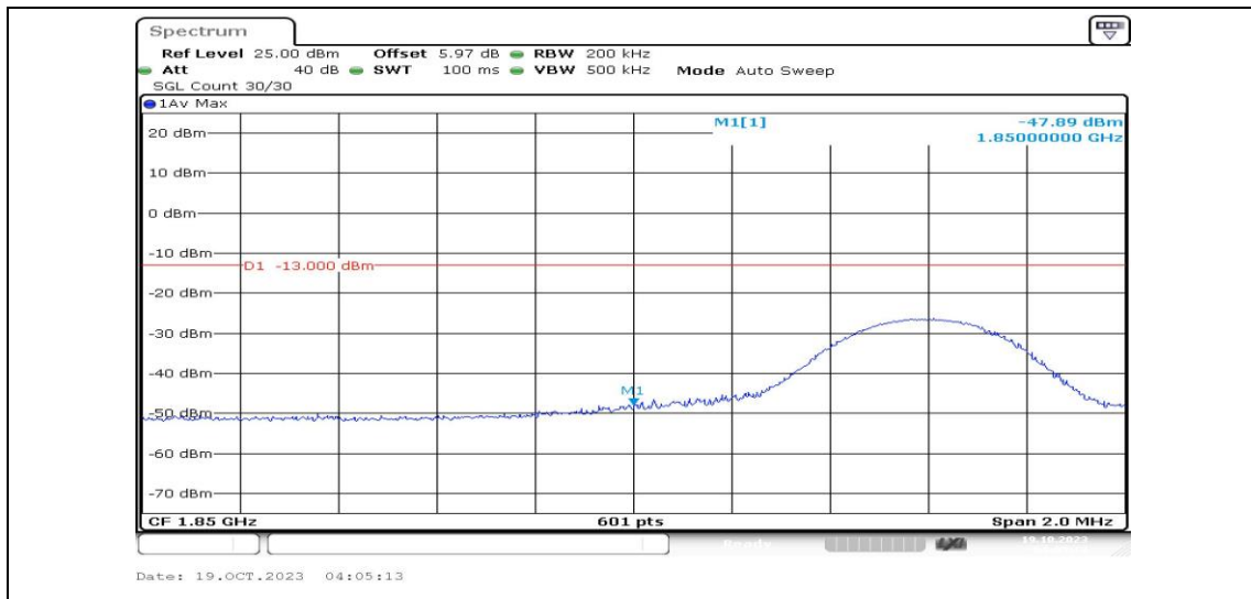
Band25-10MHz-QPSK-26090-1RB#49-PASS
