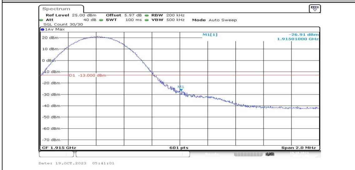
Band25-10MHz-16QAM-26640-1RB#49-PASS
