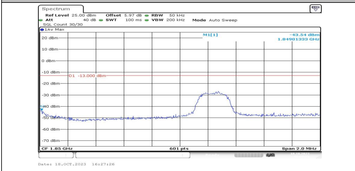
Band25-3MHz-16QAM-26055-1RB#14-PASS
