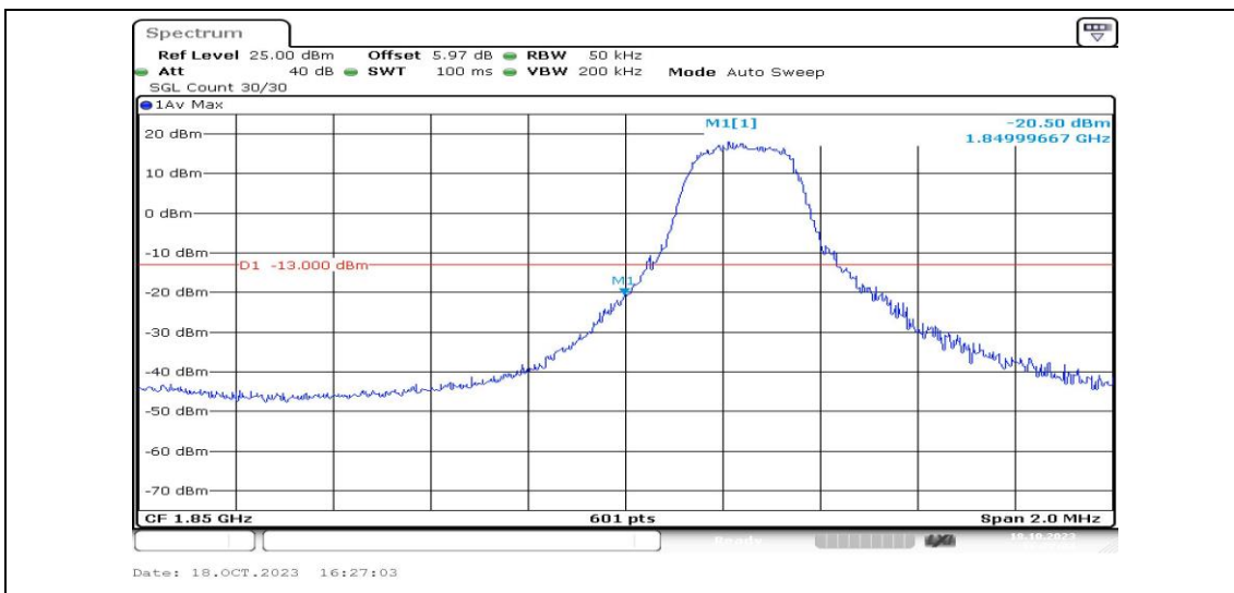
Band25-3MHz-16QAM-26055-1RB#0-PASS
