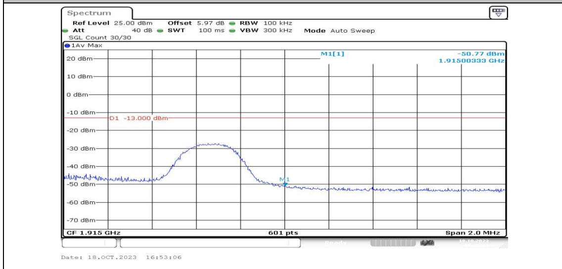
Band25-5MHz-QPSK-26665-1RB#0-PASS
