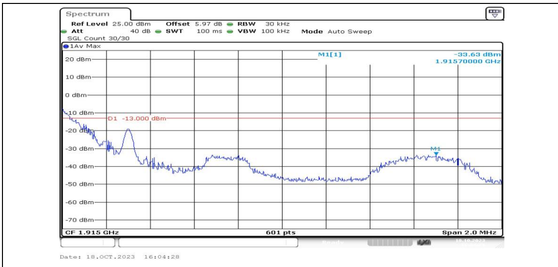
Band25-1.4MHz-16QAM-26683-1RB#0-PASS
