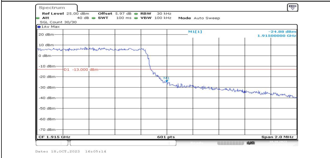
Band25-1.4MHz-16QAM-26683-6RB#0-PASS
