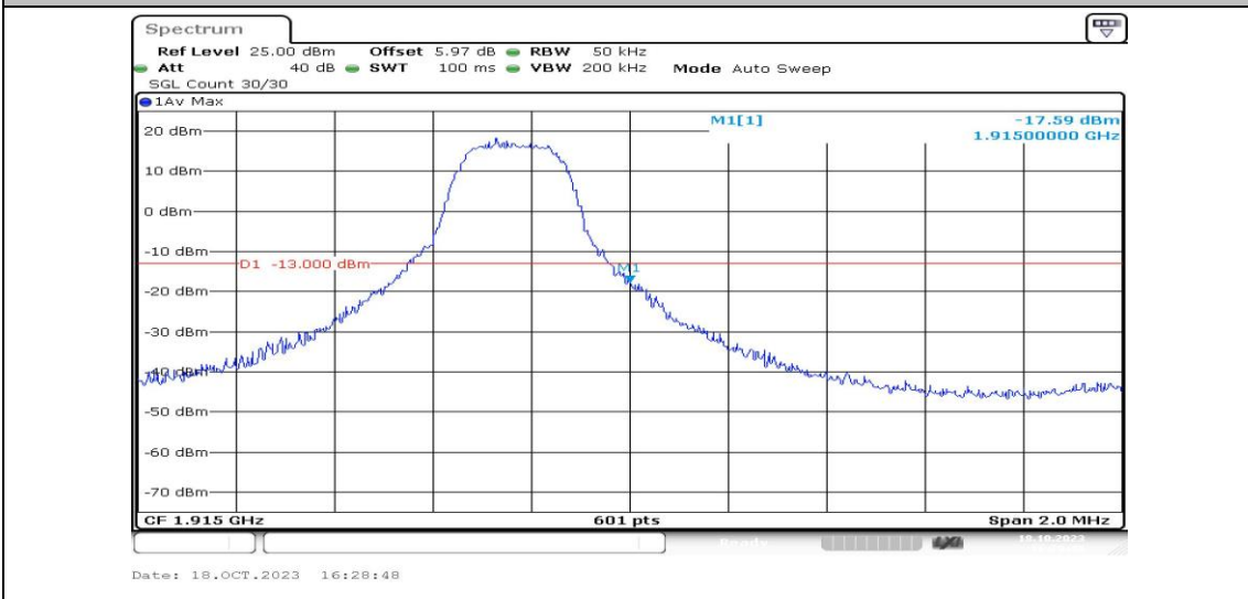
Band25-3MHz-16QAM-26675-1RB#14-PASS
