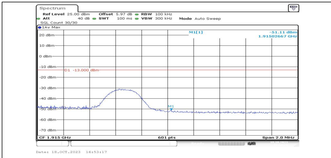
Band25-5MHz-16QAM-26665-1RB#0-PASS
