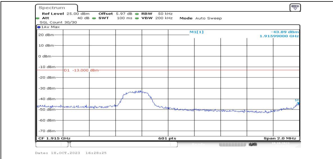
Band25-3MHz-16QAM-26675-1RB#0-PASS
