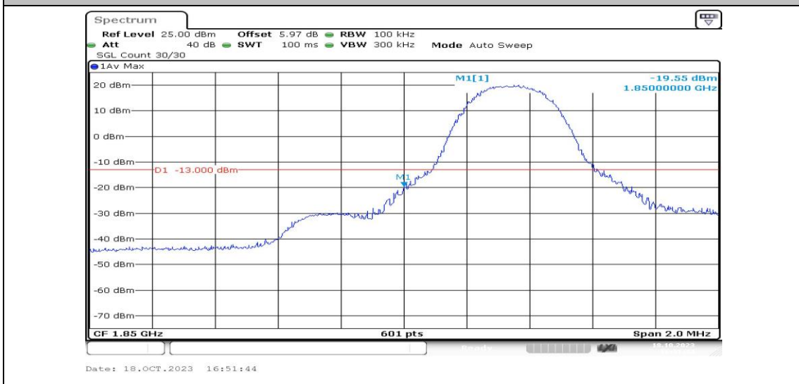
Band25-5MHz-QPSK-26065-1RB#0-PASS
