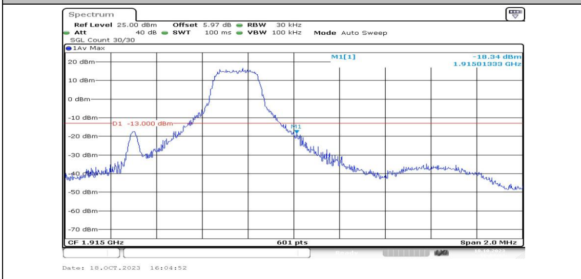
Band25-1.4MHz-16QAM-26683-1RB#5-PASS
