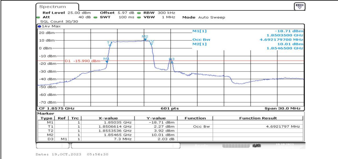
Band25-15MHz-16QAM-26115-25RB#0-PASS
