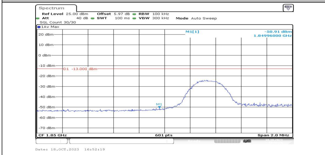
Band25-5MHz-16QAM-26065-1RB#24-PASS
