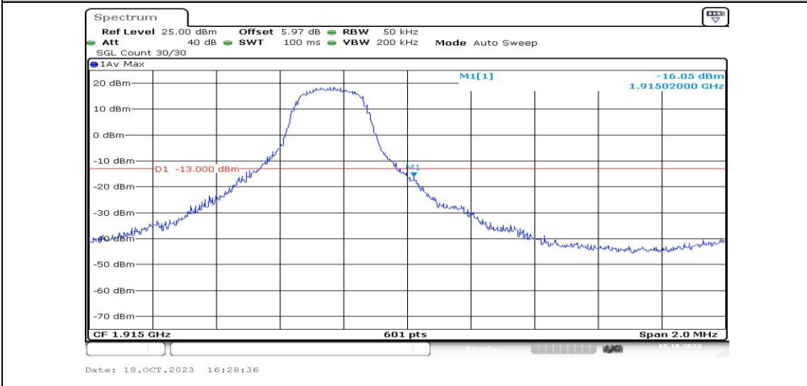
Band25-3MHz-QPSK-26675-1RB#14-PASS
