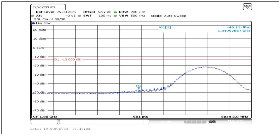
Band25-10MHz-16QAM-26090-1RB#49-PASS
