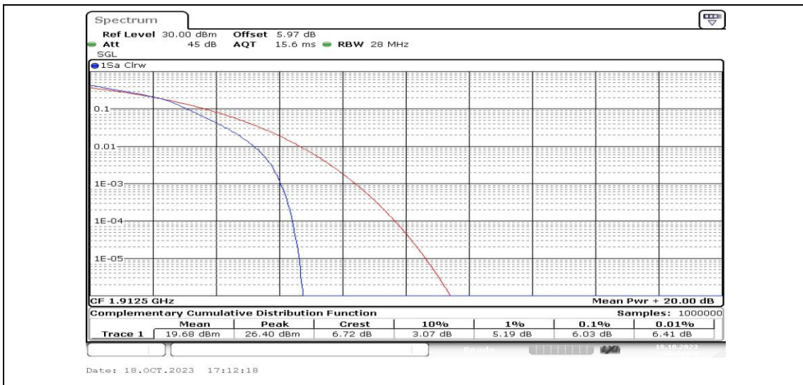
Band25-5MHz-16QAM-26665-25RB#0-PASS
