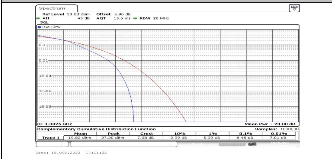
Band25-5MHz-16QAM-26365-25RB#0-PASS
