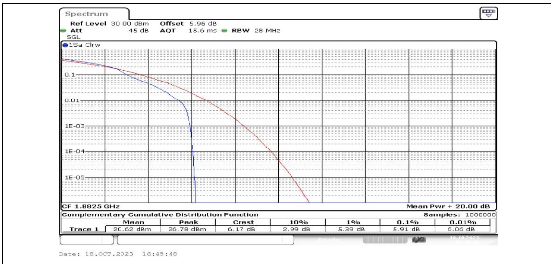
Band25-3MHz-16QAM-26365-1RB#0-PASS
