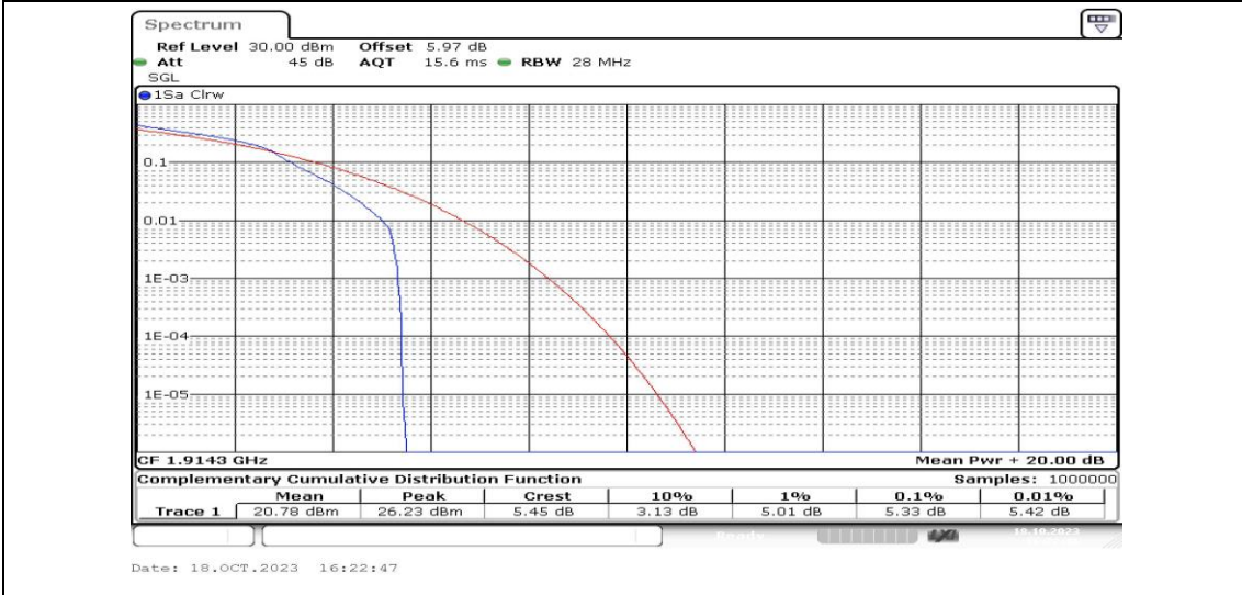
Band25-1.4MHz-16QAM-26683-1RB#0-PASS
