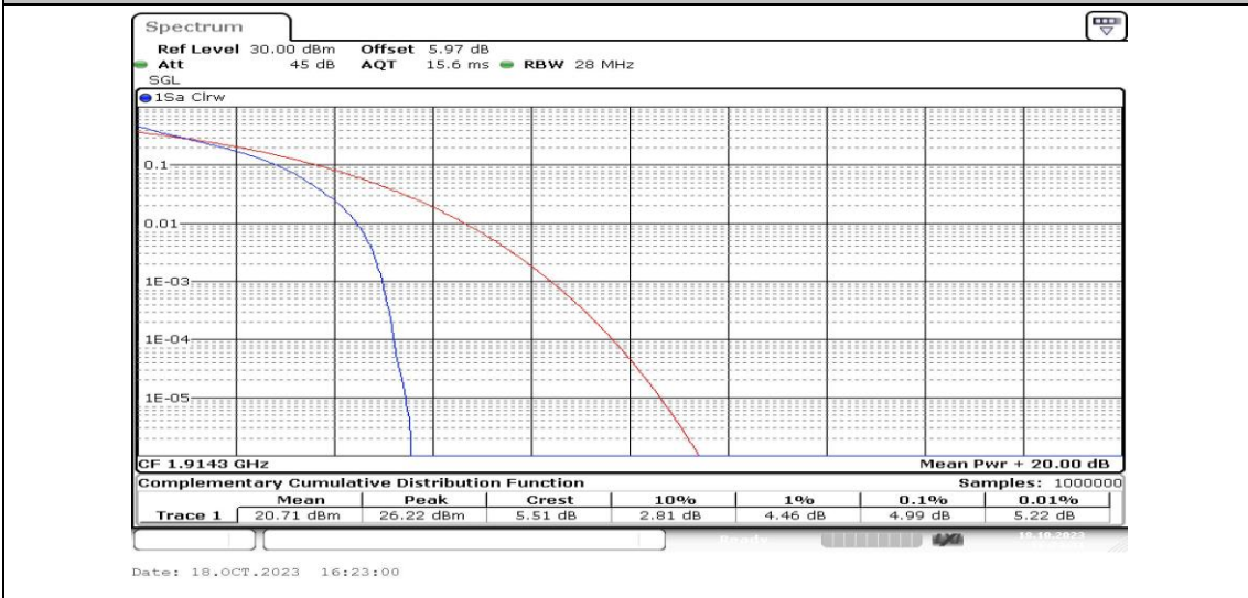
Band25-1.4MHz-QPSK-26683-6RB#0-PASS
