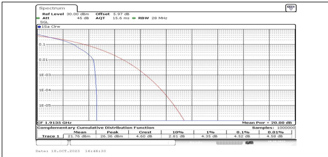
Band25-3MHz-QPSK-26675-1RB#0-PASS
