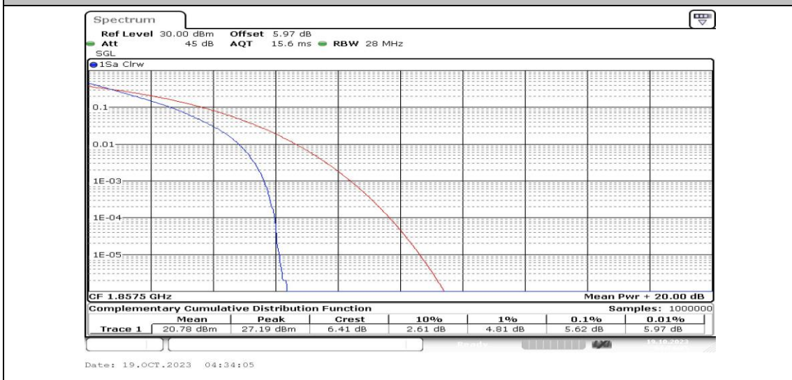
Band25-15MHz-QPSK-26115-75RB#0-PASS
