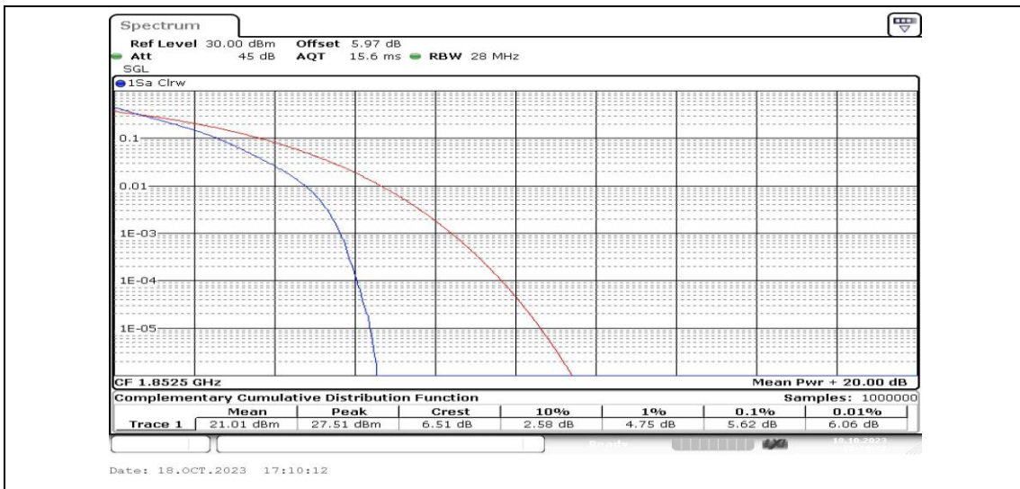
Band25-5MHz-QPSK-26065-25RB#0-PASS
