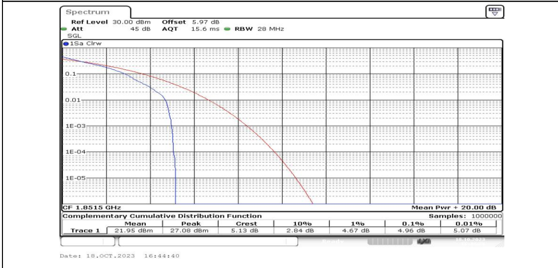
Band25-3MHz-QPSK-26055-1RB#0-PASS
