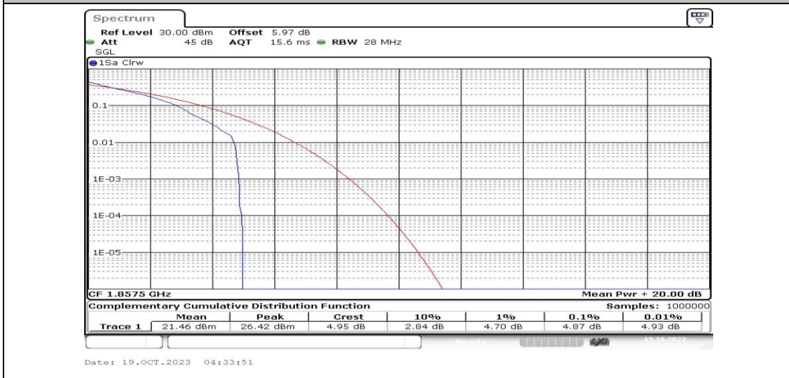
Band25-15MHz-QPSK-26115-1RB#0-PASS
