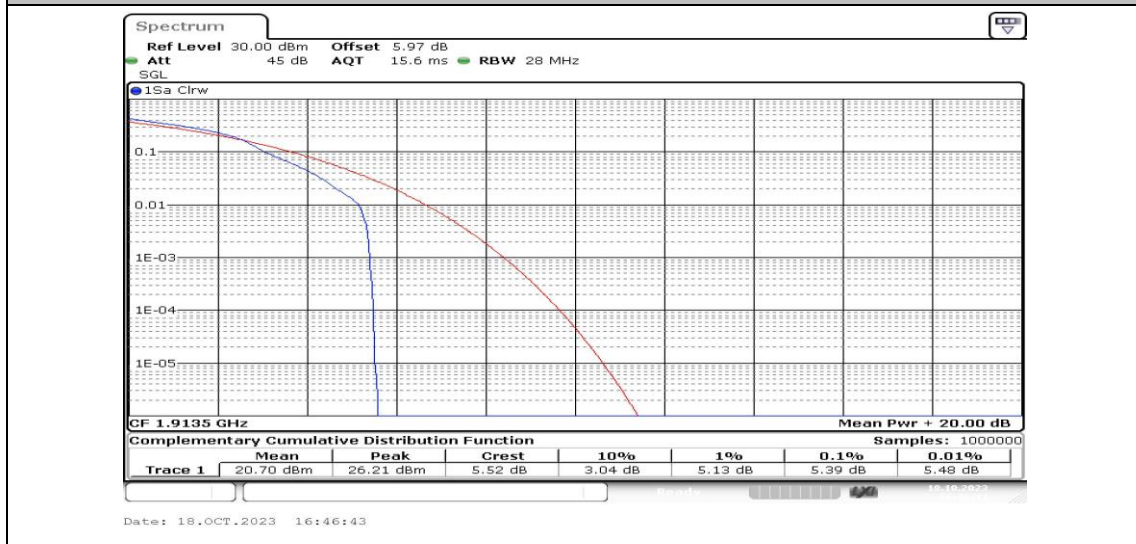
Band25-3MHz-16QAM-26675-1RB#0-PASS
