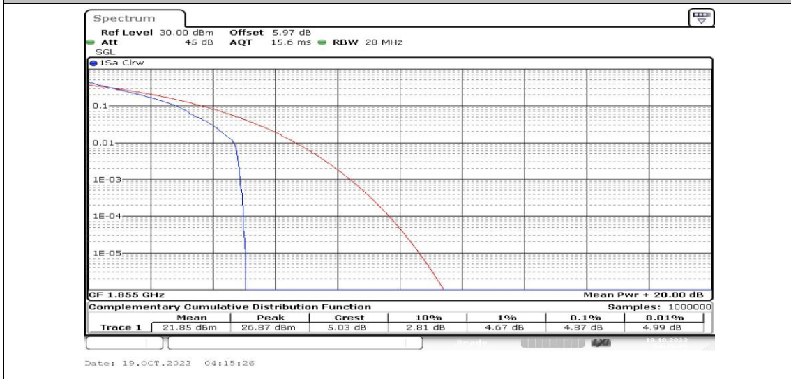
Band25-10MHz-QPSK-26090-1RB#0-PASS
