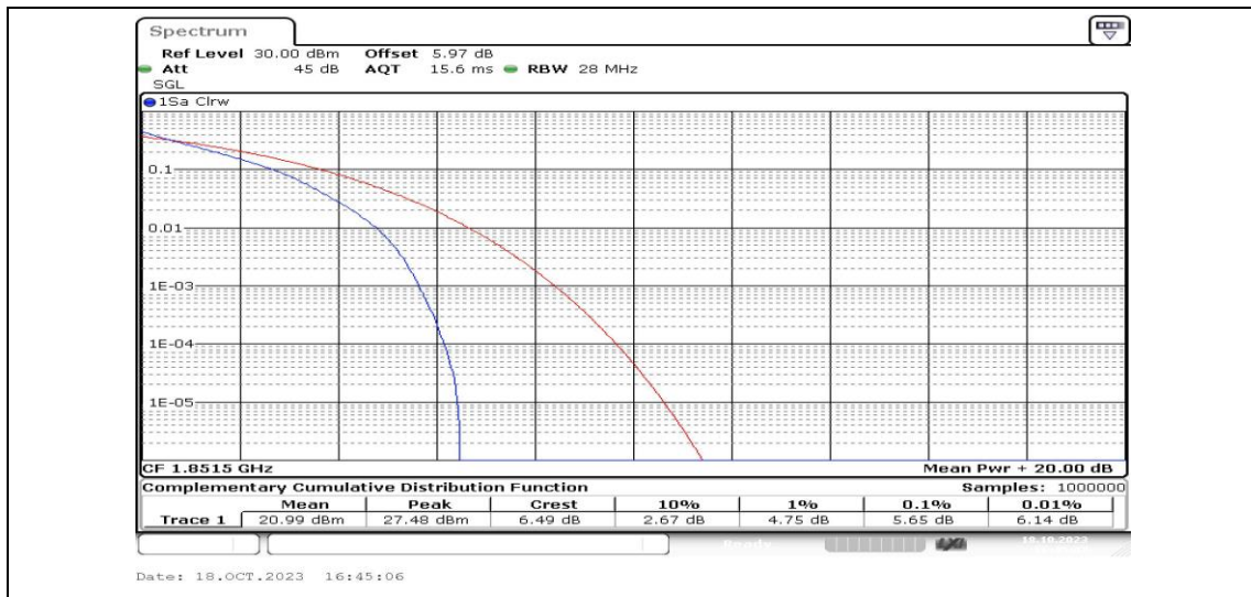
Band25-3MHz-QPSK-26055-15RB#0-PASS
