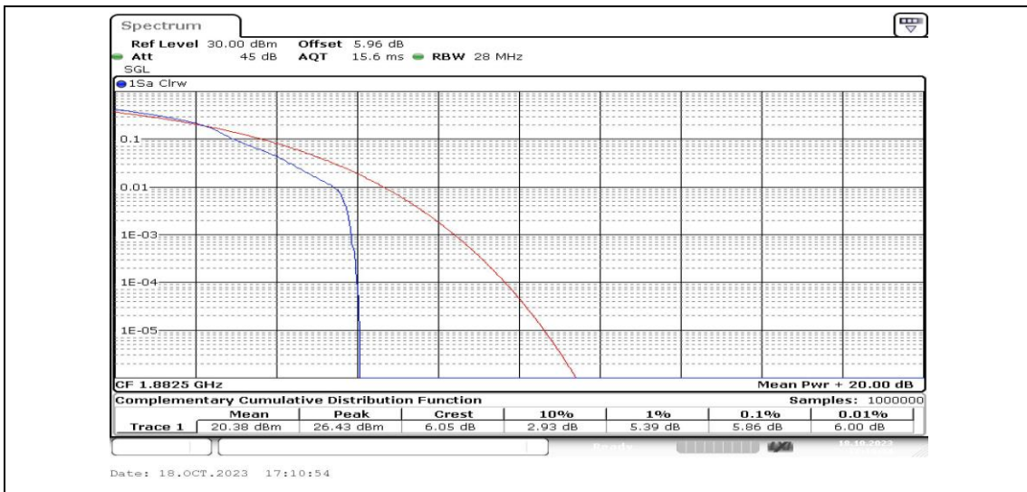
Band25-5MHz-16QAM-26365-1RB#0-PASS
