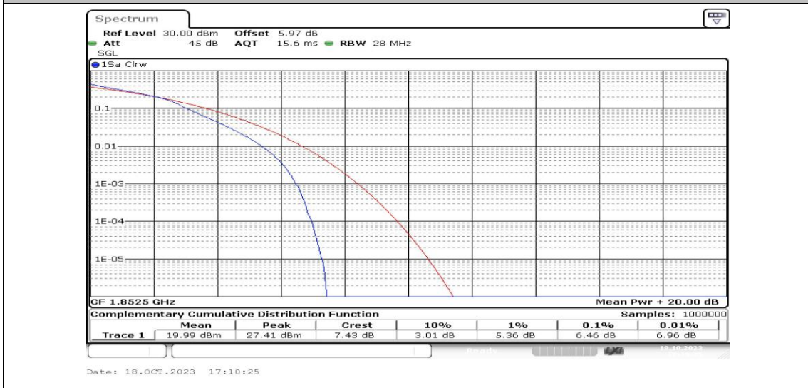
Band25-5MHz-16QAM-26065-25RB#0-PASS
