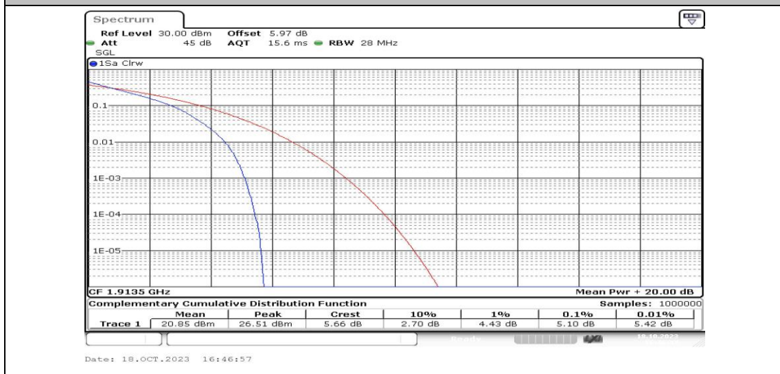
Band25-3MHz-QPSK-26675-15RB#0-PASS
