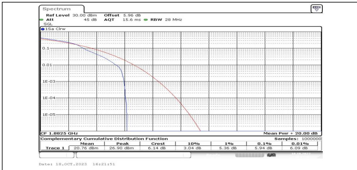
Band25-1.4MHz-16QAM-26365-1RB#0-PASS
