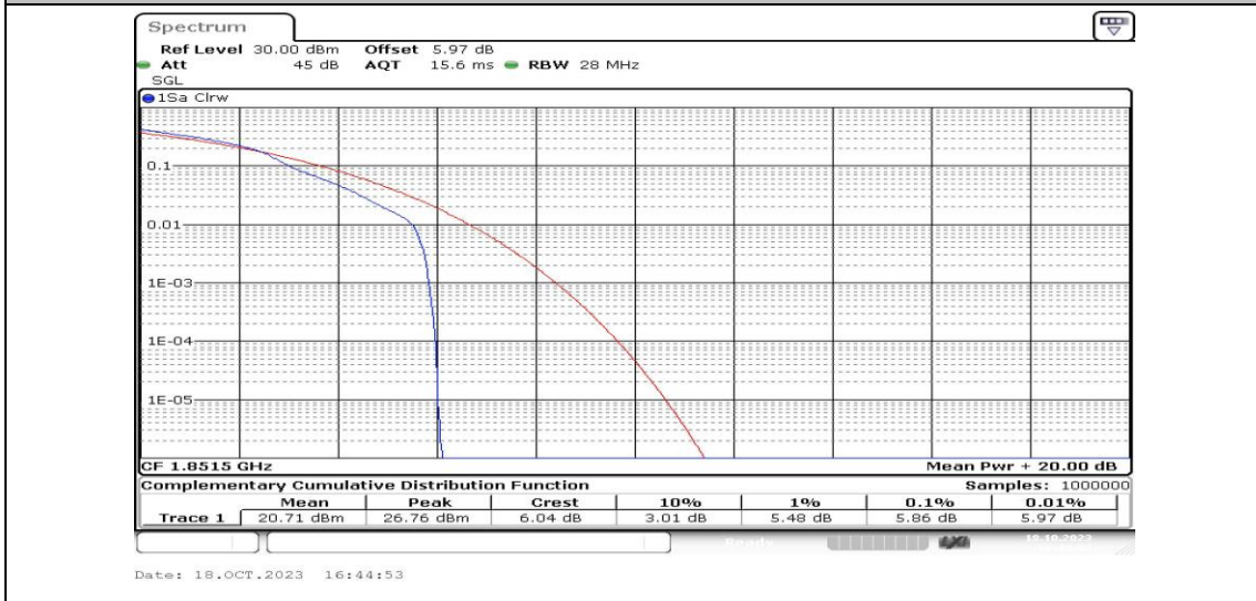
Band25-3MHz-16QAM-26055-1RB#0-PASS
