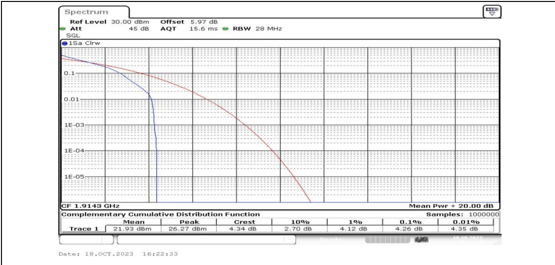
Band25-1.4MHz-QPSK-26683-1RB#0-PASS
