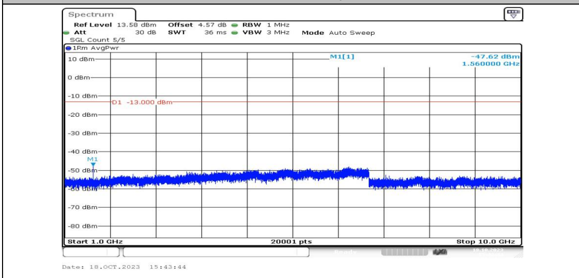
Band13-5MHz-QPSK-23230-1RB#0-Range4:1000~10000MHz-PASS
