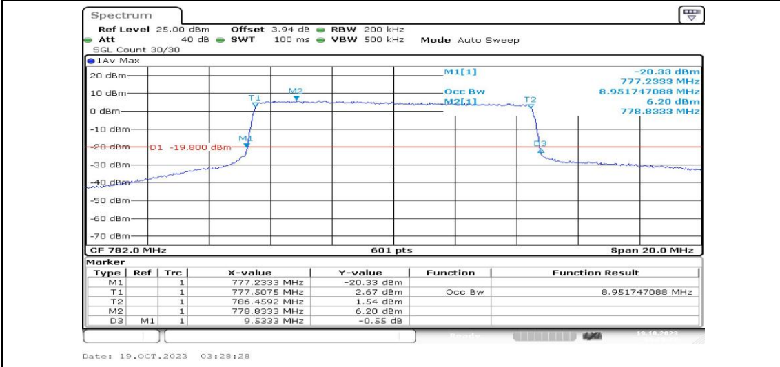
Band13-10MHz-QPSK-23230-50RB#0-PASS
