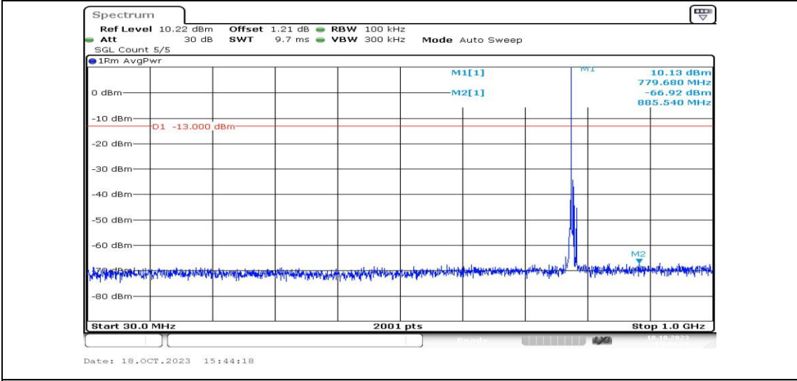
Band13-5MHz-16QAM-23230-1RB#0-Range3:30~1000MHz-PASS
