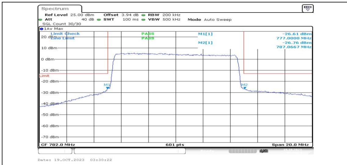
Band13-10MHz-QPSK-23230-50RB#0-PASS
