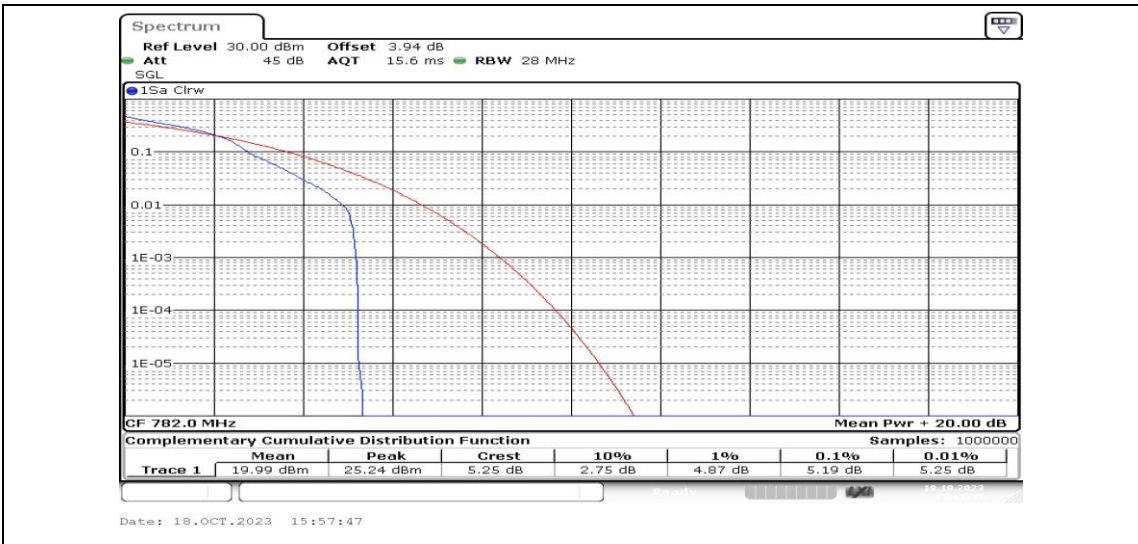
Band13-5MHz-16QAM-23230-1RB#0-PASS
