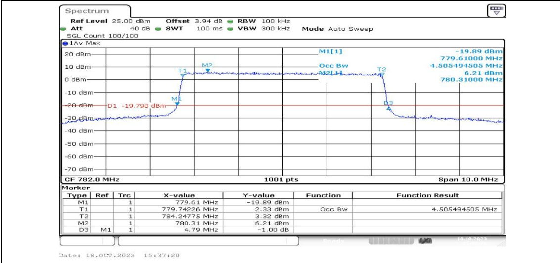
Band13-5MHz-16QAM-23230-25RB#0-PASS
