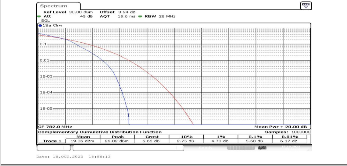
Band13-5MHz-16QAM-23230-25RB#0-PASS
