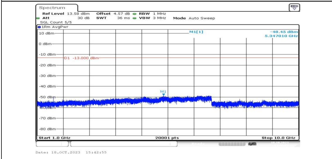
Band13-5MHz-16QAM-23205-1RB#0-Range4:1000~10000MHz-PASS
