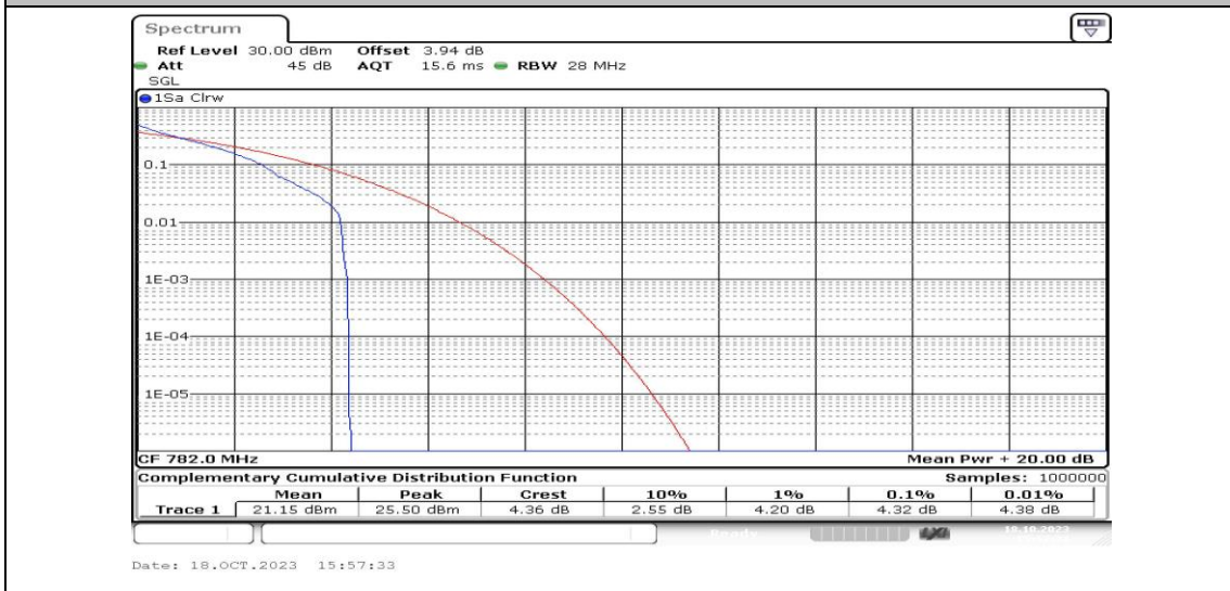
Band13-5MHz-QPSK-23230-1RB#0-PASS
