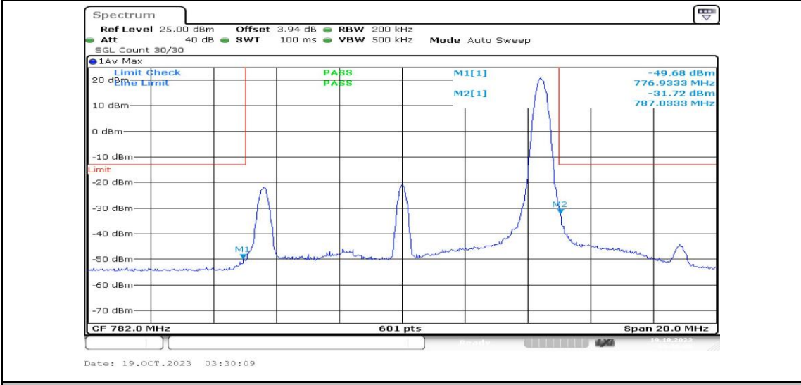
Band13-10MHz-QPSK-23230-1RB#49-PASS
