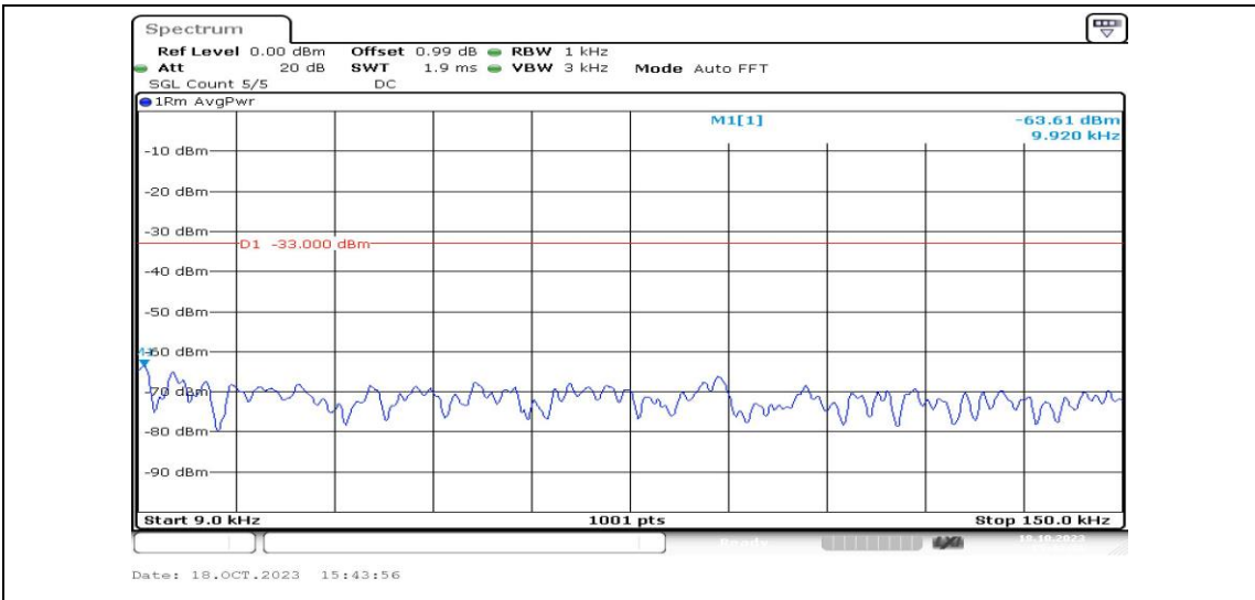
Band13-5MHz-16QAM-23230-1RB#0-Range1:0.009~0.15MHz-PASS
