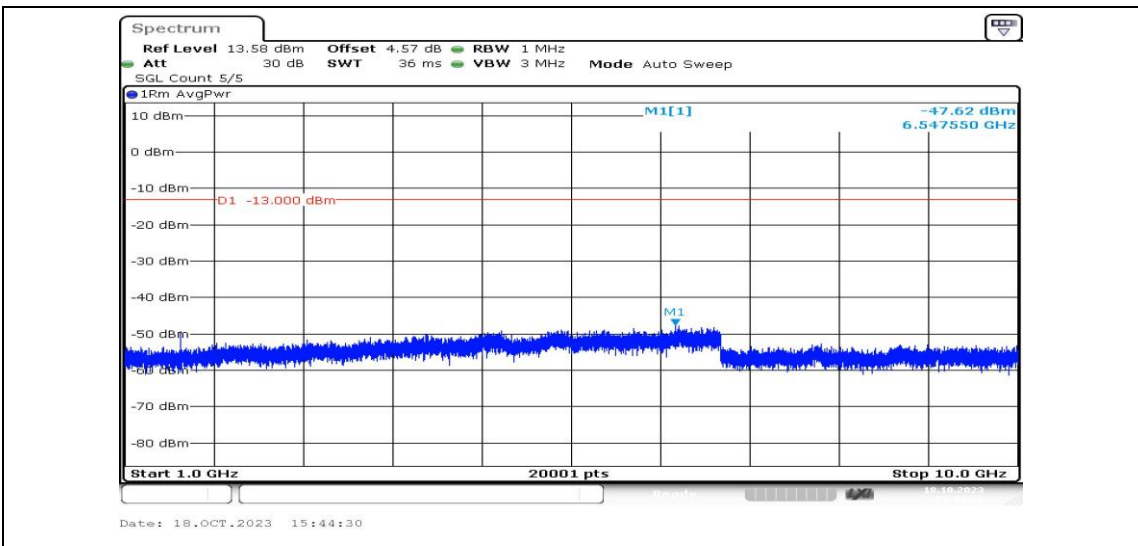
Band13-5MHz-16QAM-23230-1RB#0-Range4:1000~10000MHz-PASS
