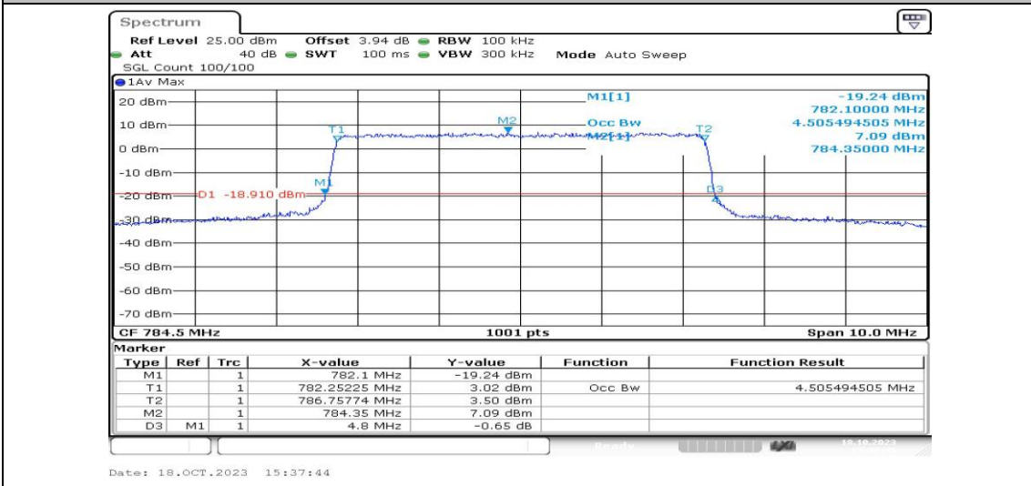
Band13-5MHz-QPSK-23255-25RB#0-PASS
