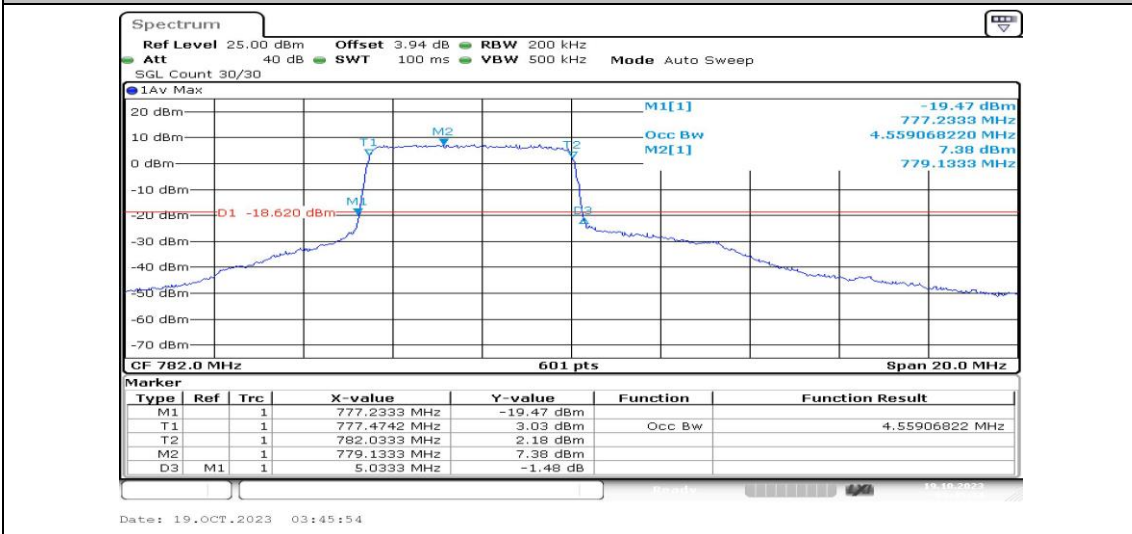
Band13-10MHz-16QAM-23230-25RB#0-PASS
