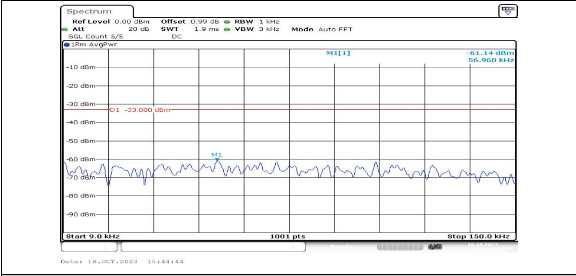
Band13-5MHz-QPSK-23255-1RB#0-Range1:0.009~0.15MHz-PASS
