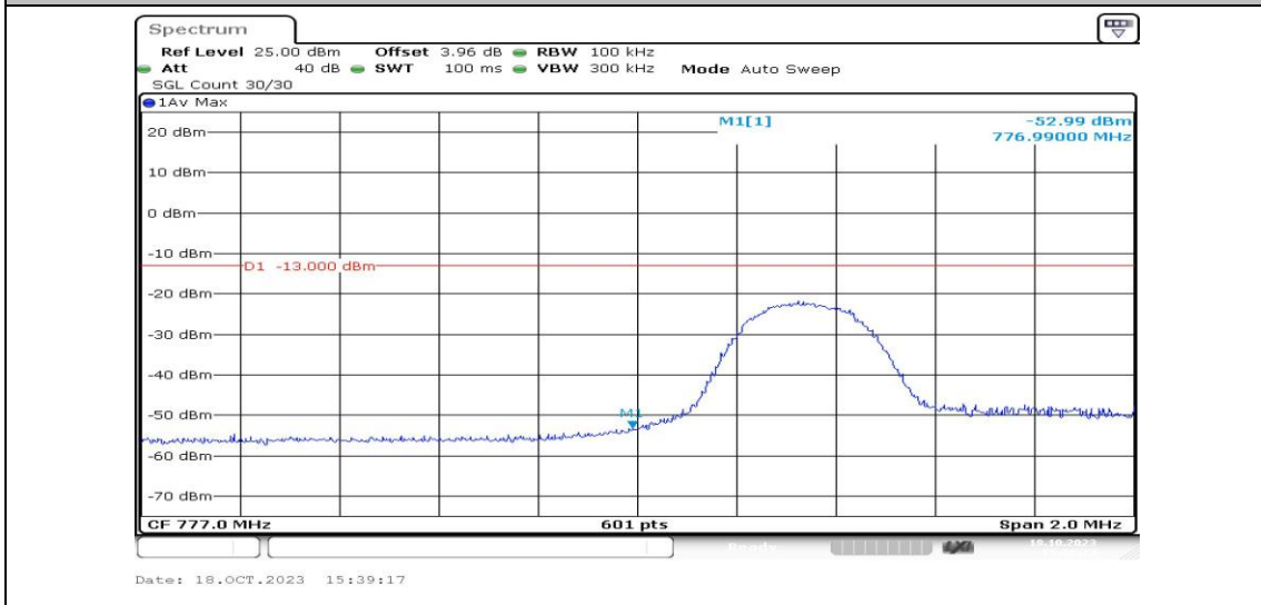
Band13-5MHz-16QAM-23205-1RB#24-PASS
