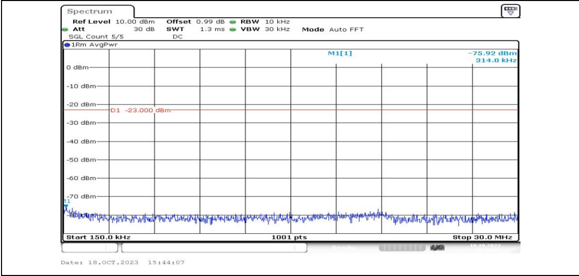
Band13-5MHz-16QAM-23230-1RB#0-Range2:0.15~30MHz-PASS
