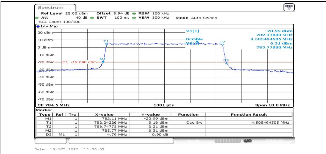
Band13-5MHz-16QAM-23255-25RB#0-PASS
