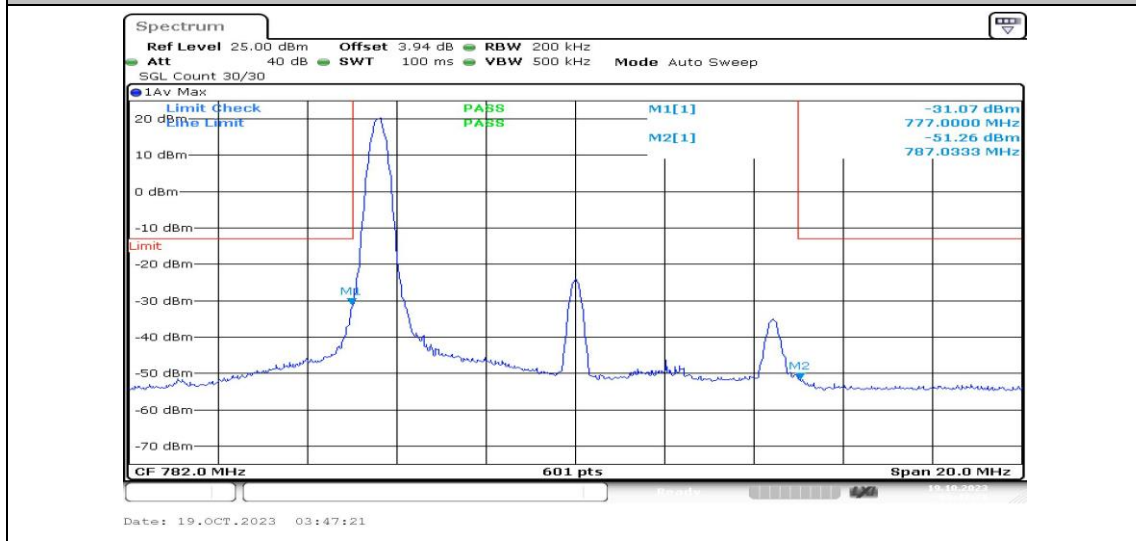
Band13-10MHz-16QAM-23230-1RB#0-PASS
