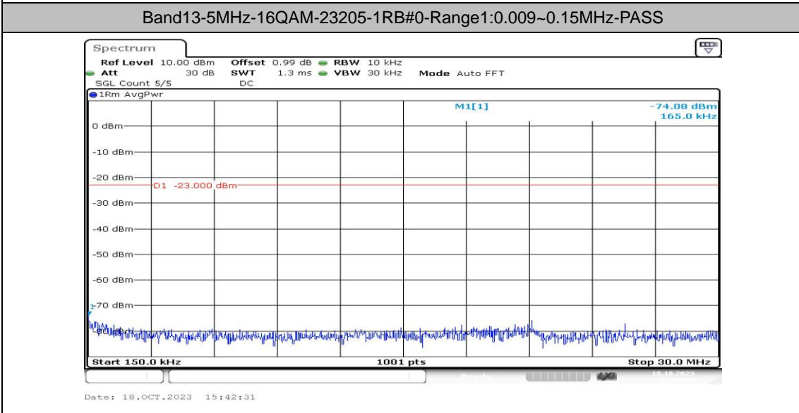
Band13-5MHz-16QAM-23205-1RB#0-Range2:0.15~30MHz-PASS
