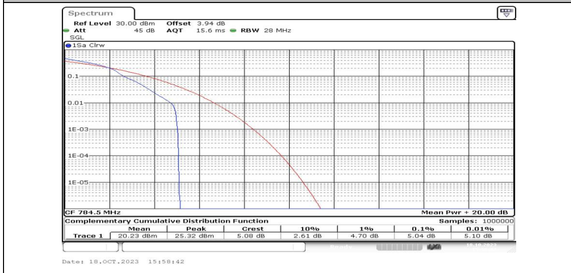
Band13-5MHz-16QAM-23255-1RB#0-PASS
