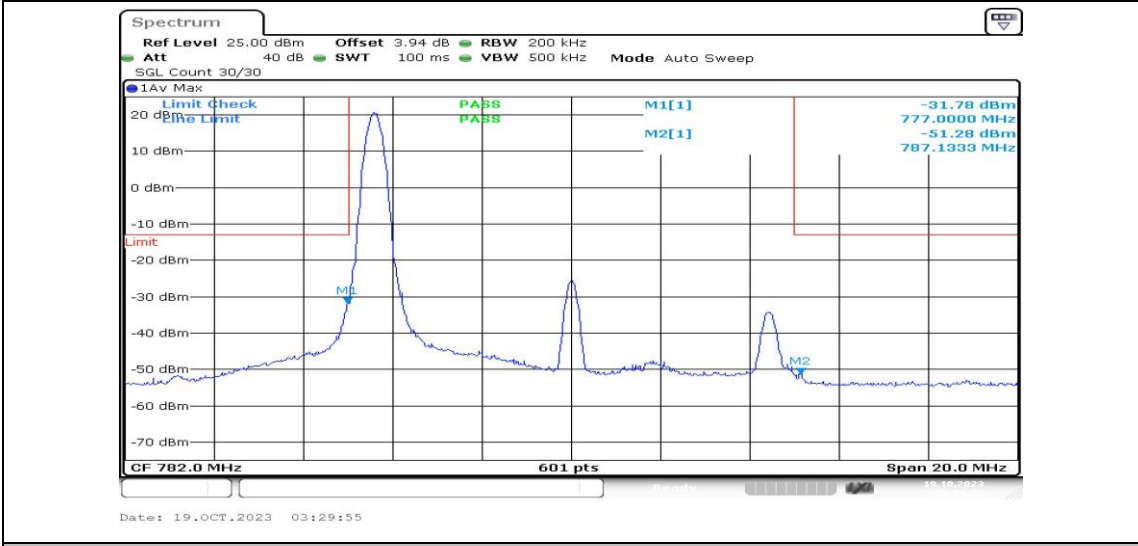
Band13-10MHz-QPSK-23230-1RB#0-PASS
