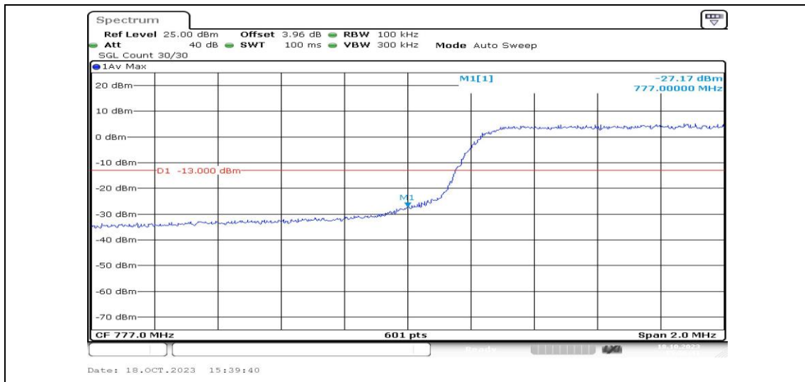
Band13-5MHz-16QAM-23205-25RB#0-PASS
