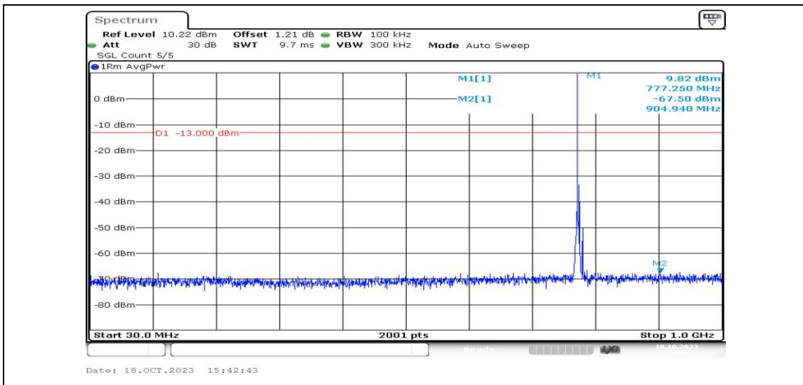
Band13-5MHz-16QAM-23205-1RB#0-Range3:30~1000MHz-PASS
