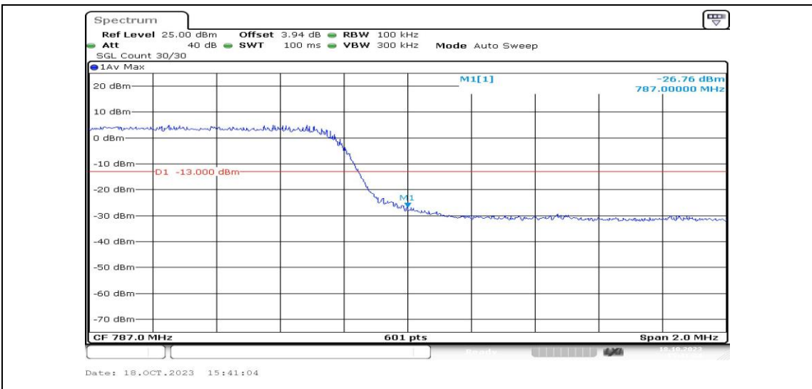
Band13-5MHz-16QAM-23255-25RB#0-PASS
