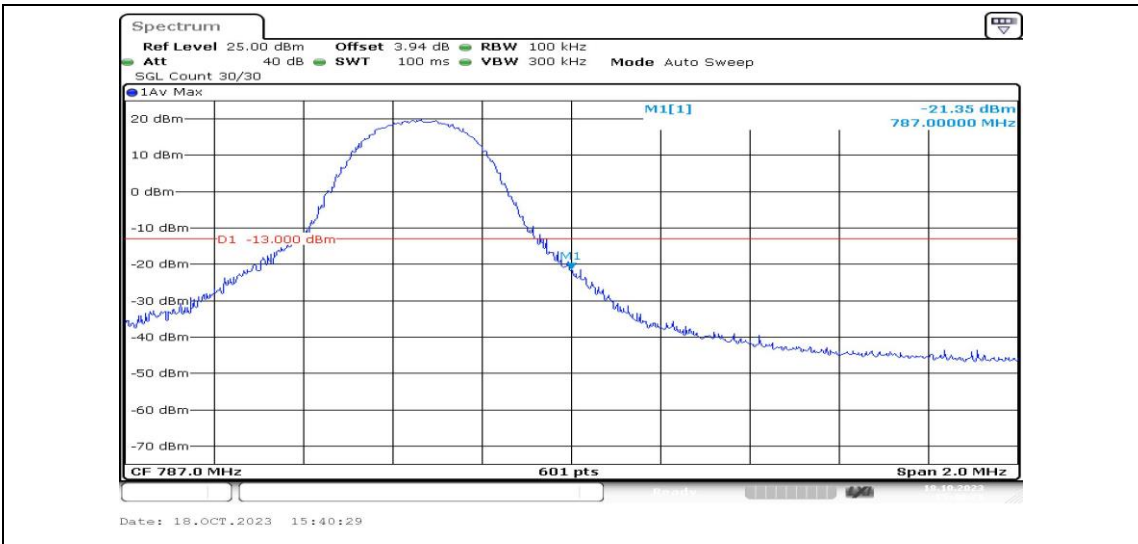
Band13-5MHz-QPSK-23255-1RB#24-PASS
