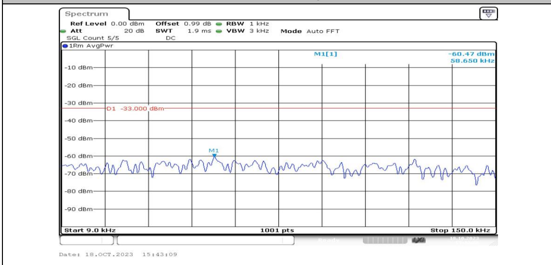
Band13-5MHz-QPSK-23230-1RB#0-Range1:0.009~0.15MHz-PASS
