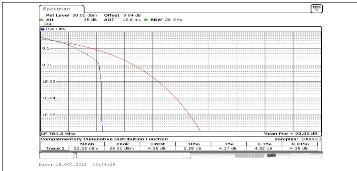
Band13-5MHz-QPSK-23255-1RB#0-PASS
