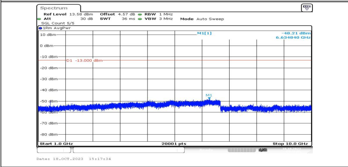
Band12-5MHz-16QAM-23035-1RB#0-Range4:1000~10000MHz-PASS
