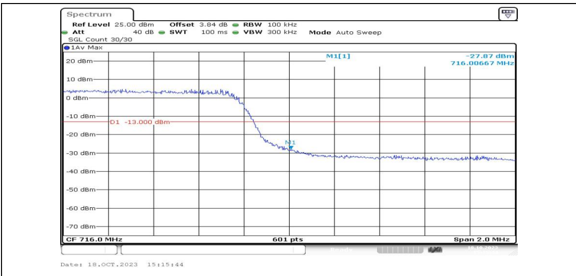
Band12-5MHz-16QAM-23155-25RB#0-PASS
