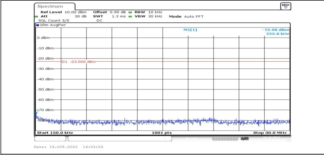
Band12-3MHz-QPSK-23095-1RB#0-Range2:0.15~30MHz-PASS
