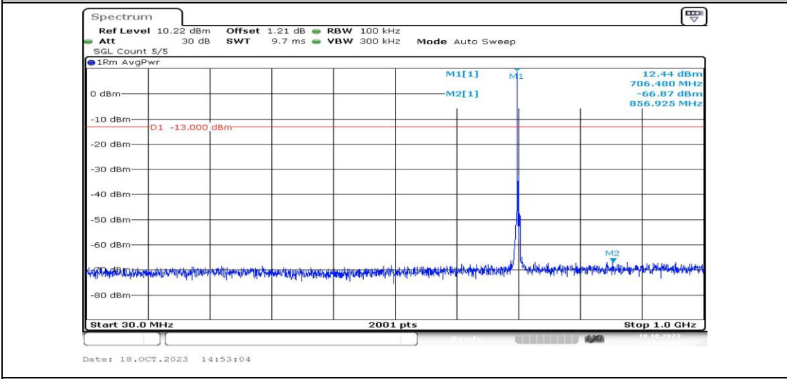
Band12-3MHz-QPSK-23095-1RB#0-Range3:30~1000MHz-PASS
