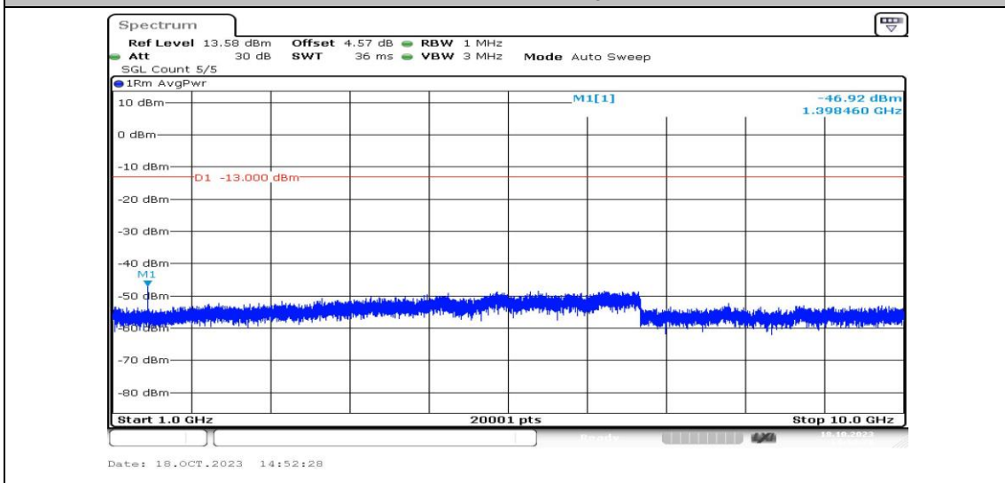
Band12-3MHz-16QAM-23025-1RB#0-Range4:1000~10000MHz-PASS
