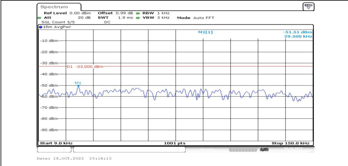
Band12-5MHz-QPSK-23035-1RB#0-Range1:0.009~0.15MHz-PASS
