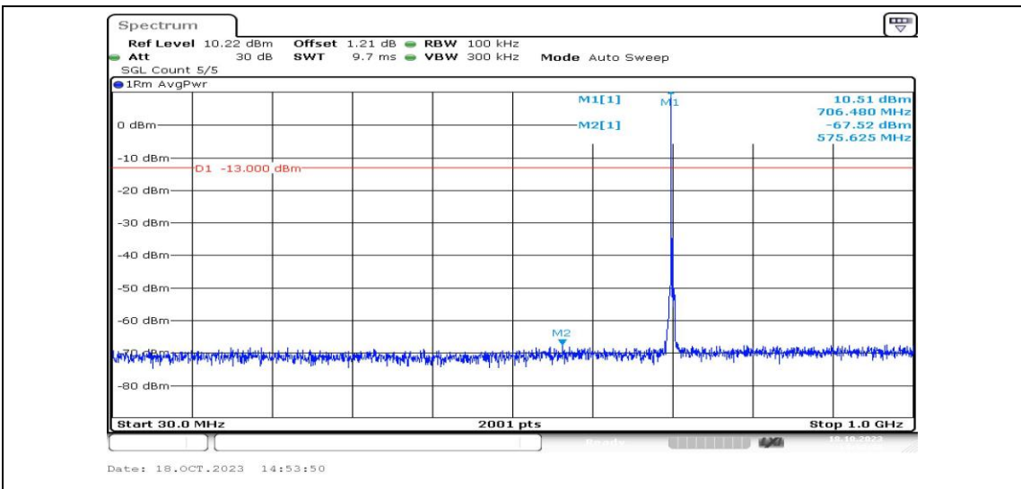
Band12-3MHz-16QAM-23095-1RB#0-Range3:30~1000MHz-PASS
