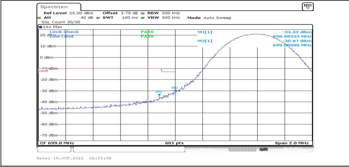
Band12-10MHz-QPSK-23060-1RB#0-PASS
