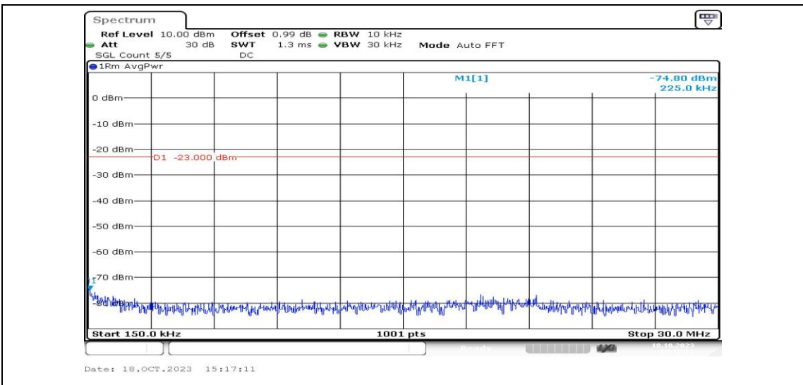
Band12-5MHz-16QAM-23035-1RB#0-Range2:0.15~30MHz-PASS
