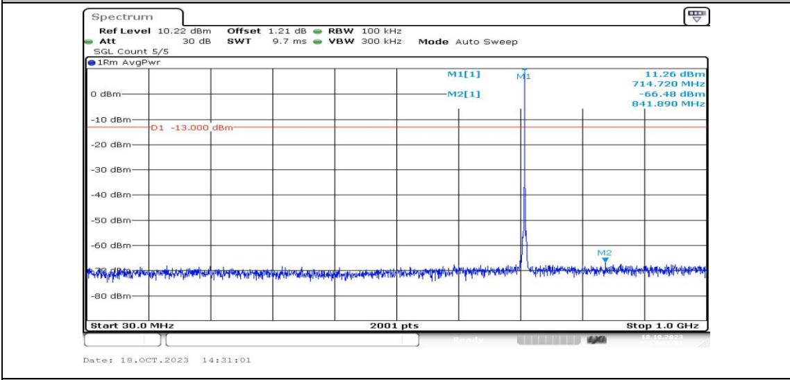
Band12-1.4MHz-16QAM-23173-1RB#0-Range3:30~1000MHz-PASS
