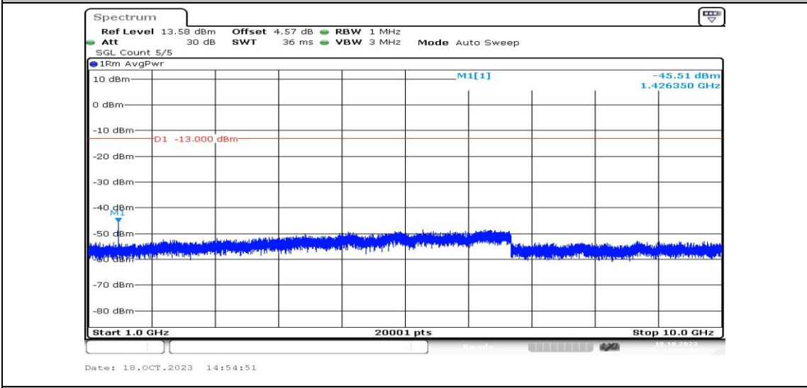
Band12-3MHz-QPSK-23165-1RB#0-Range4:1000~10000MHz-PASS
