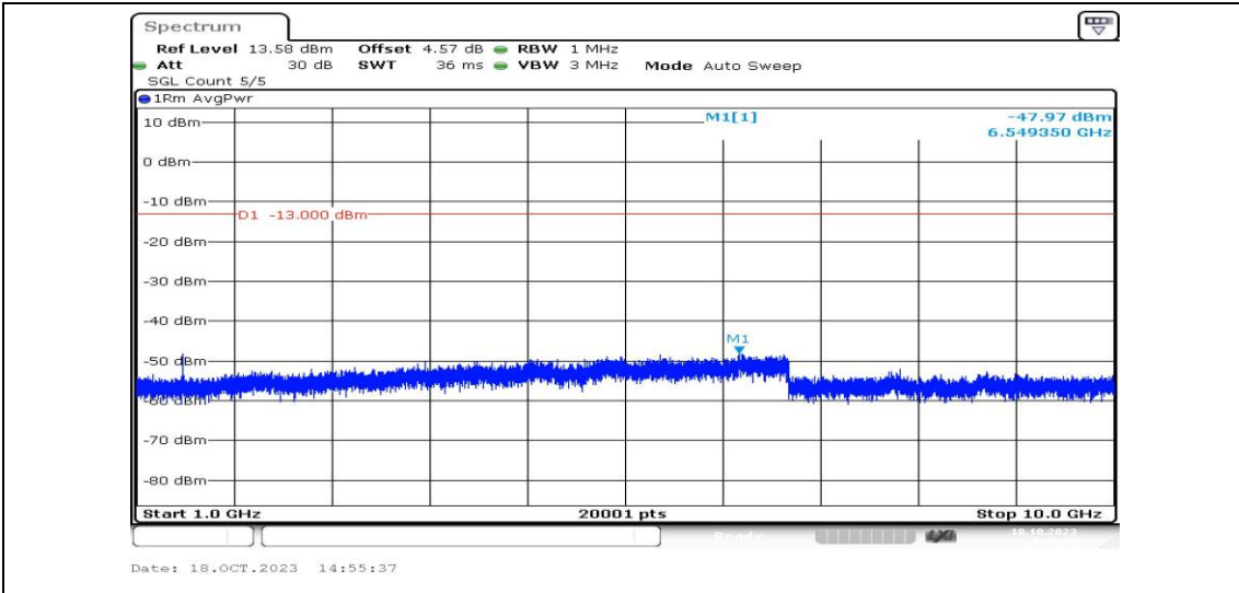
Band12-3MHz-16QAM-23165-1RB#0-Range4:1000~10000MHz-PASS
