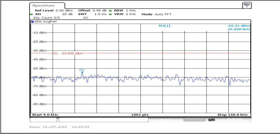
Band12-1.4MHz-16QAM-23095-1RB#0-Range1:0.009~0.15MHz-PASS
