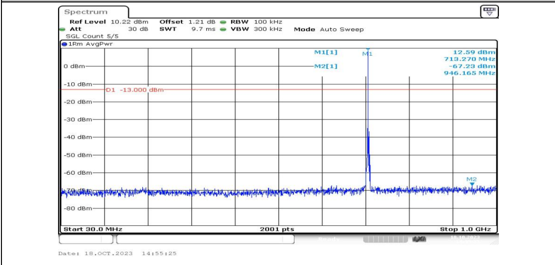
Band12-3MHz-16QAM-23165-1RB#0-Range3:30~1000MHz-PASS
