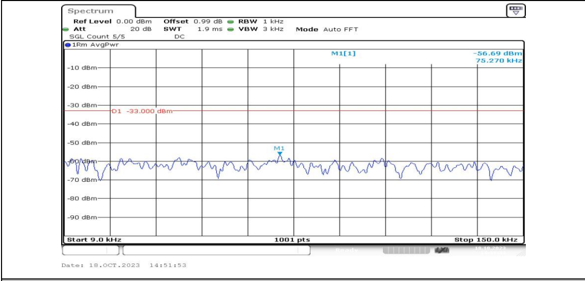
Band12-3MHz-16QAM-23025-1RB#0-Range1:0.009~0.15MHz-PASS
