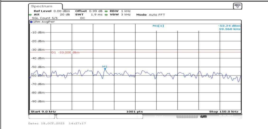
Band12-1.4MHz-16QAM-23017-1RB#0-Range1:0.009~0.15MHz-PASS
