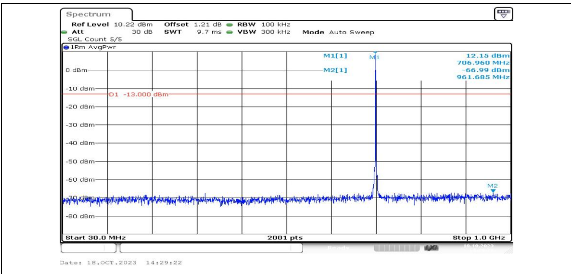
Band12-1.4MHz-16QAM-23095-1RB#0-Range3:30~1000MHz-PASS
