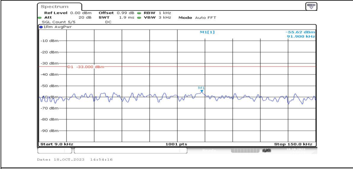
Band12-3MHz-QPSK-23165-1RB#0-Range1:0.009~0.15MHz-PASS
