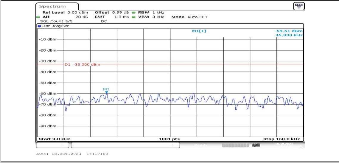
Band12-5MHz-16QAM-23035-1RB#0-Range1:0.009~0.15MHz-PASS
