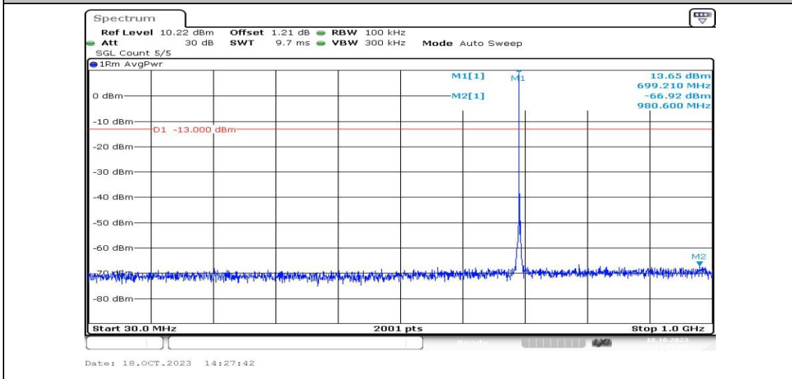
Band12-1.4MHz-16QAM-23017-1RB#0-Range3:30~1000MHz-PASS
