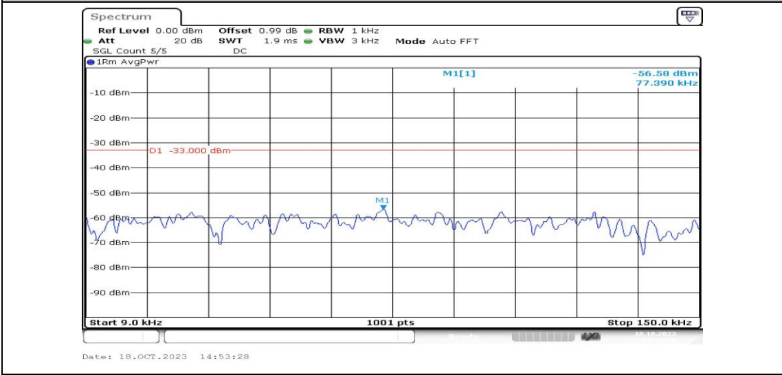
Band12-3MHz-16QAM-23095-1RB#0-Range1:0.009~0.15MHz-PASS
