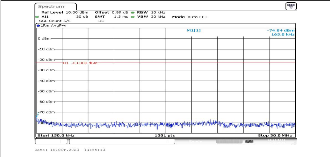
Band12-3MHz-16QAM-23165-1RB#0-Range2:0.15~30MHz-PASS
