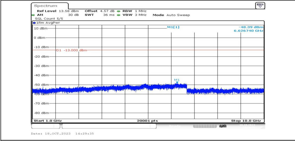
Band12-1.4MHz-16QAM-23095-1RB#0-Range4:1000~10000MHz-PASS
