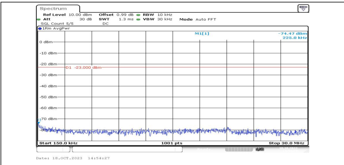
Band12-3MHz-QPSK-23165-1RB#0-Range2:0.15~30MHz-PASS
