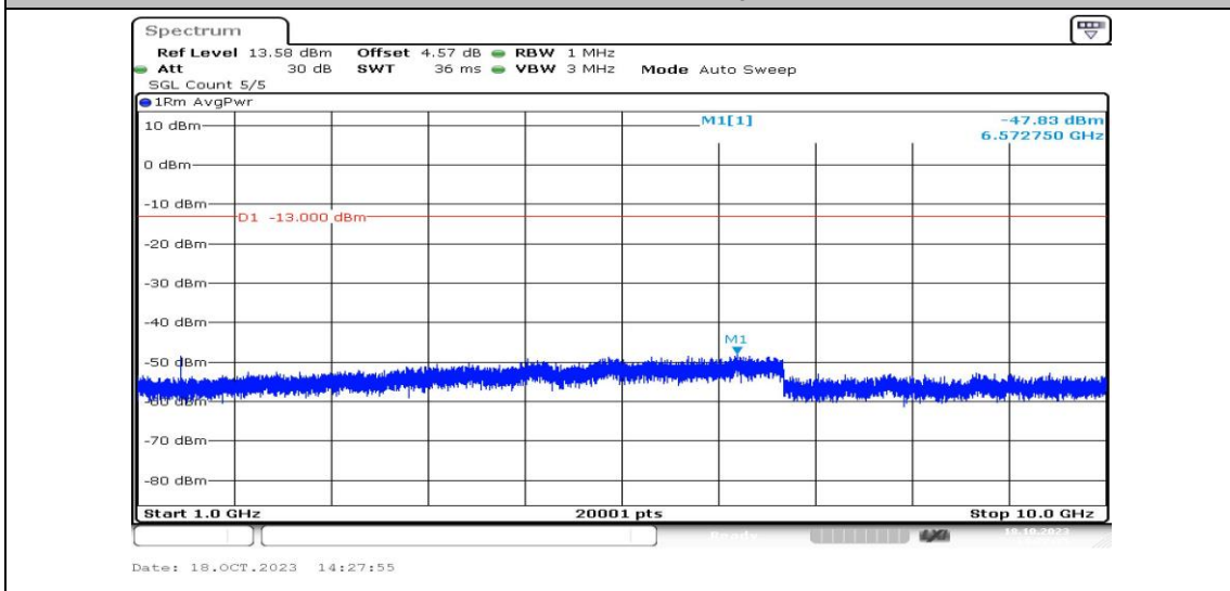
Band12-1.4MHz-16QAM-23017-1RB#0-Range4:1000~10000MHz-PASS
