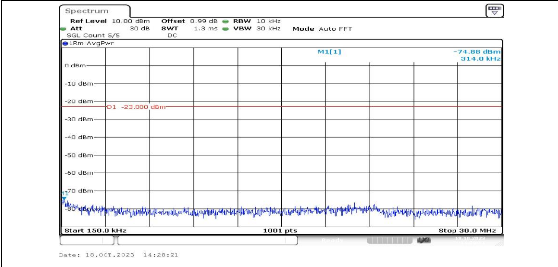
Band12-1.4MHz-QPSK-23095-1RB#0-Range2:0.15~30MHz-PASS
