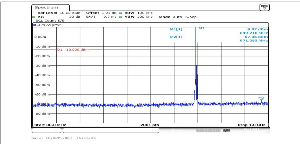
Band12-5MHz-QPSK-23035-1RB#0-Range3:30~1000MHz-PASS
