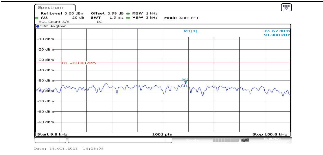
Band12-1.4MHz-QPSK-23095-1RB#0-Range1:0.009~0.15MHz-PASS
