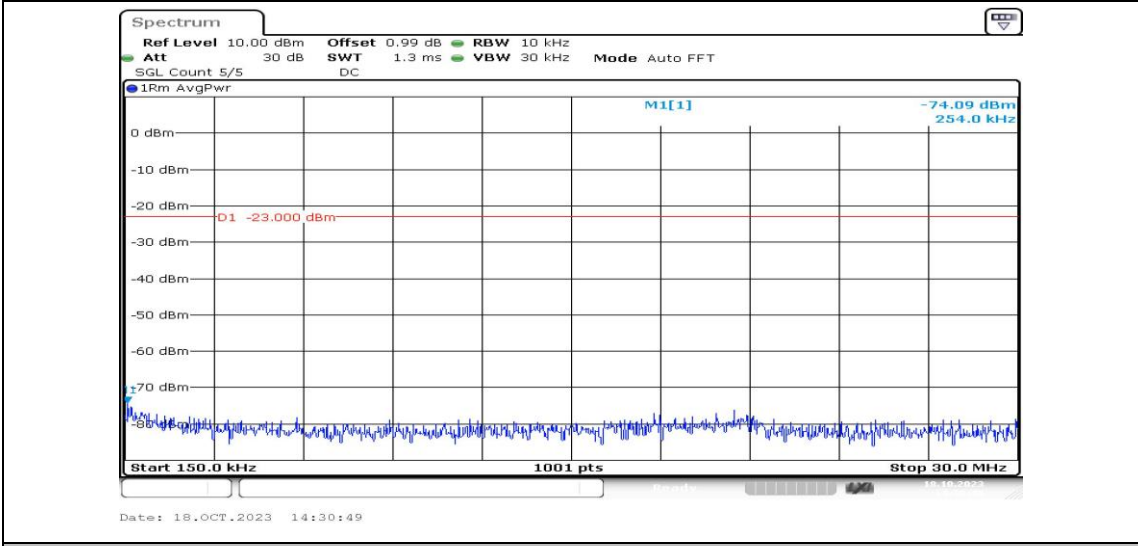
Band12-1.4MHz-16QAM-23173-1RB#0-Range2:0.15~30MHz-PASS
