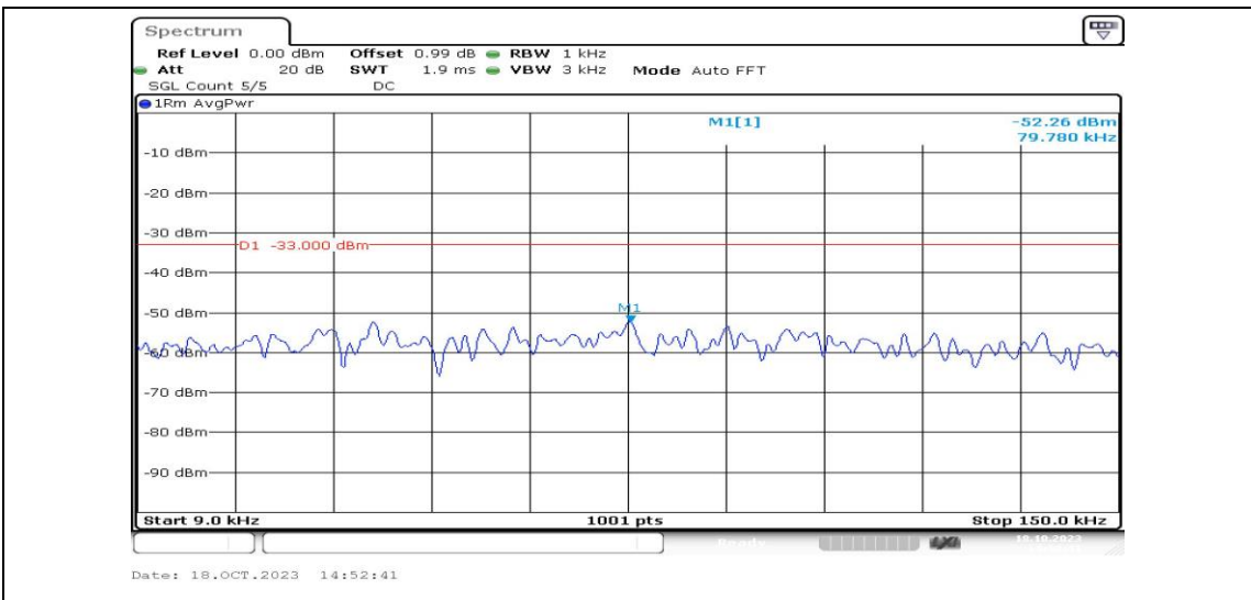
Band12-3MHz-QPSK-23095-1RB#0-Range1:0.009~0.15MHz-PASS
