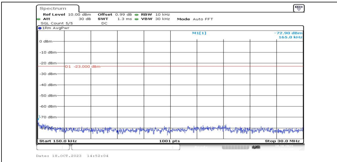
Band12-3MHz-16QAM-23025-1RB#0-Range2:0.15~30MHz-PASS
