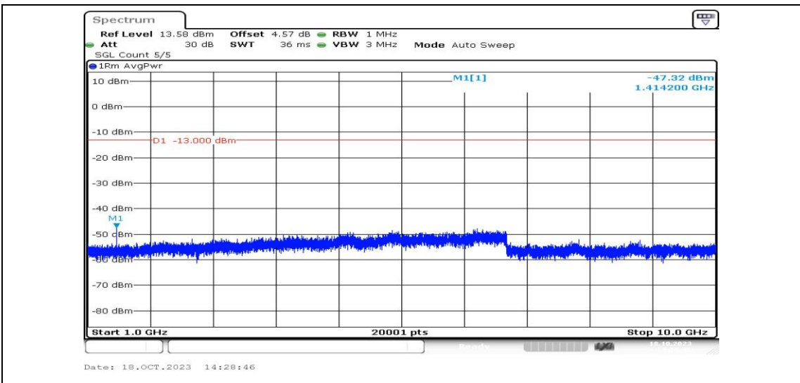
Band12-1.4MHz-QPSK-23095-1RB#0-Range4:1000~10000MHz-PASS
