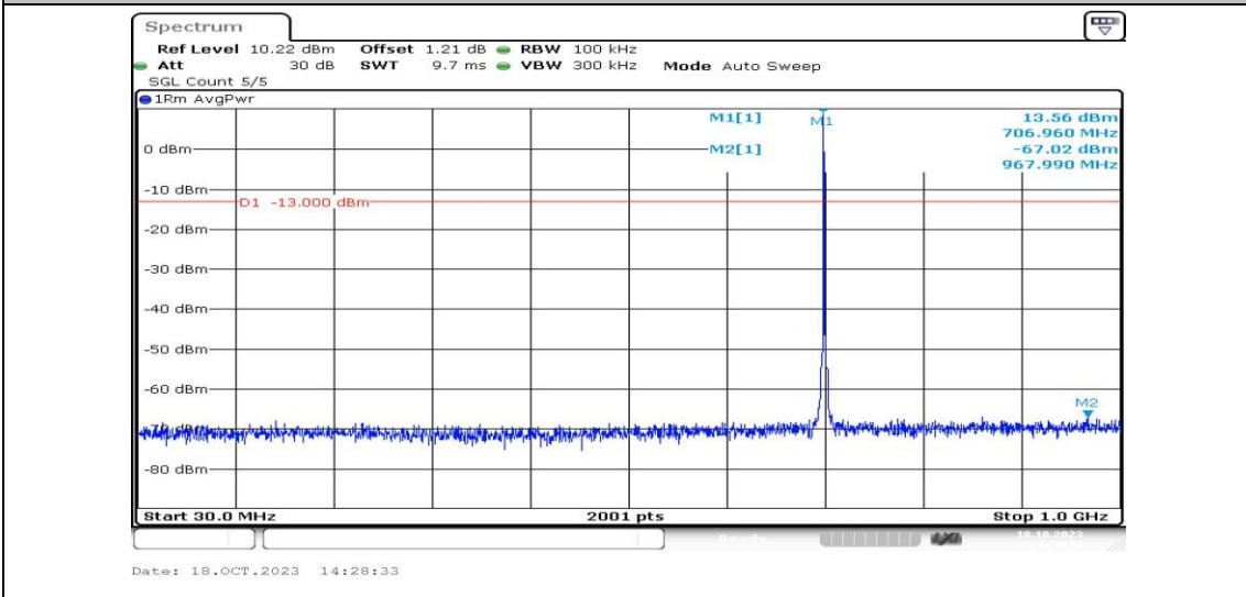
Band12-1.4MHz-QPSK-23095-1RB#0-Range3:30~1000MHz-PASS
