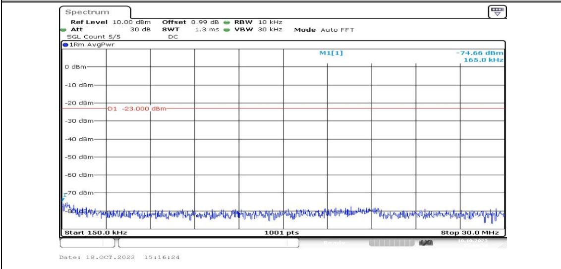
Band12-5MHz-QPSK-23035-1RB#0-Range2:0.15~30MHz-PASS
