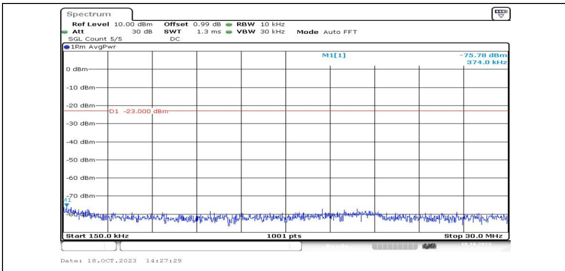
Band12-1.4MHz-16QAM-23017-1RB#0-Range2:0.15~30MHz-PASS
