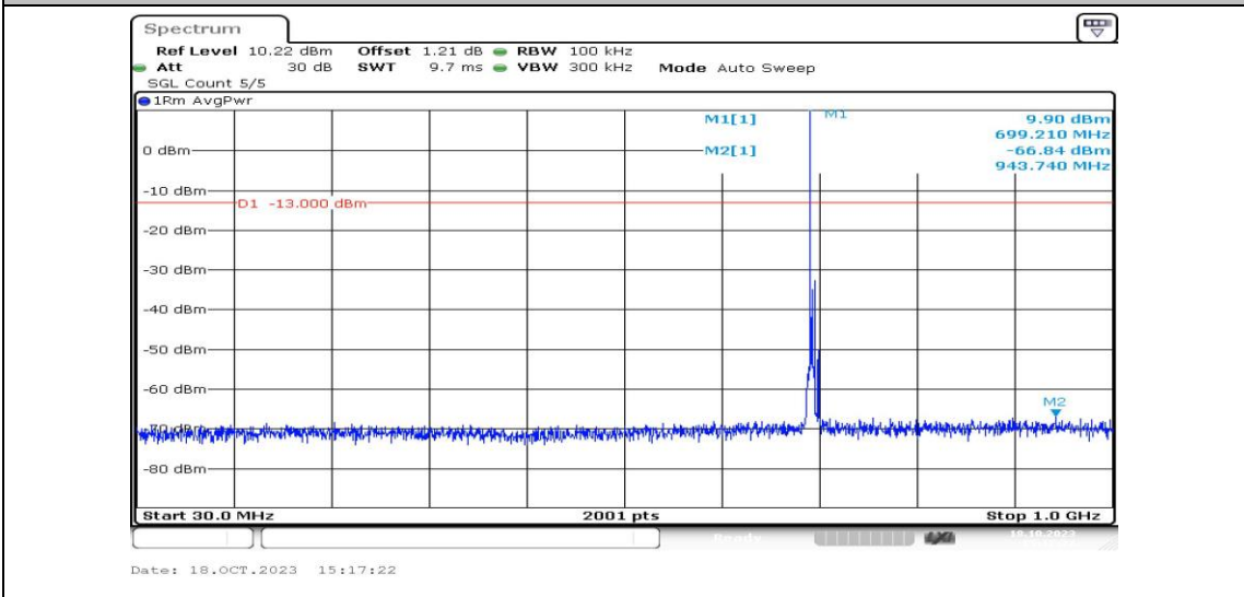
Band12-5MHz-16QAM-23035-1RB#0-Range3:30~1000MHz-PASS
