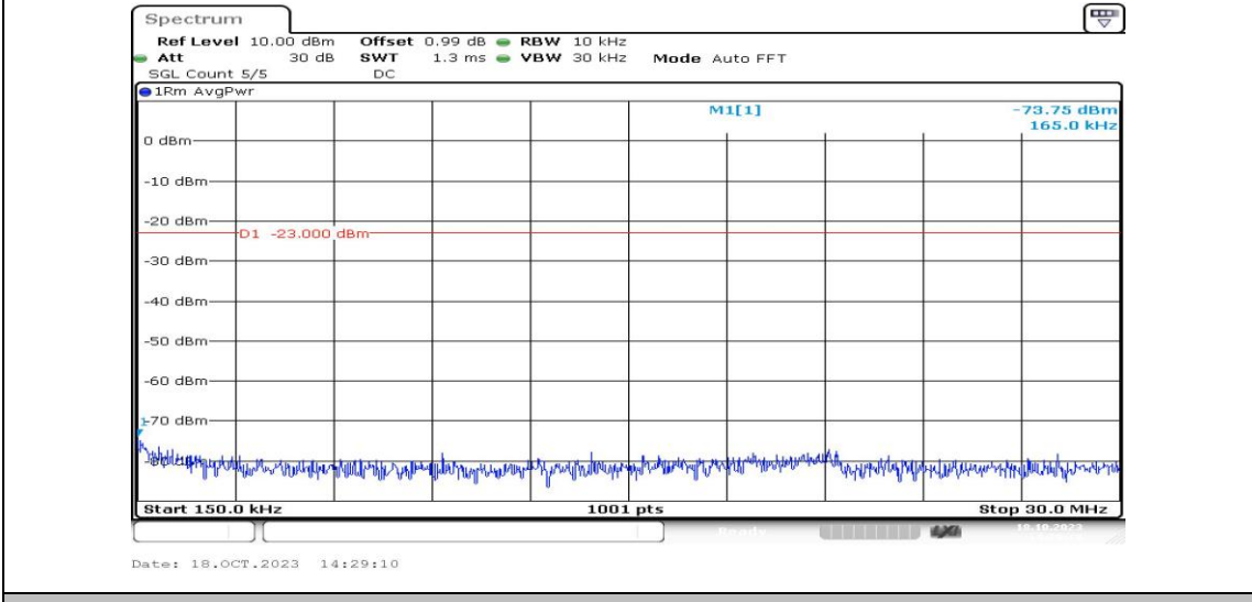
Band12-1.4MHz-16QAM-23095-1RB#0-Range2:0.15~30MHz-PASS
