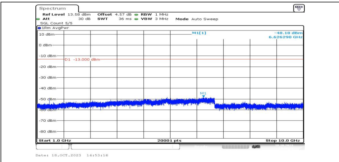
Band12-3MHz-QPSK-23095-1RB#0-Range4:1000~10000MHz-PASS
