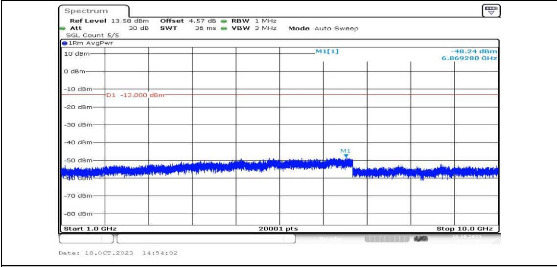
Band12-3MHz-16QAM-23095-1RB#0-Range4:1000~10000MHz-PASS
