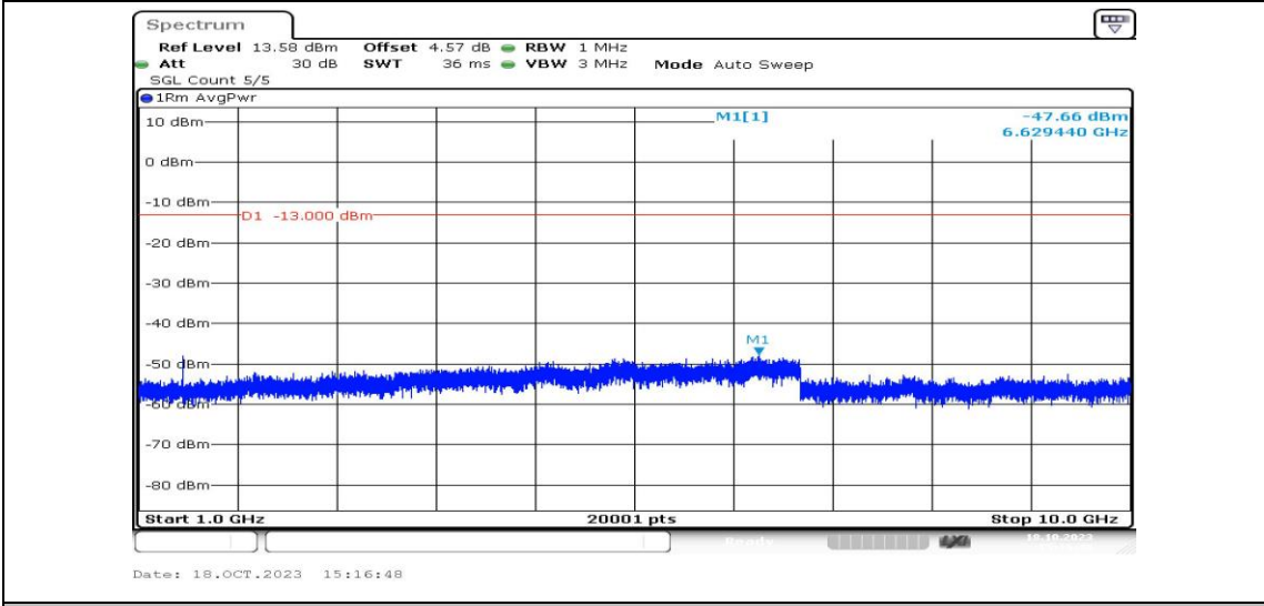
Band12-5MHz-QPSK-23035-1RB#0-Range4:1000~10000MHz-PASS
