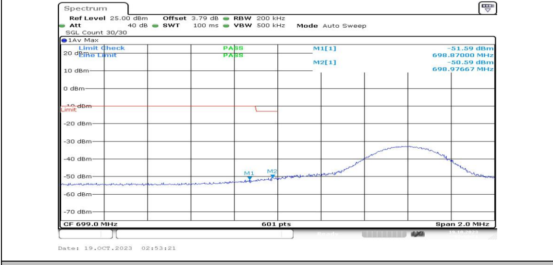
Band12-10MHz-QPSK-23060-1RB#49-PASS
