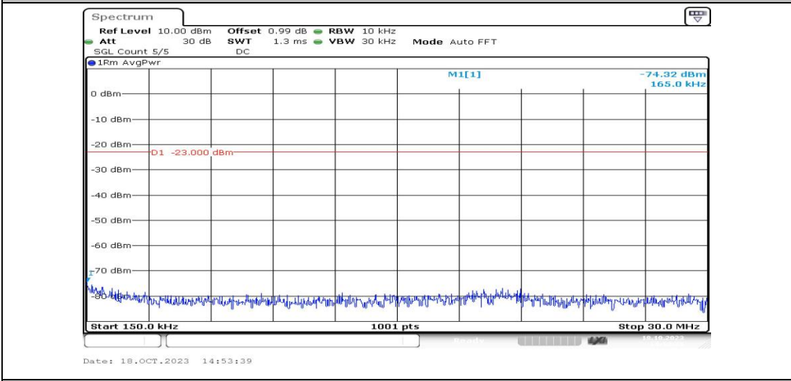
Band12-3MHz-16QAM-23095-1RB#0-Range2:0.15~30MHz-PASS
