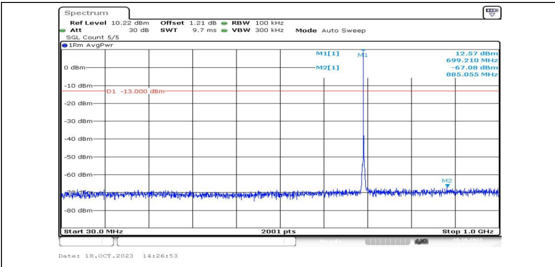
Band12-1.4MHz-QPSK-23017-1RB#0-Range3:30~1000MHz-PASS
