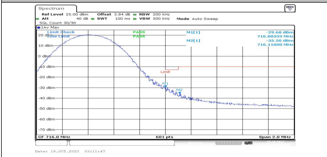
Band12-10MHz-16QAM-23130-1RB#49-PASS
