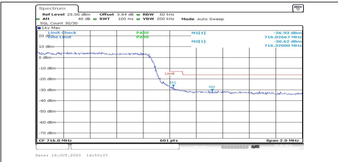
Band12-3MHz-16QAM-23165-15RB#0-PASS
