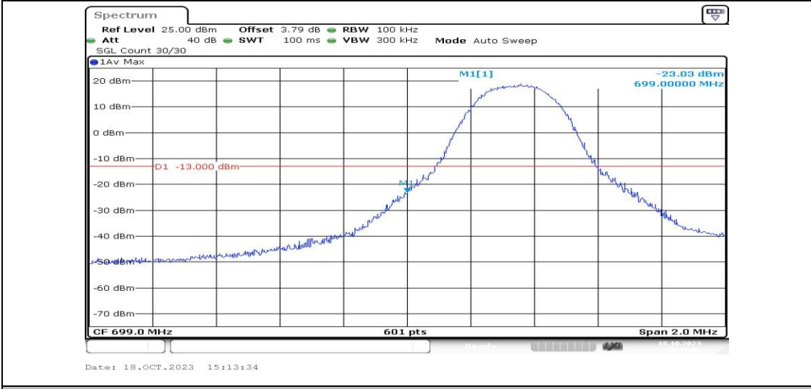
Band12-5MHz-16QAM-23035-1RB#0-PASS
