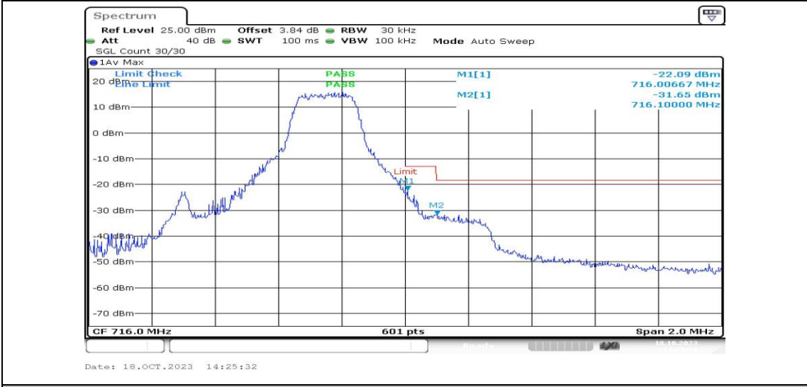
Band12-1.4MHz-16QAM-23173-1RB#5-PASS
