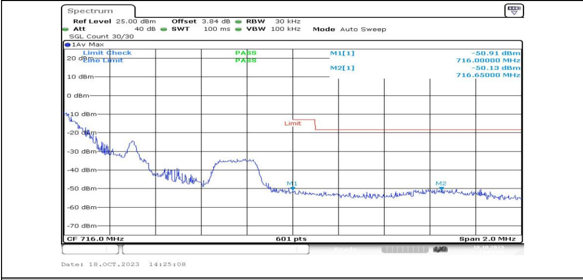
Band12-1.4MHz-16QAM-23173-1RB#0-PASS
