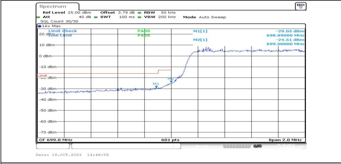
Band12-3MHz-QPSK-23025-15RB#0-PASS
