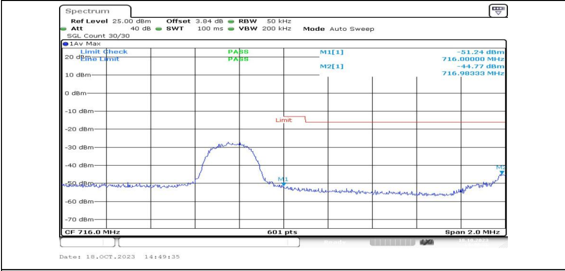
Band12-3MHz-QPSK-23165-1RB#0-PASS
