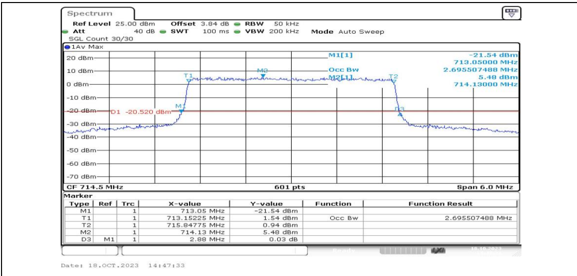
Band12-3MHz-16QAM-23165-15RB#0-PASS
