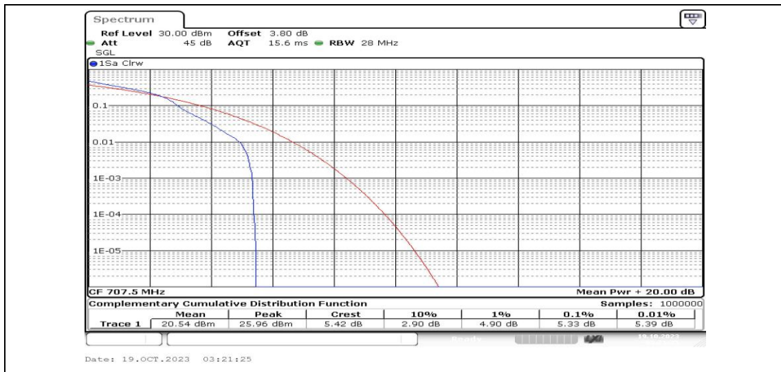
Band12-10MHz-16QAM-23095-1RB#0-PASS
