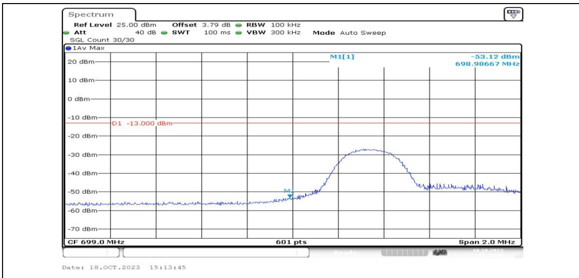
Band12-5MHz-QPSK-23035-1RB#24-PASS
