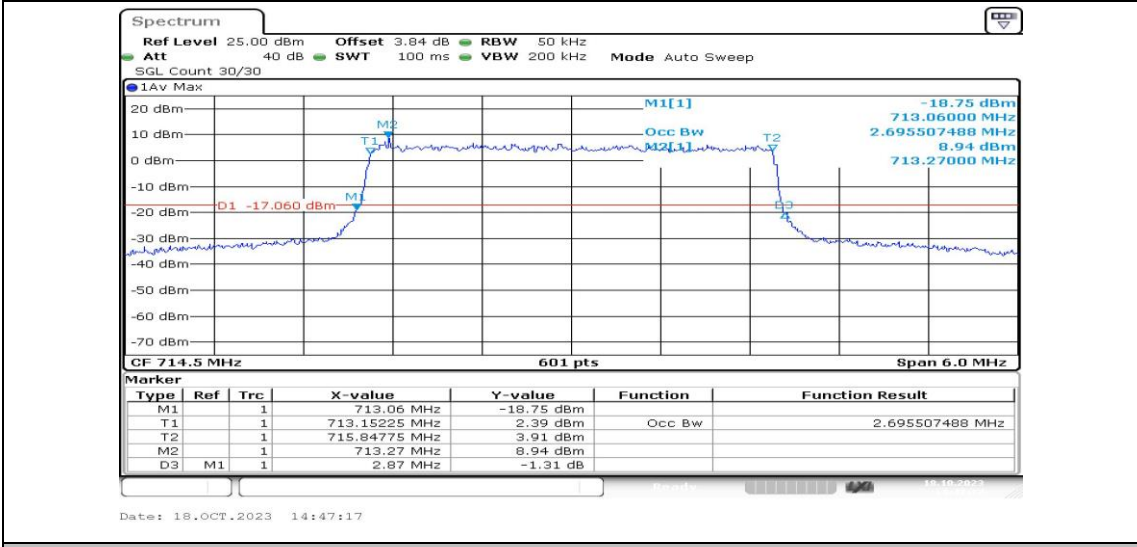
Band12-3MHz-QPSK-23165-15RB#0-PASS
