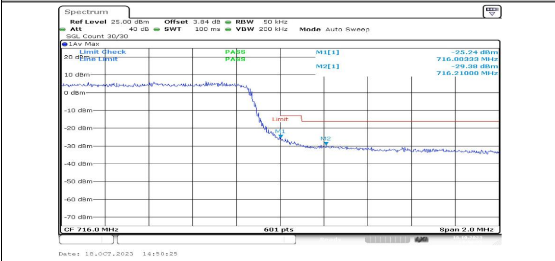
Band12-3MHz-QPSK-23165-15RB#0-PASS
