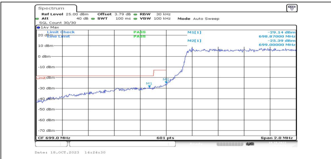
Band12-1.4MHz-16QAM-23017-6RB#0-PASS
