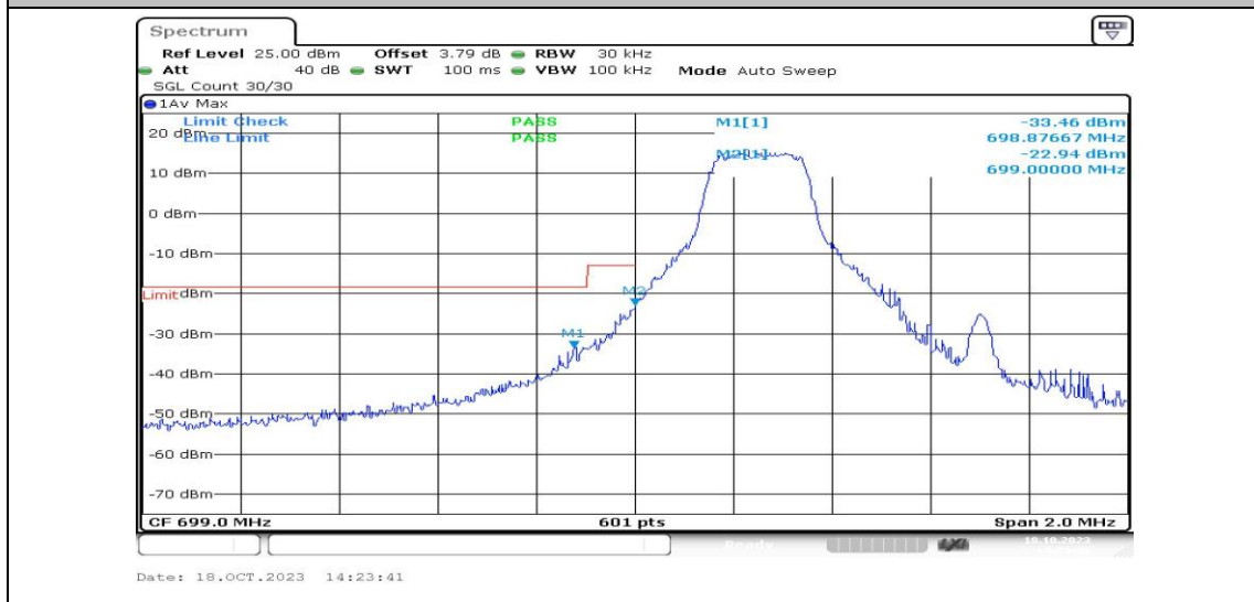
Band12-1.4MHz-16QAM-23017-1RB#0-PASS
