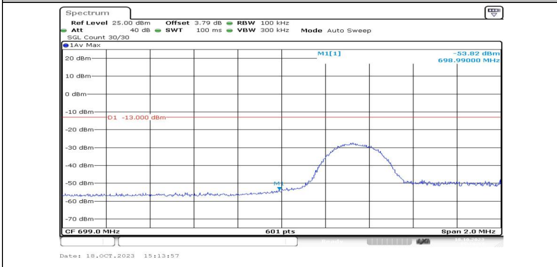
Band12-5MHz-16QAM-23035-1RB#24-PASS
