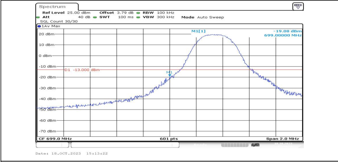
Band12-5MHz-QPSK-23035-1RB#0-PASS
