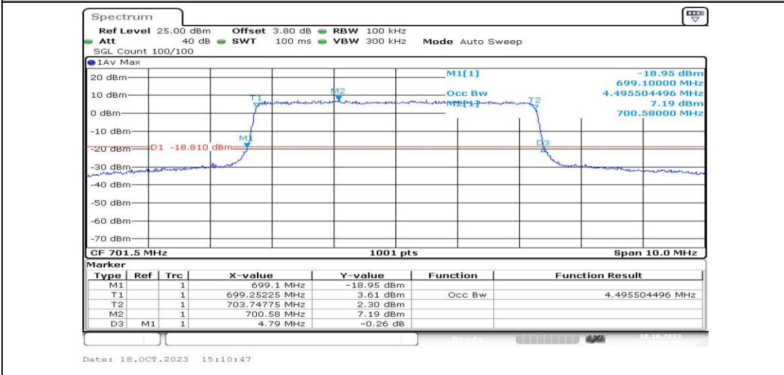
Band12-5MHz-QPSK-23035-25RB#0-PASS
