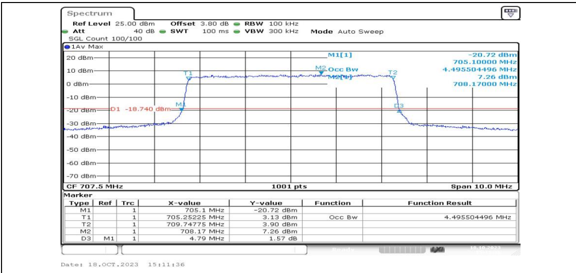
Band12-5MHz-QPSK-23095-25RB#0-PASS
