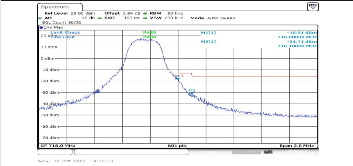
Band12-3MHz-16QAM-23165-1RB#14-PASS
