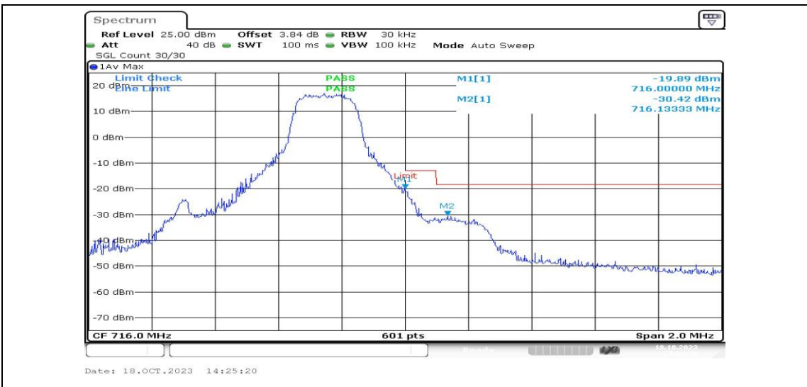
Band12-1.4MHz-QPSK-23173-1RB#5-PASS
