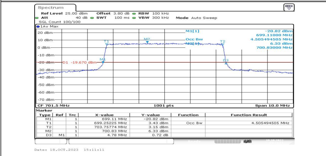
Band12-5MHz-16QAM-23035-25RB#0-PASS
