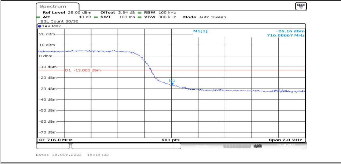
Band12-5MHz-QPSK-23155-25RB#0-PASS
