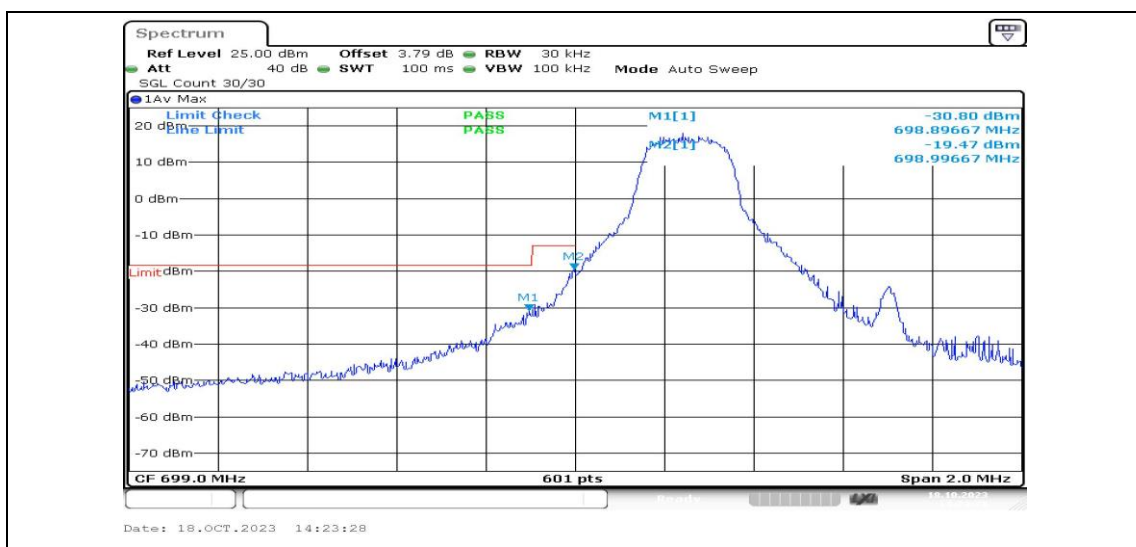
Band12-1.4MHz-QPSK-23017-1RB#0-PASS
