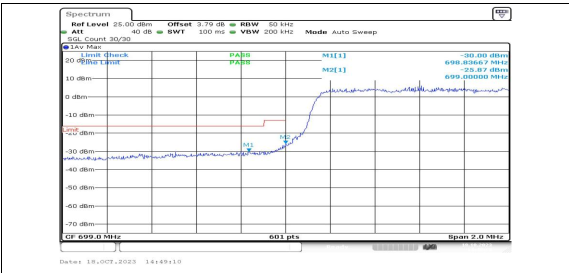
Band12-3MHz-16QAM-23025-15RB#0-PASS
