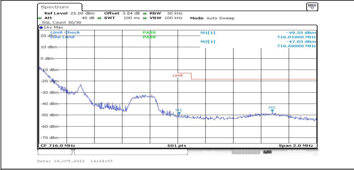
Band12-1.4MHz-QPSK-23173-1RB#0-PASS
