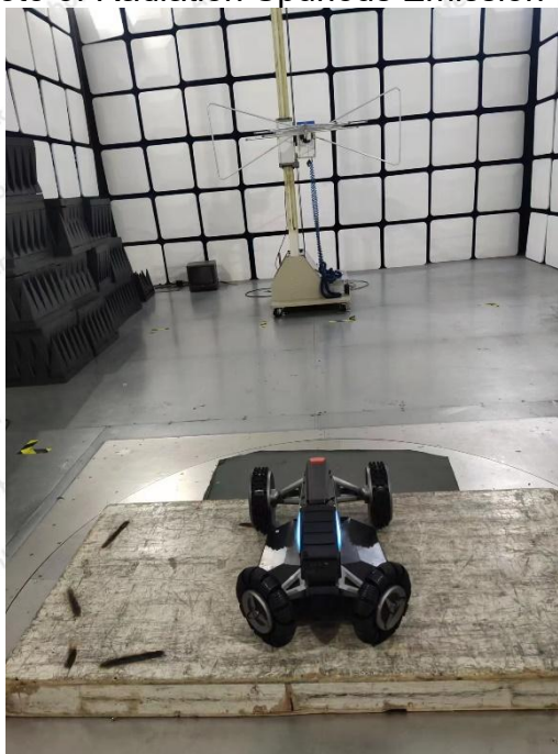
Photo of Radiation Spurious Emission Test
