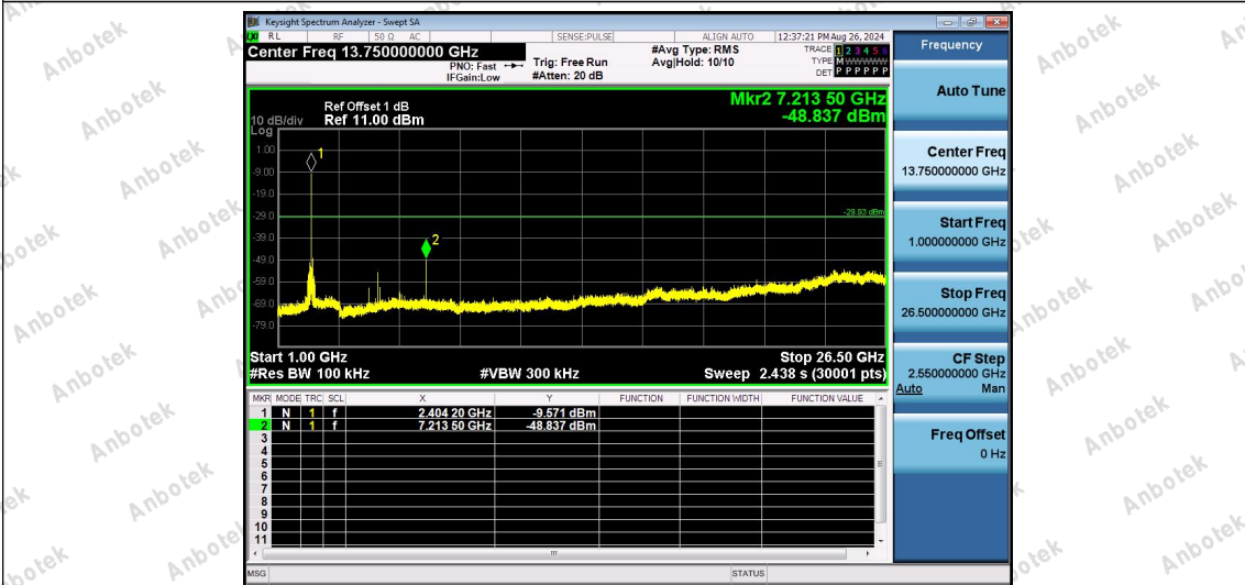
2.4G-Ant1-2405-1000~26500-PASS
