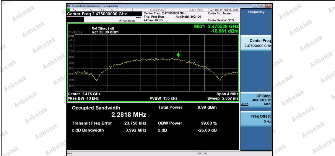
2.4G-Ant1-2475
