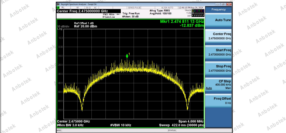
2.4G-Ant1-2475-PASS
