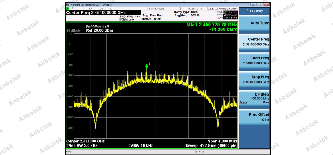
2.4G-Ant1-2451-PASS
