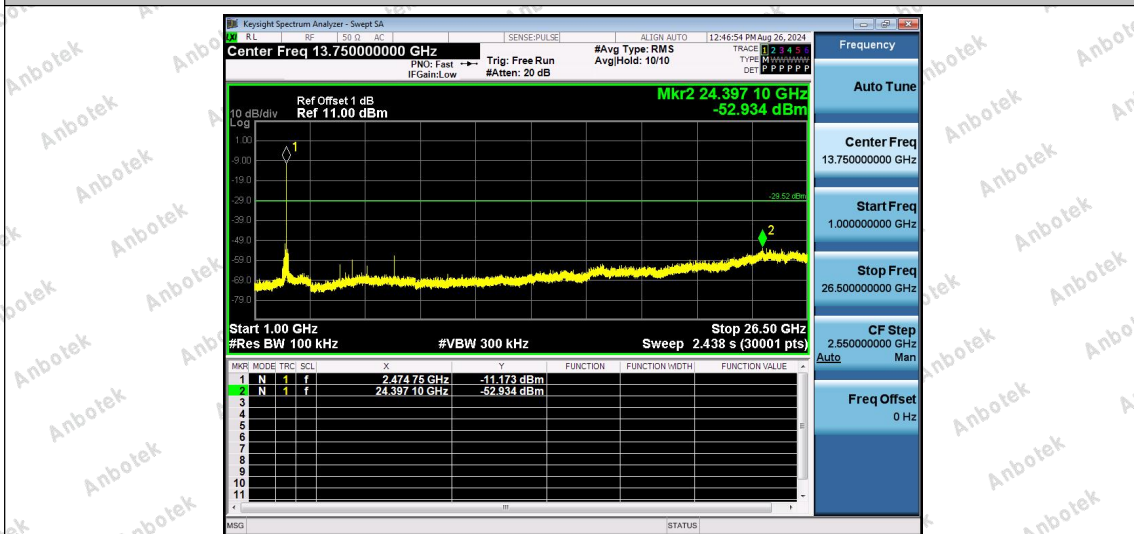
2.4G-Ant1-2475-1000~26500-PASS
