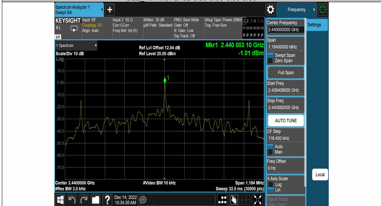
BLE_1M-Ant1-2440--1.01-0.00-0.00-0.00
