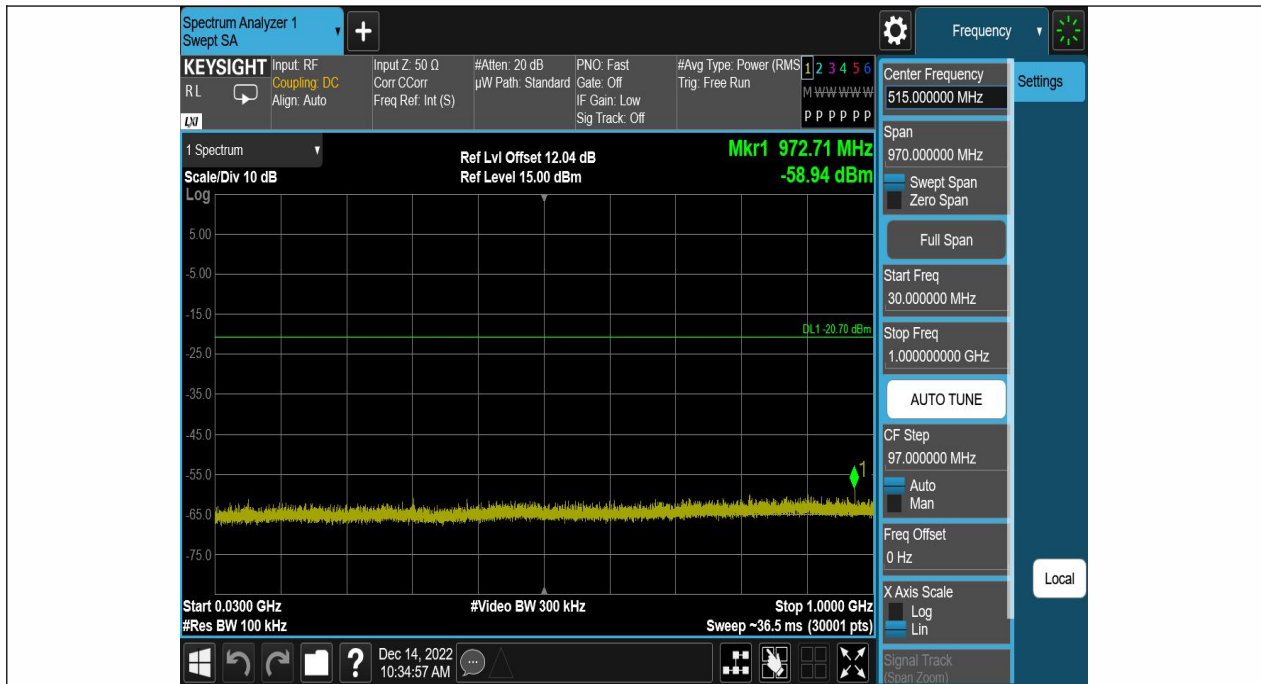
BLE_1M-Ant1-2440-30~1000--0.70
