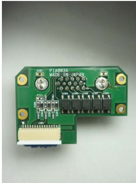
PCB3(Rear)
