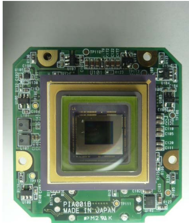
PCB1(Front)
