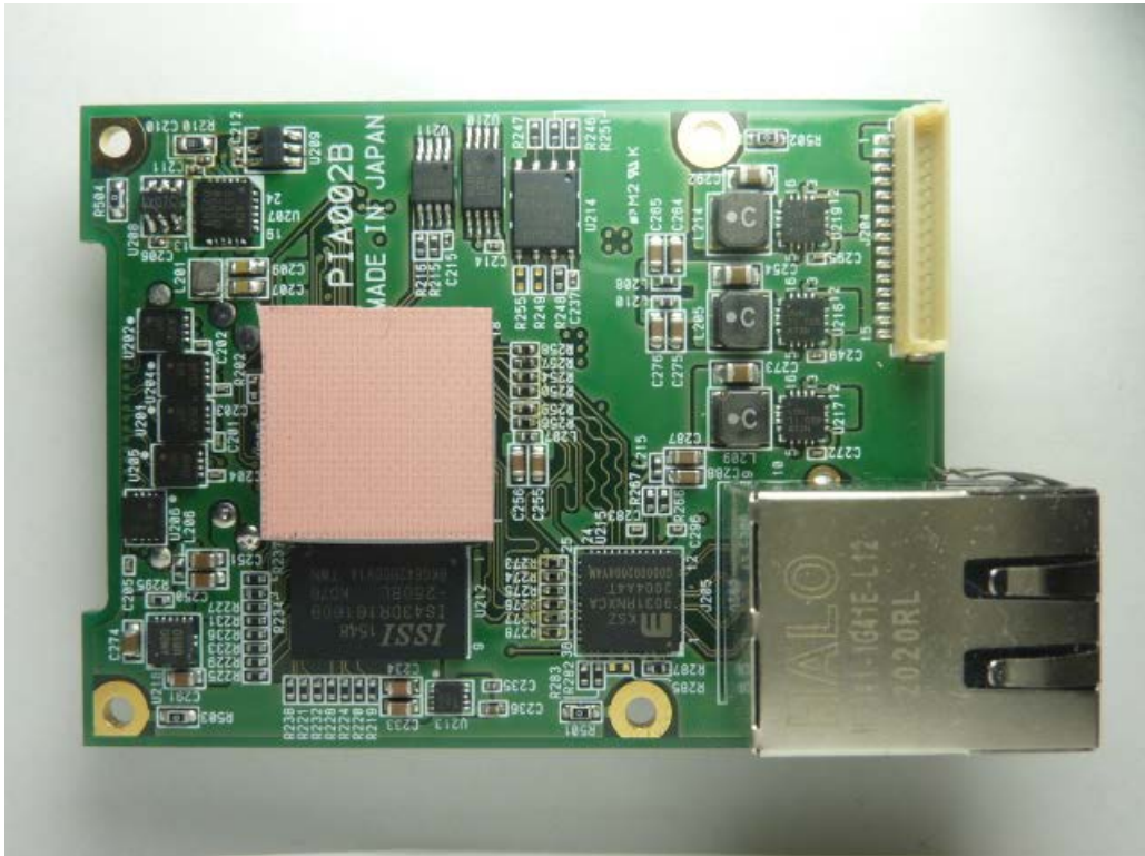
PCB2(Front)
