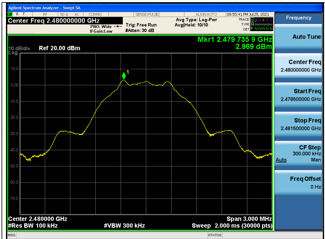
Test_Graph_LE1M_ANT1_2480_1Mbps_Reference Level
