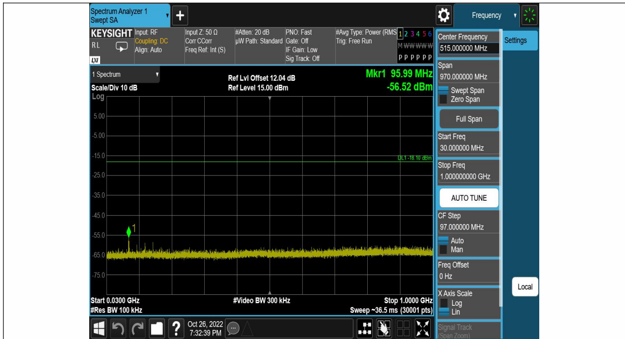
BLE_1M-Ant1-2440-30~1000-1.90
