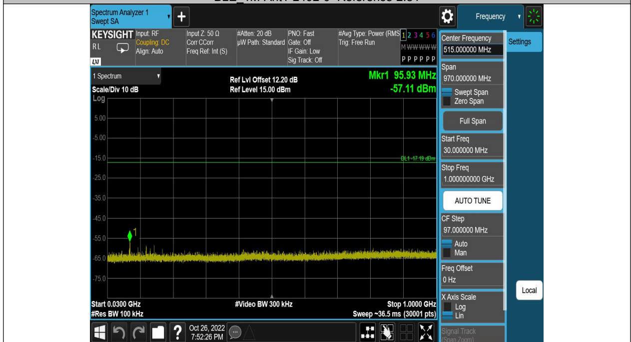
BLE_1M-Ant1-2402-30~1000-2.81
