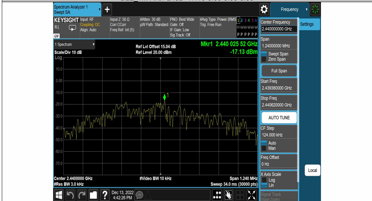
BLE_1M-Ant1-2440--17.13-0.00-0.00-0.00
