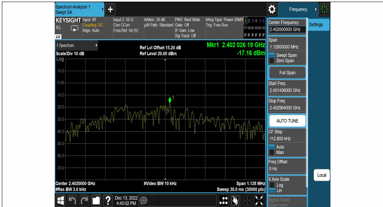
BLE_1M-Ant1-2402--17.16-0.00-0.00-0.00
