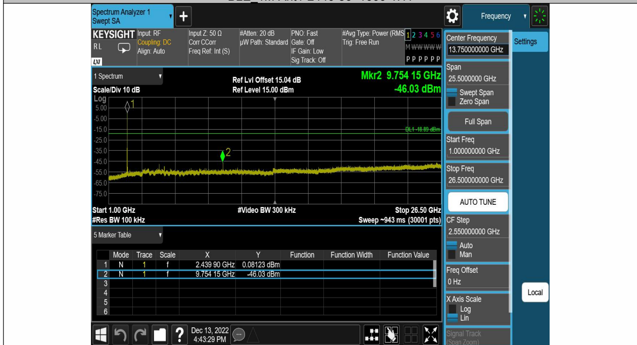
BLE_1M-Ant1-2440-1000~26500-1.11
