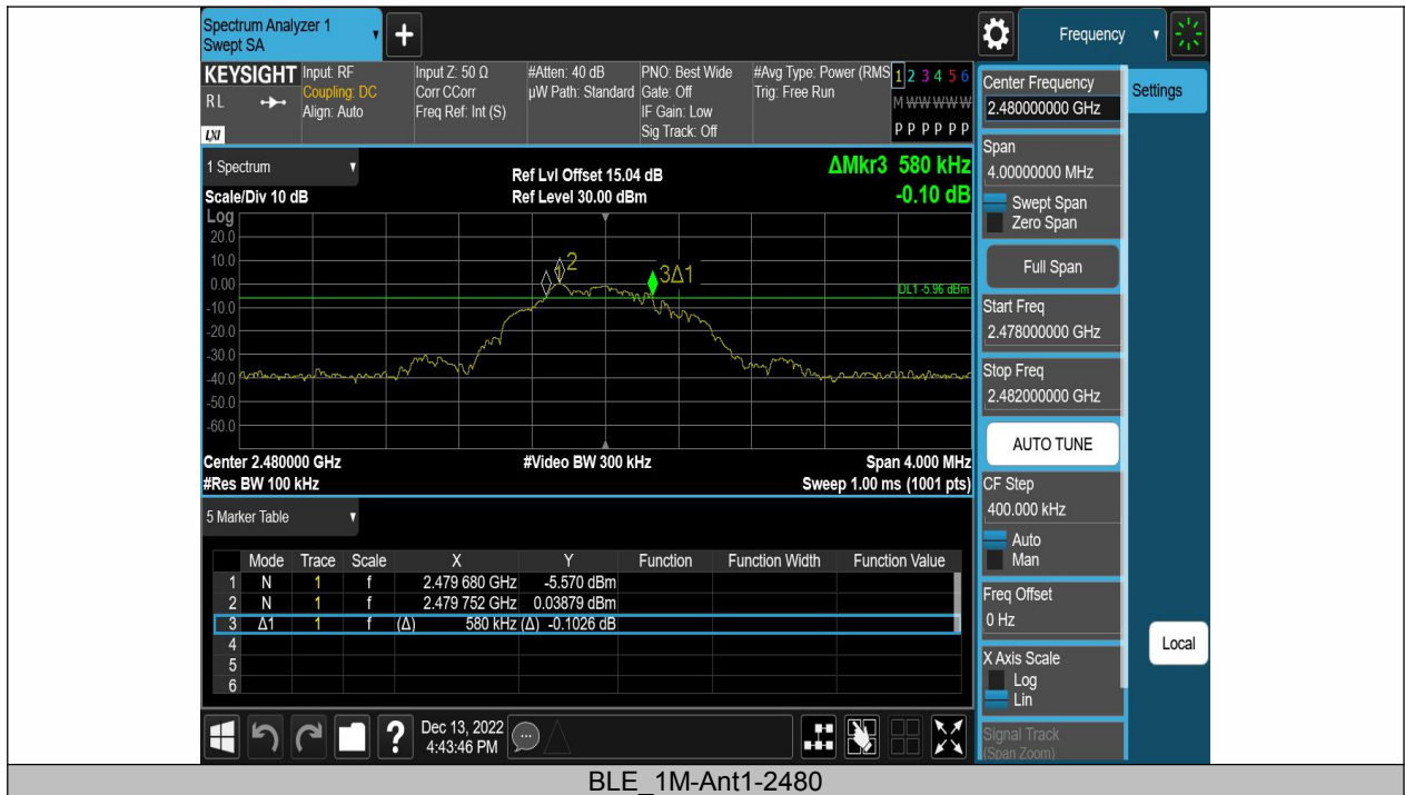
BLE_1M-Ant1-2480
