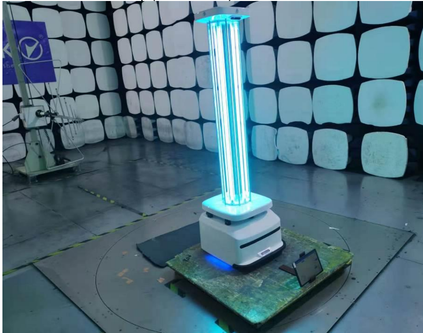
Spurious Emission Test Setup (Below 1GHz)
