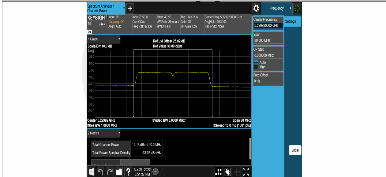
11AC40SISO_Ant2_5230
