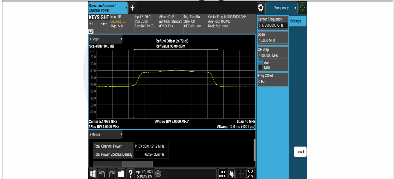
11AC20SISO_Ant2_5180
