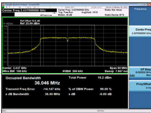
6dB Bandwidth-802.11n(HT40),2437MHz
