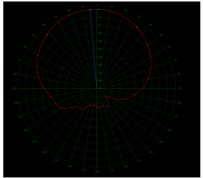
1269MHz Pattern Graph
