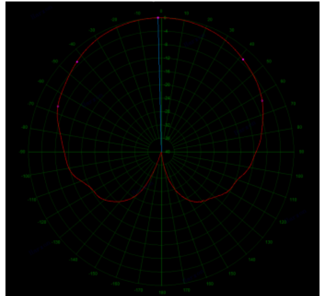
1610MHz Pattern Graph
