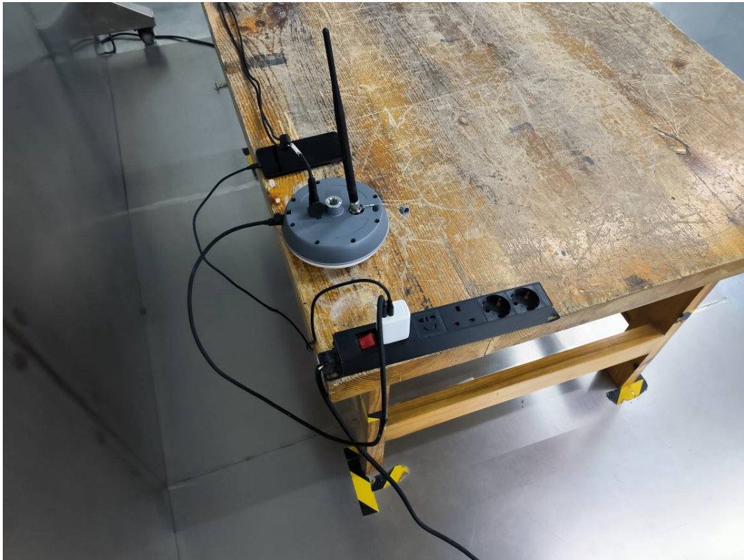
Conducted Emissions Side View USB-A Power Supply
