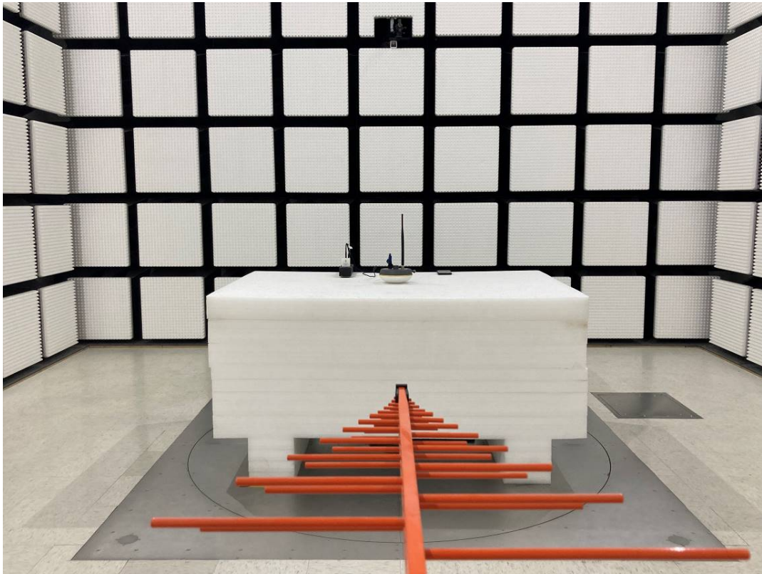
Radiated Emission Below 1GHz View USB-C Power Supply
