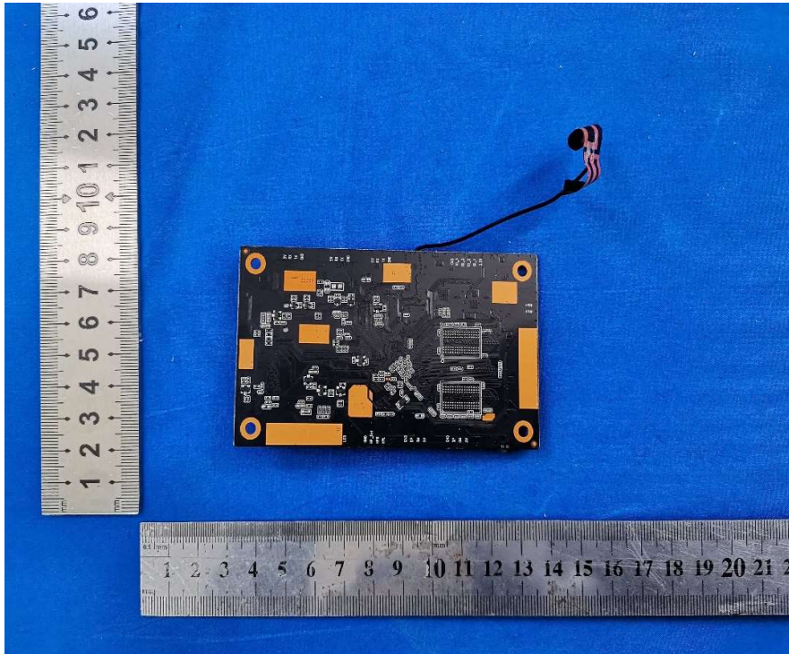
Control PCB view for both models
