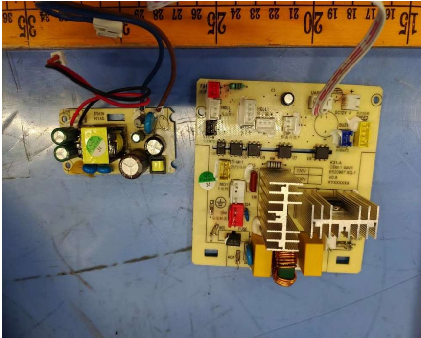
Power PCB for both models
