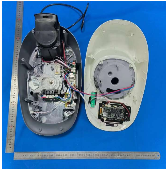
Internal of K3118
