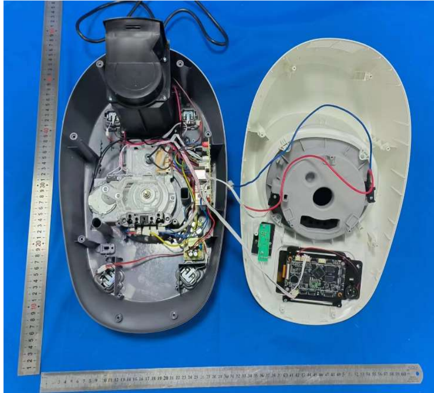
Internal of K3113
