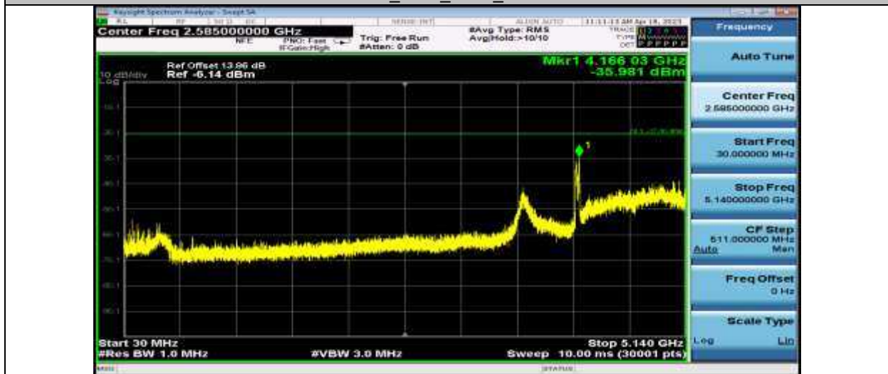
11AC40SISO_Ant1_5190_30~5140
