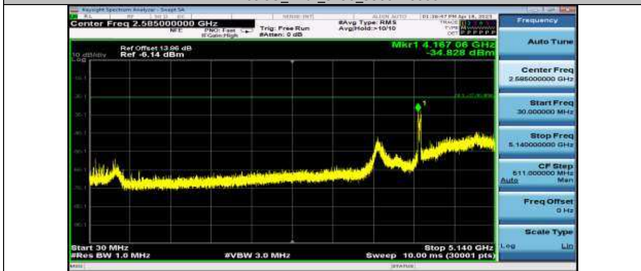
11AX40SISO_Ant1_5230_30~5140
