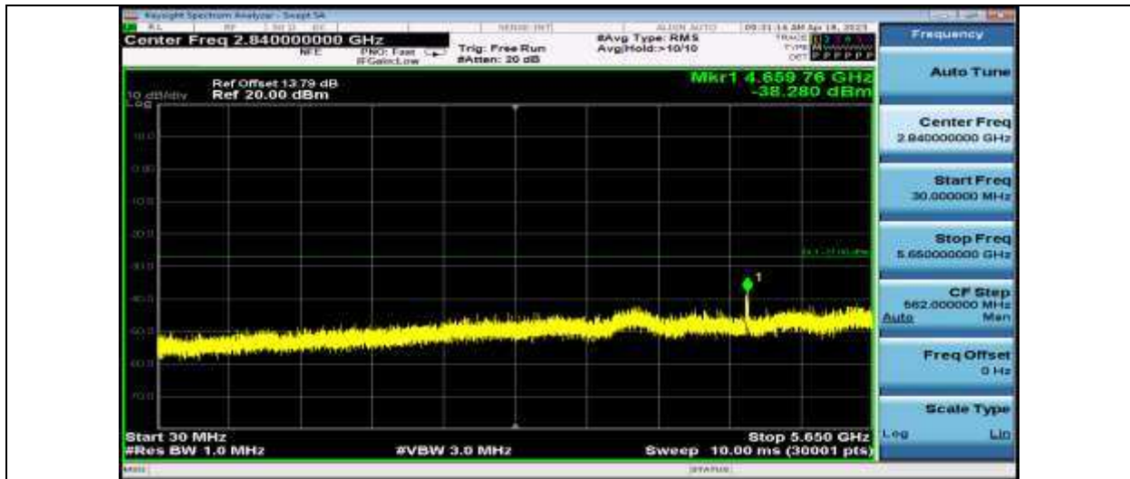
11N20SISO_Ant1_5825_30~5650
