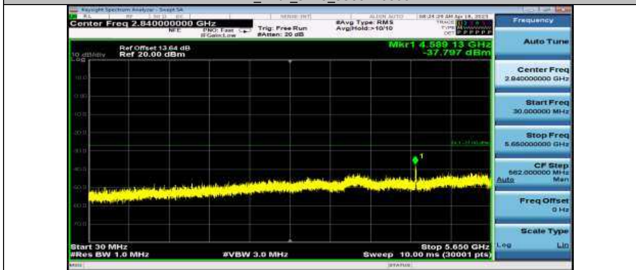
11A_Ant1_5745_30~5650
