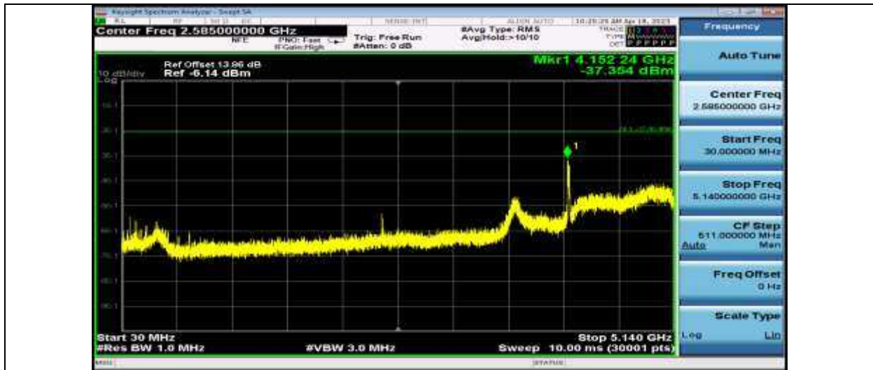
11AC20SISO_Ant1_5200_30~5140
