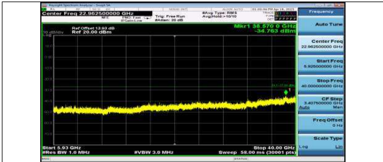
11AX20SISO_Ant1_5785_5925~40000
