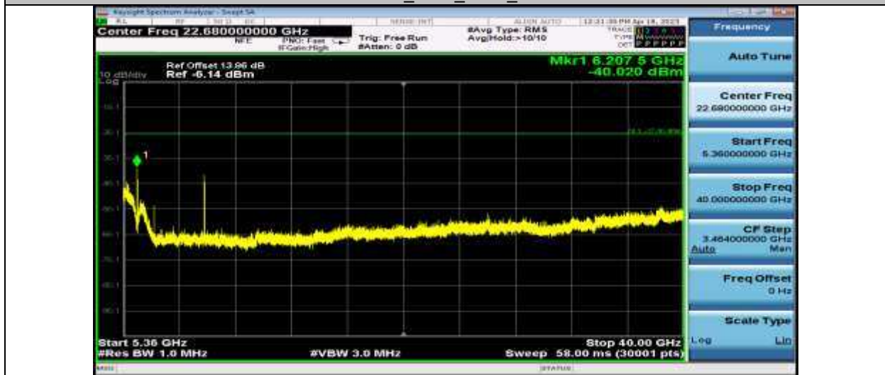
11AX20SISO_Ant1_5180_5360~40000
