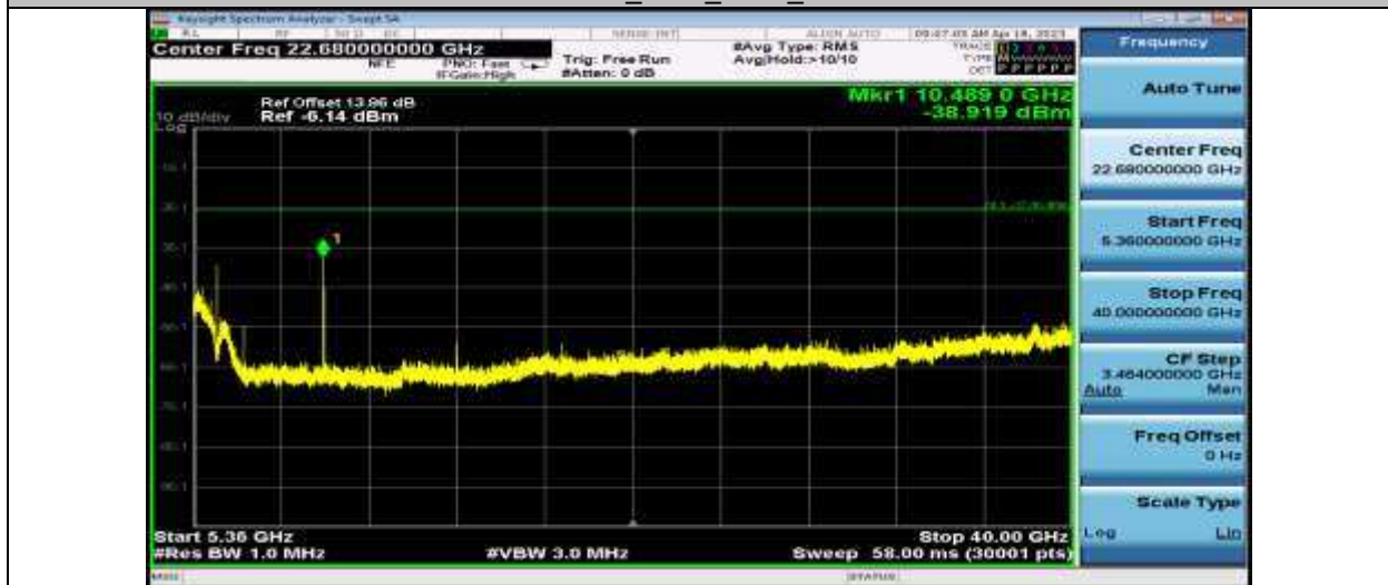
11N20SISO_Ant1_5240_5360~40000
