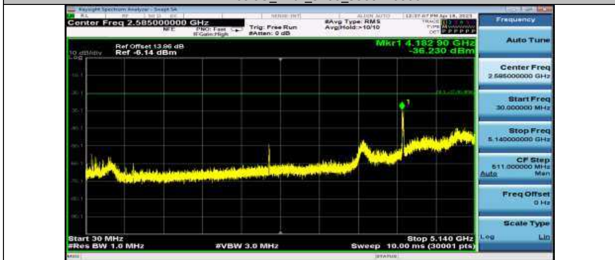
11AX20SISO_Ant1_5240_30~5140
