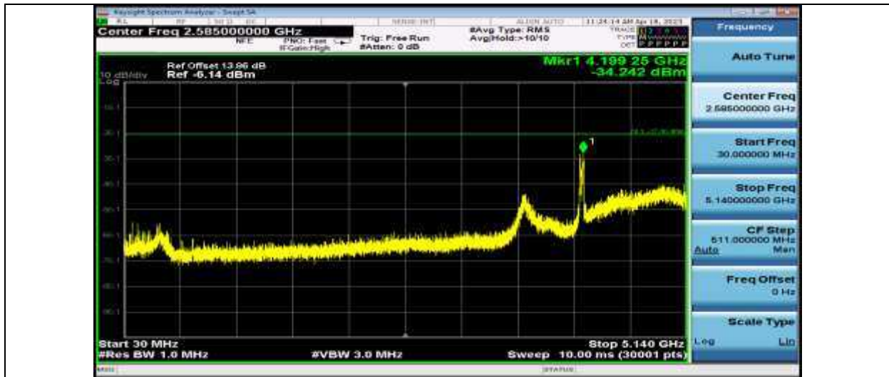
11AC40SISO_Ant1_5230_30~5140
