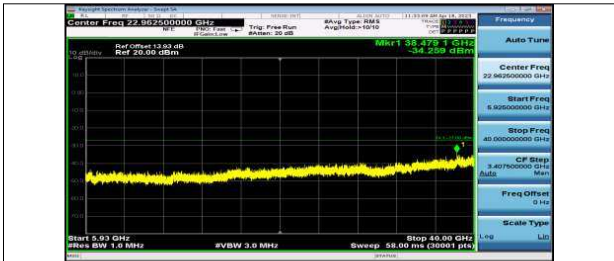
11AC40SISO_Ant1_5755_5925~40000
