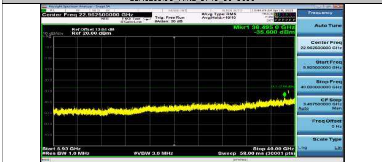
11AC20SISO_Ant1_5745_5925~40000
