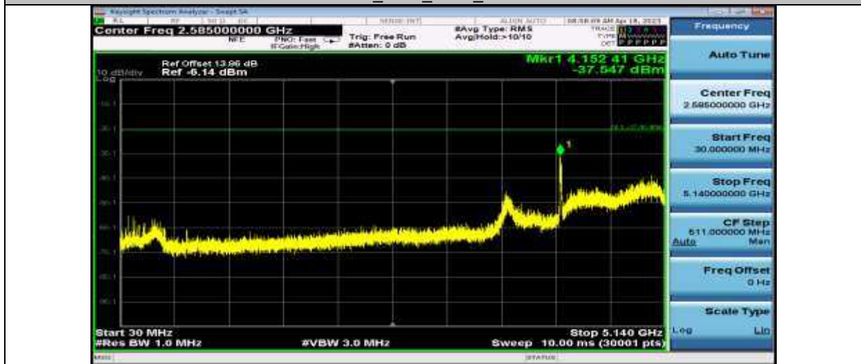
11N20SISO_Ant1_5200_30~5140
