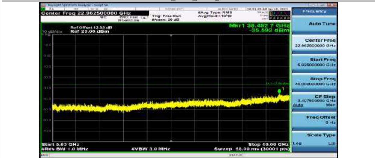
11AC20SISO_Ant1_5785_5925~40000
