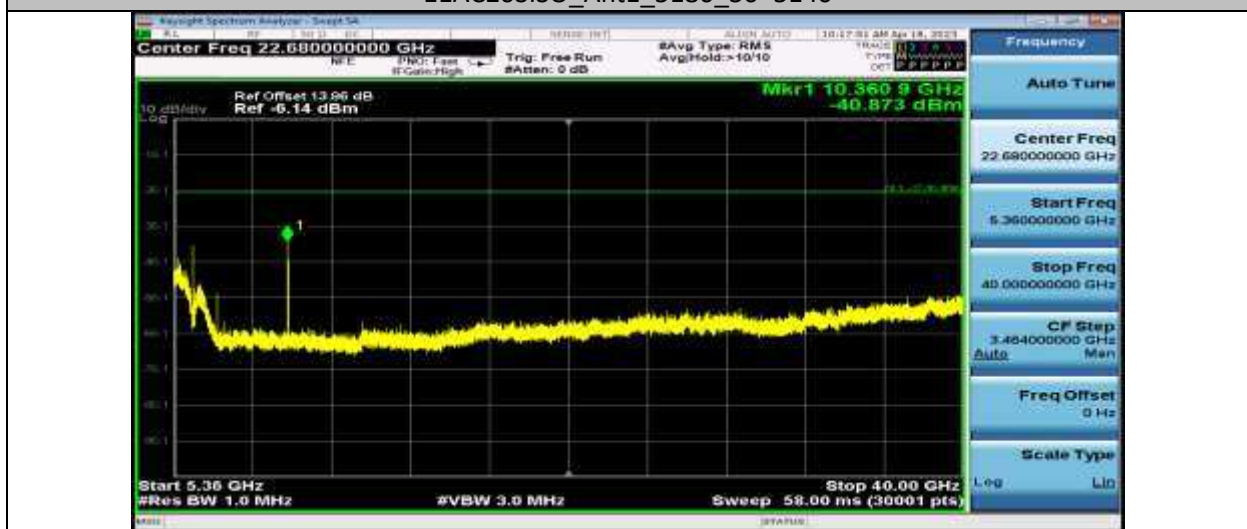
11A20SISO_Ant1_5180_5360~40000
