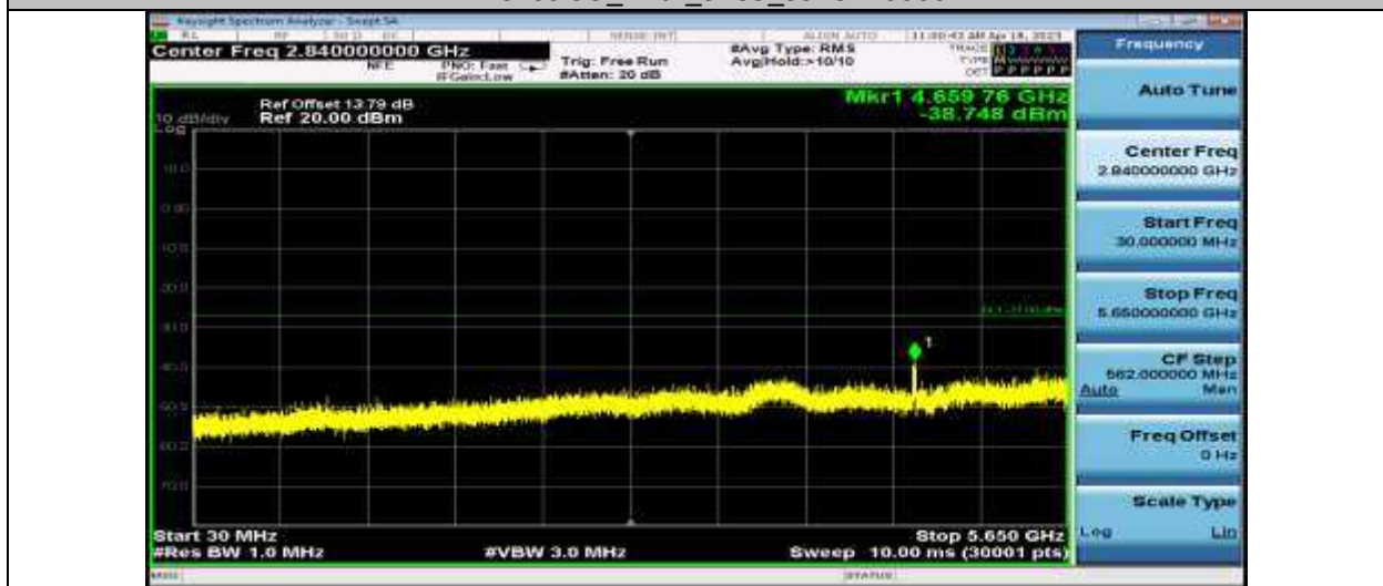
11AC20SISO_Ant1_5825_30~5650
