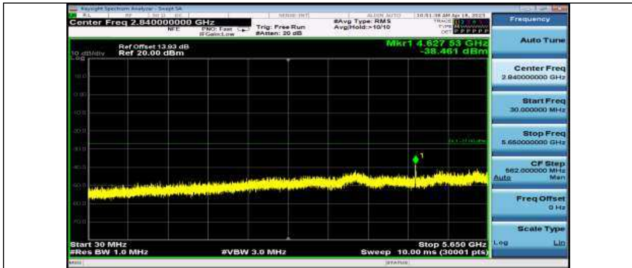
11AC20SISO_Ant1_5785_30~5650
