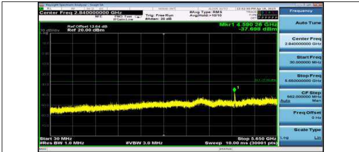
11AX20SISO_Ant1_5745_30~5650
