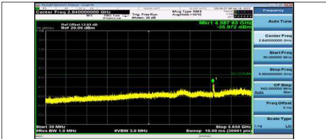
11N40SISO_Ant1_5755_30~5650
