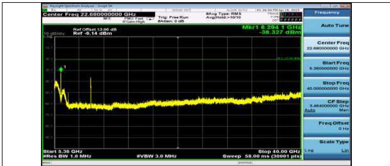
11AX40SISO_Ant1_5230_5360~40000
