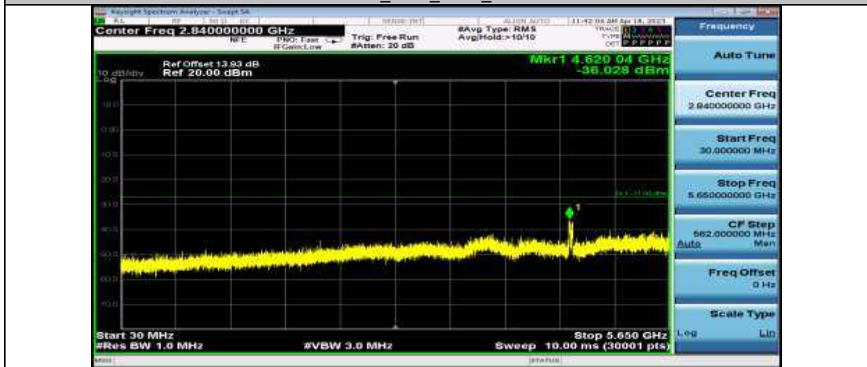
11AC40SISO_Ant1_5795_30~5650
