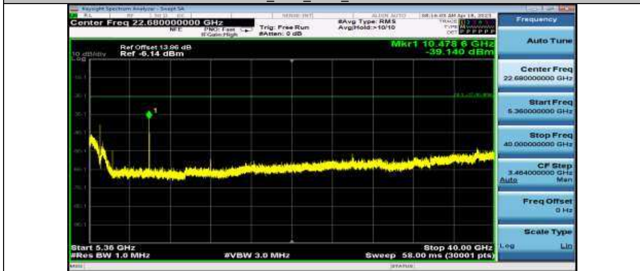
11A_Ant1_5240_5360~40000
