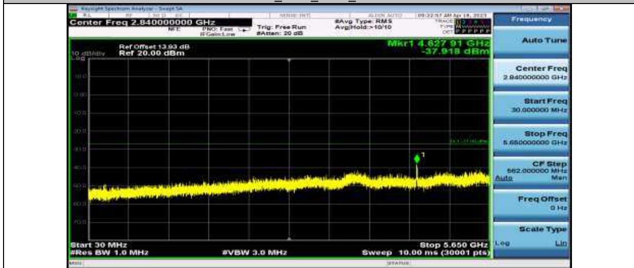
11N20SISO_Ant1_5785_30~5650
