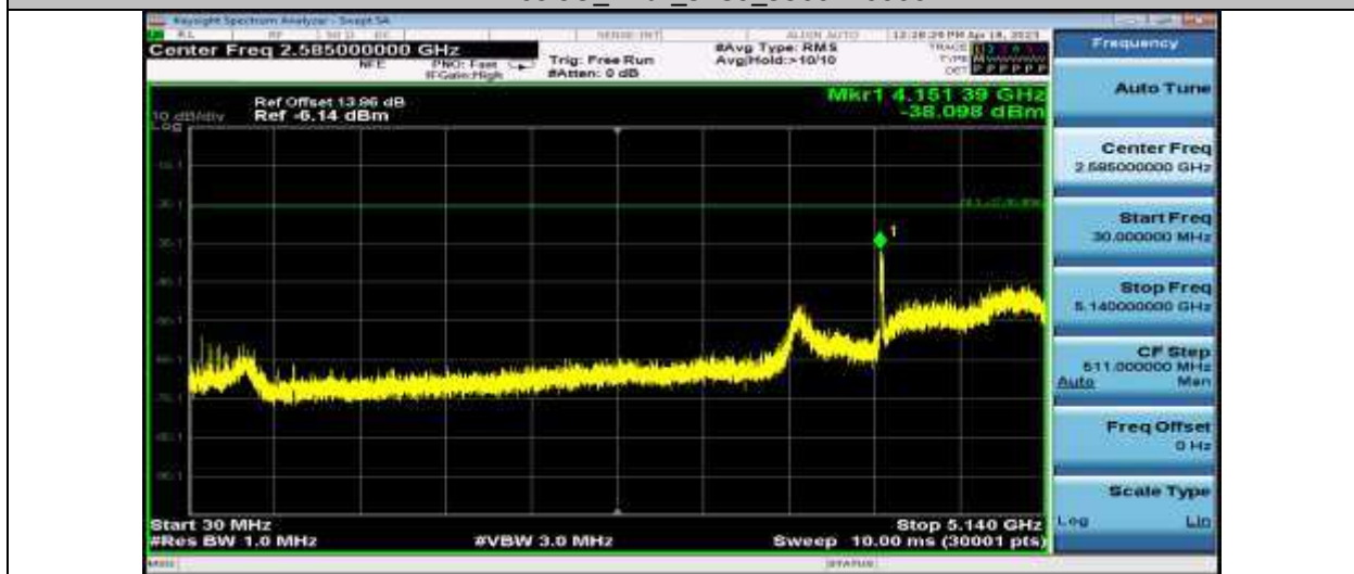
11AX20SISO_Ant1_5200_30~5140
