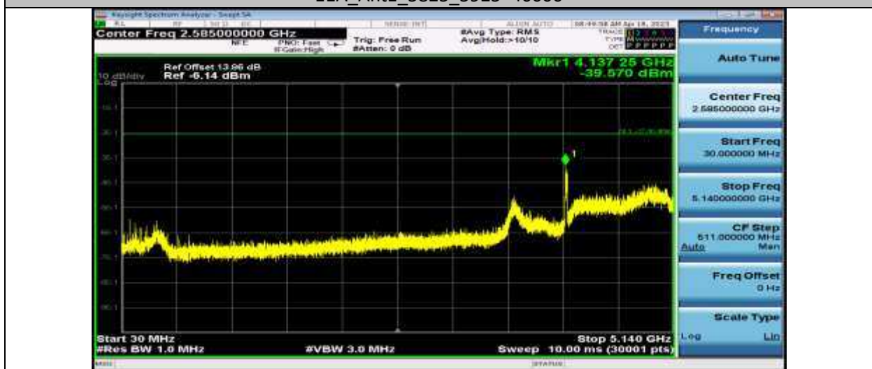
11N20SISO_Ant1_5180_30~5140
