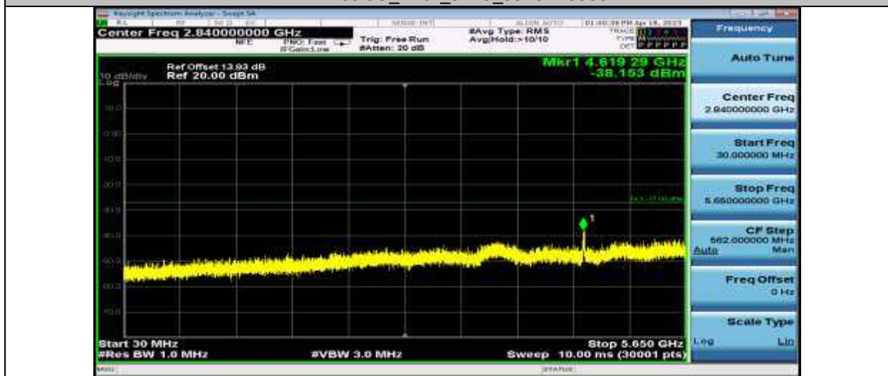
11AX20SISO_Ant1_5785_30~5650
