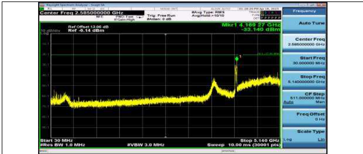
11AX40SISO_Ant1_5190_30~5140
