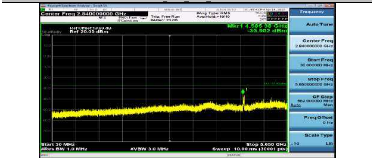
11AX40SISO_Ant1_5755_30~5650
