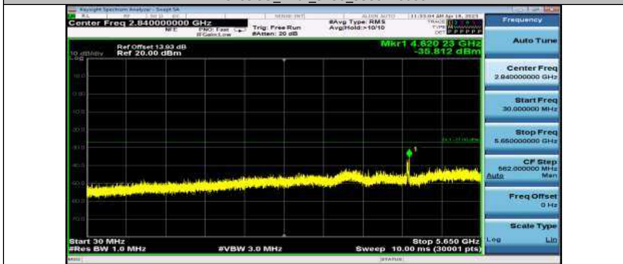
11AC40SISO_Ant1_5755_30~5650
