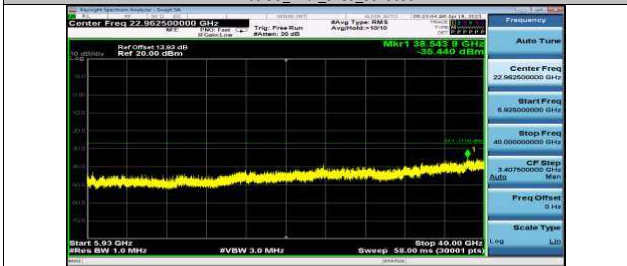
11N20SISO_Ant1_5785_5925~40000
