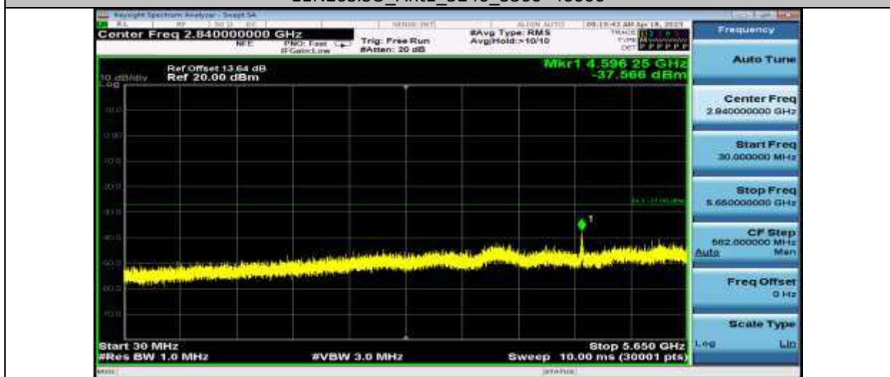
11N20SISO_Ant1_5745_30~5650
