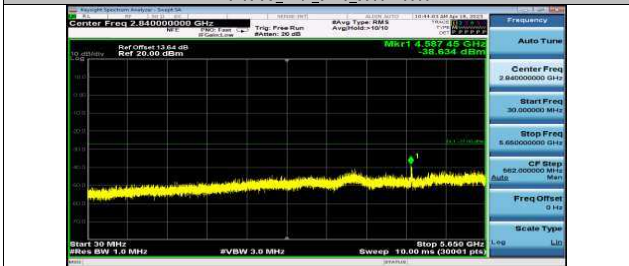
11AC20SISO_Ant1_5745_30~5650
