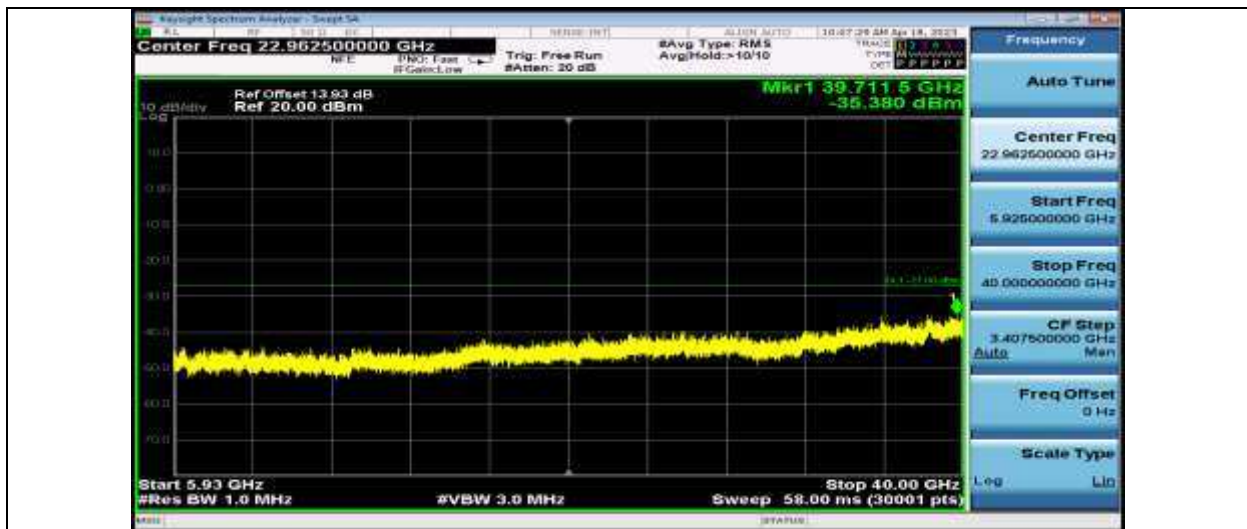
11N40SISO_Ant1_5795_5925~40000
