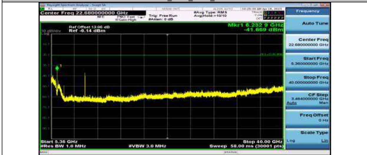
11AC20SISO_Ant1_5200_5360~40000
