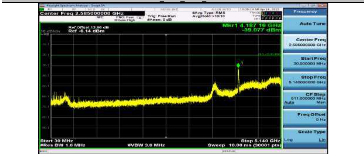
11AC20SISO_Ant1_5240_30~5140
