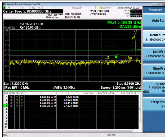
11N40SISO_Ant1_Low_5510_AV
