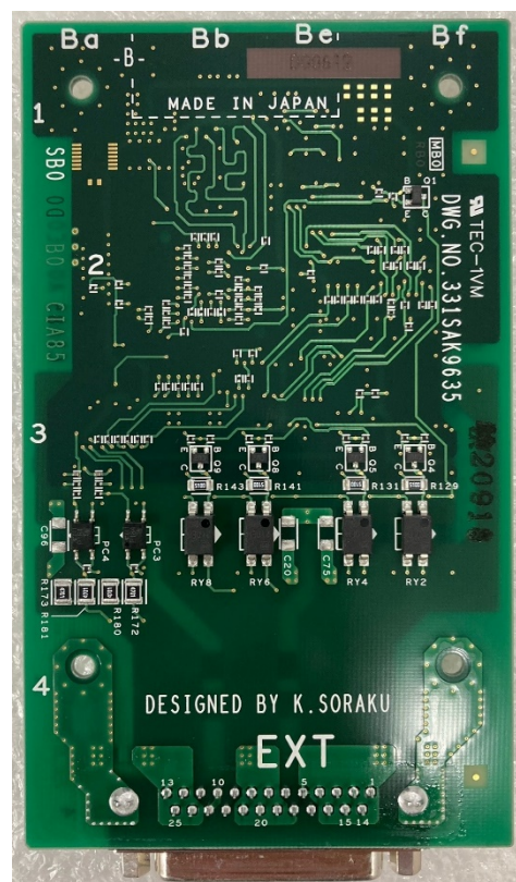
I/O bord bottom view
