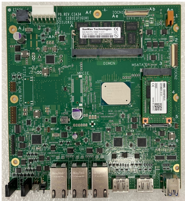
Main bord top view
