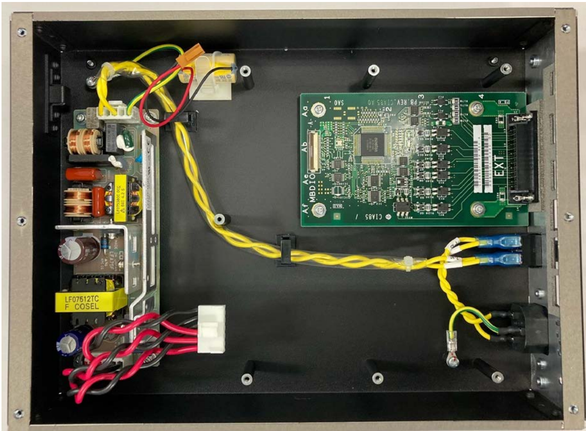
Inside view 2 with I/O board
