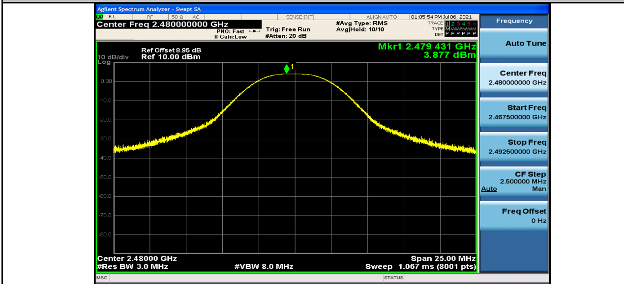
Maximum peak conducted output power_BLE_2480_2M
