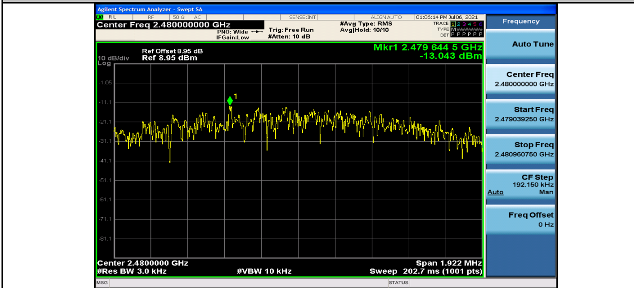
Maximum Peak power spectral density_BLE_2480_2M
