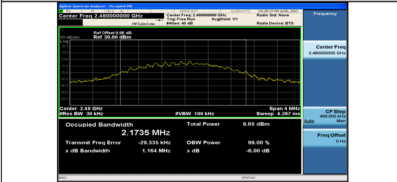
Occupied Bandwidth_BLE_2480_2M
