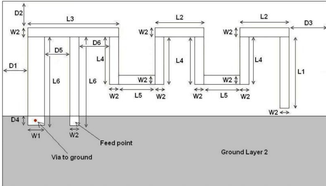
Figure 3: Antenna Dimensions
