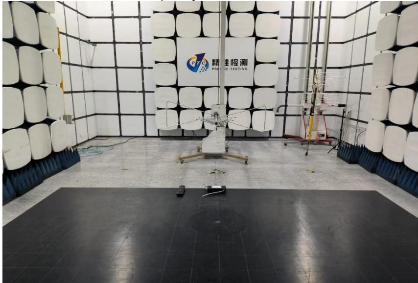
Radiated Spurious Emissions Test Frequency From Below 30MHz
