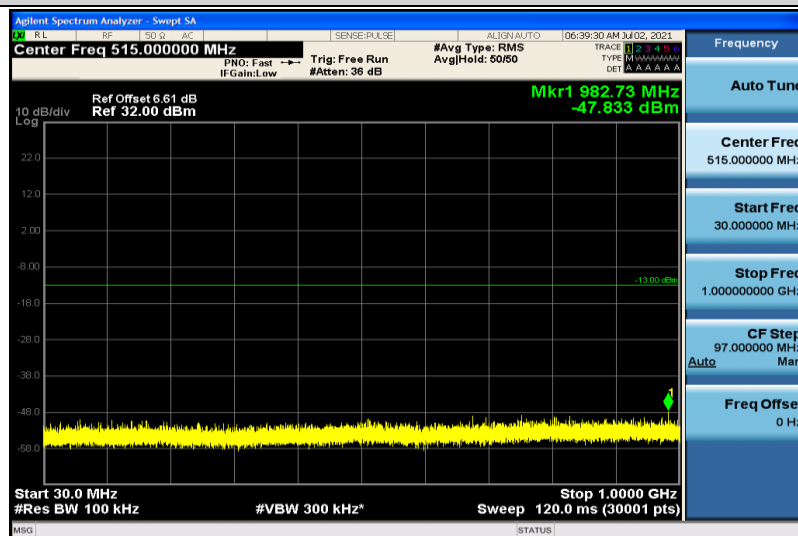
Band25-15MHz-16QAM-26615-1RB#0-30~1000MHz
