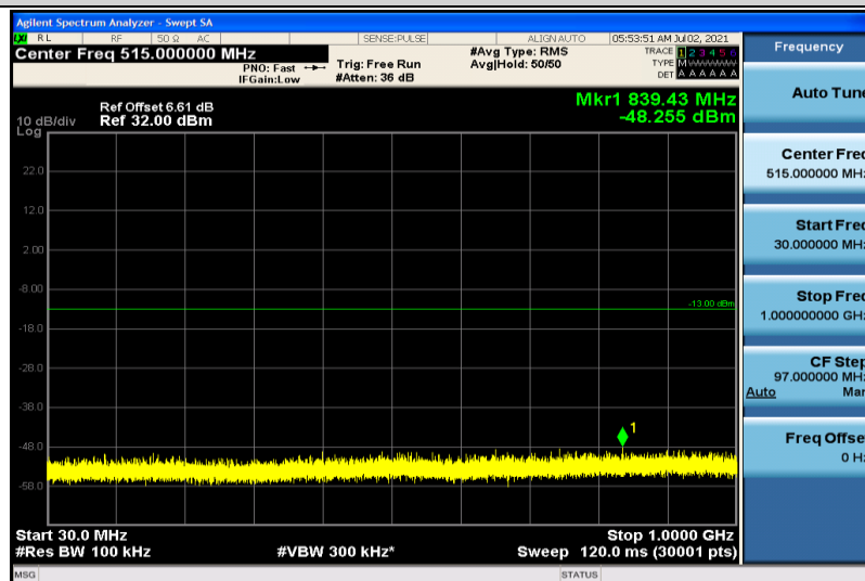
Band25-5MHz-QPSK-26665-1RB#0-30~1000MHz
