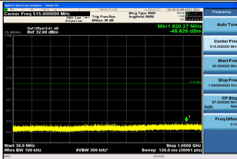
Band25-15MHz-16QAM-26365-1RB#0-30~1000MHz
