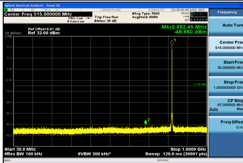
Band5-1.4MHz-QPSK-20407-1RB#0-30~1000MHz
