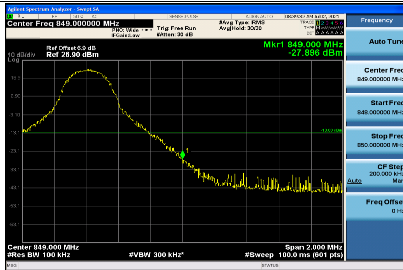
Band26-10MHz-QPSK-26990-1RB#49
