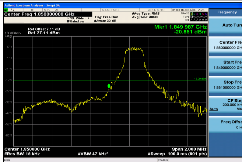
Band25-1.4MHz-QPSK-26047-1RB#0
