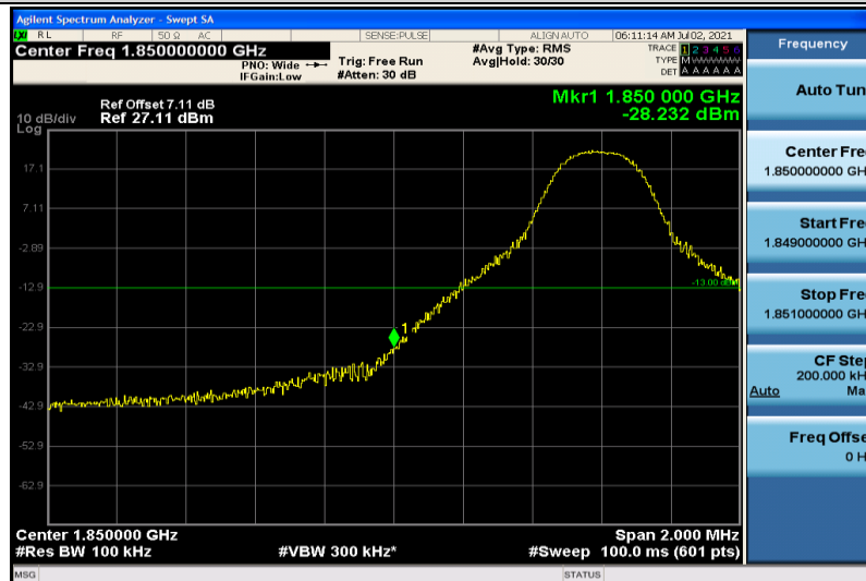
Band25-10MHz-QPSK-26090-1RB#0
