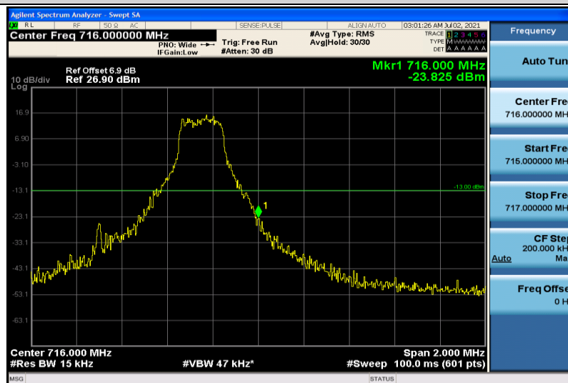
Band12-1.4MHz-16QAM-23173-1RB#5
