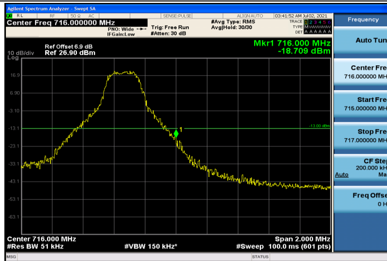
Band12-5MHz-16QAM-23155-1RB#24
