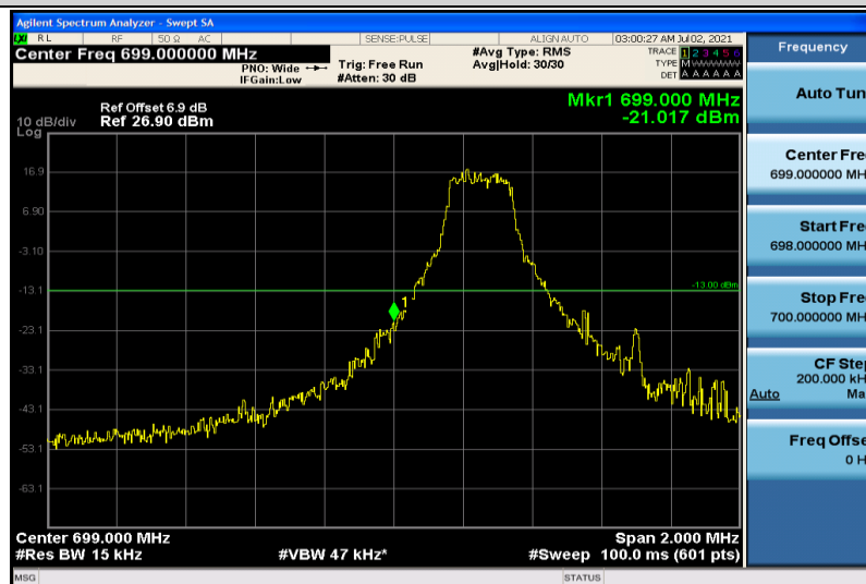
Band12-1.4MHz-QPSK-23017-1RB#0
