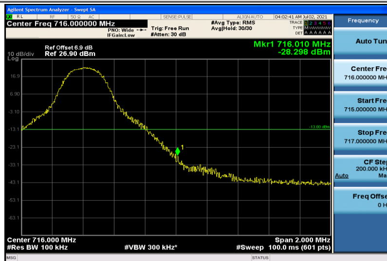
Band12-10MHz-QPSK-23130-1RB#49
