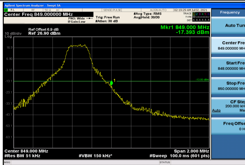
Band5-5MHz-QPSK-20625-1RB#24
