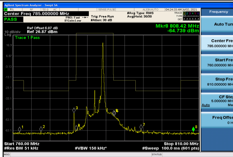
Band13-5MHz-QPSK-23230-1RB#24
