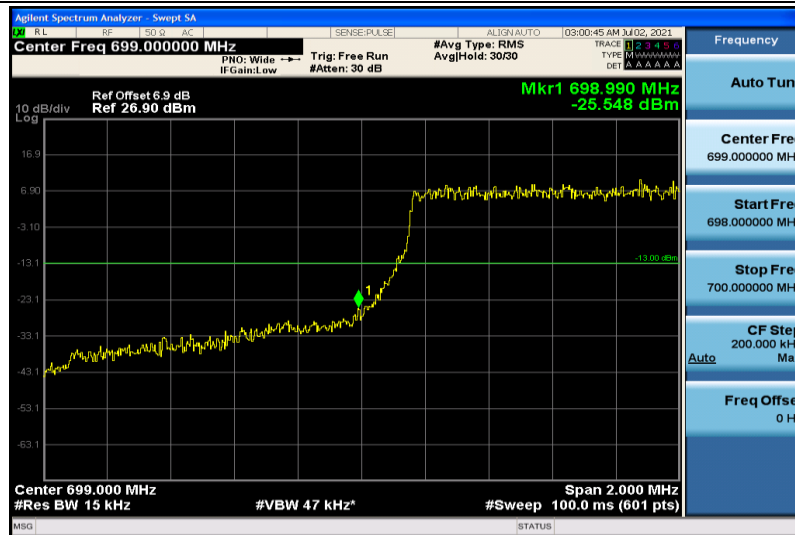
Band12-1.4MHz-QPSK-23017-6RB#0
