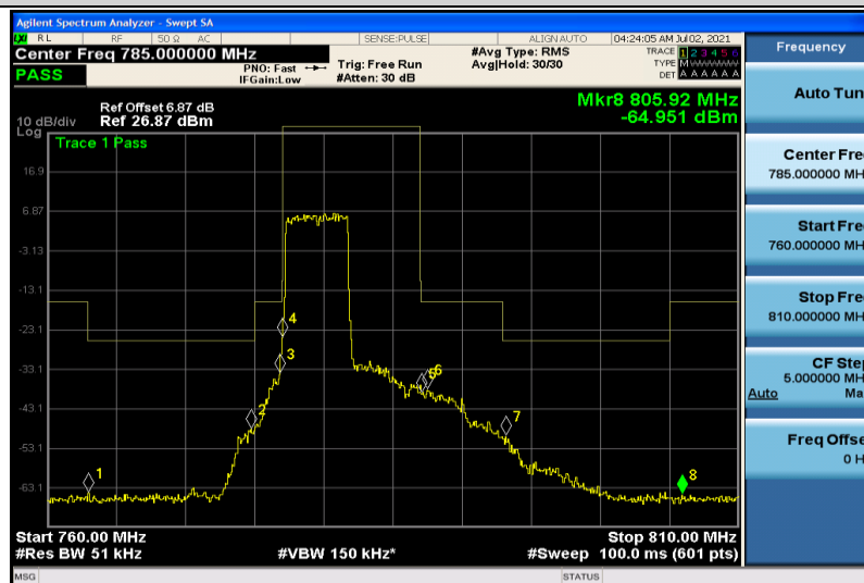
Band13-5MHz-QPSK-23205-25RB#0
