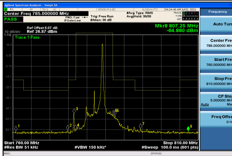
Band13-5MHz-16QAM-23230-1RB#24
