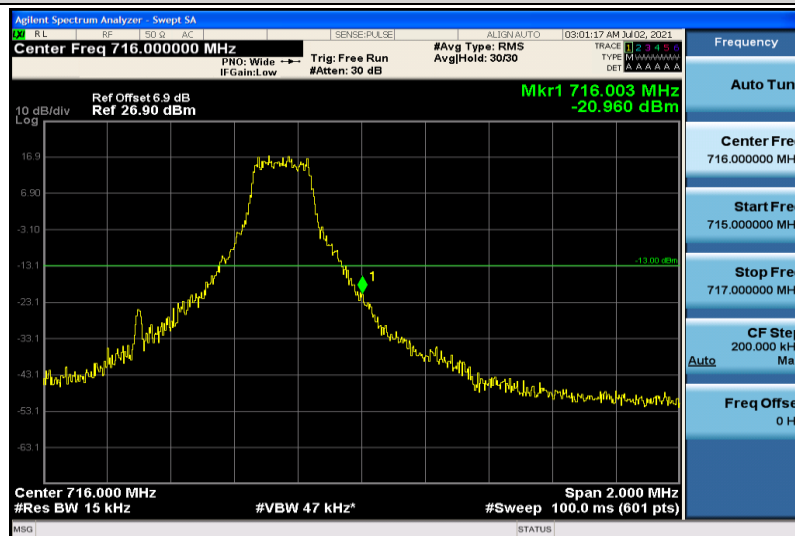
Band12-1.4MHz-QPSK-23173-1RB#5
