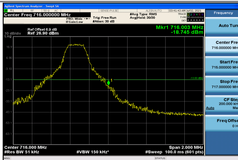
Band12-5MHz-QPSK-23155-1RB#24
