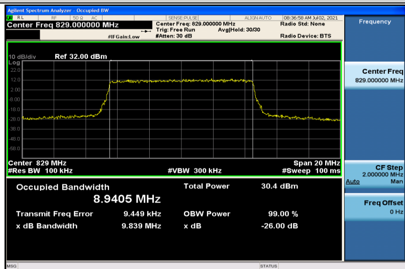
Band26-10MHz-QPSK-26840-50RB#0-8.9405
