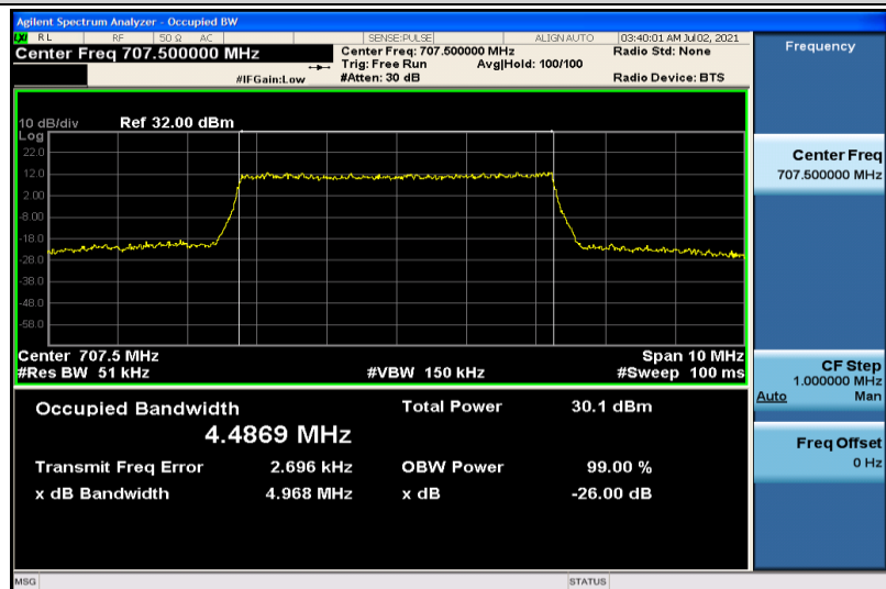
Band12-5MHz-16QAM-23095-25RB#0-4.4869
