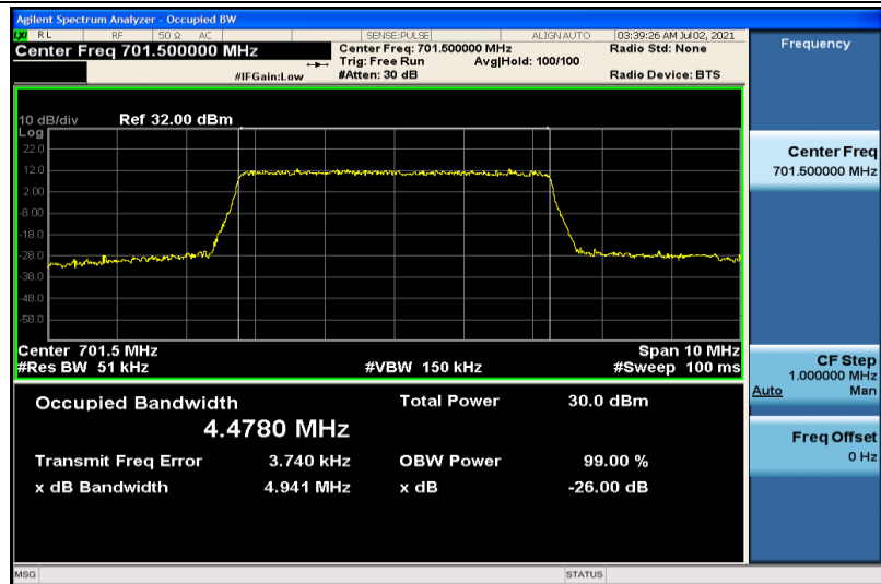
Band12-5MHz-16QAM-23035-25RB#0-4.4780
