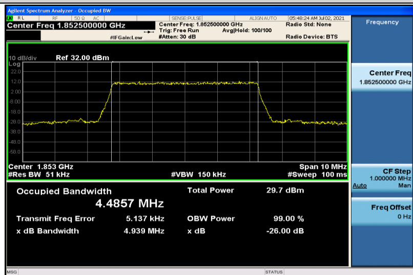
Band25-5MHz-16QAM-26065-25RB#0-4.4857
