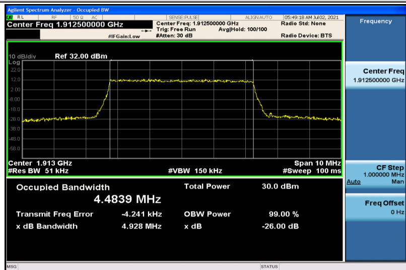
Band25-5MHz-QPSK-26665-25RB#0-4.4839
