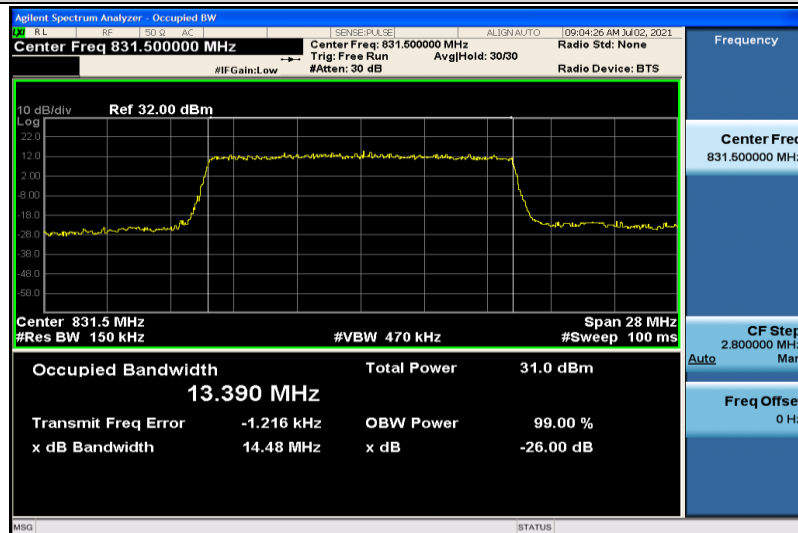
Band26-15MHz-QPSK-26865-75RB#0-13.390
