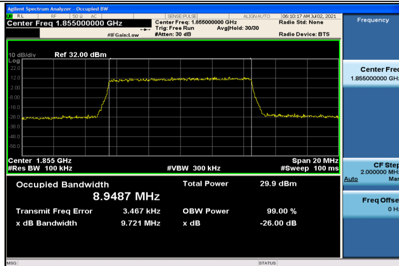
Band25-10MHz-16QAM-26090-50RB#0-8.9487
