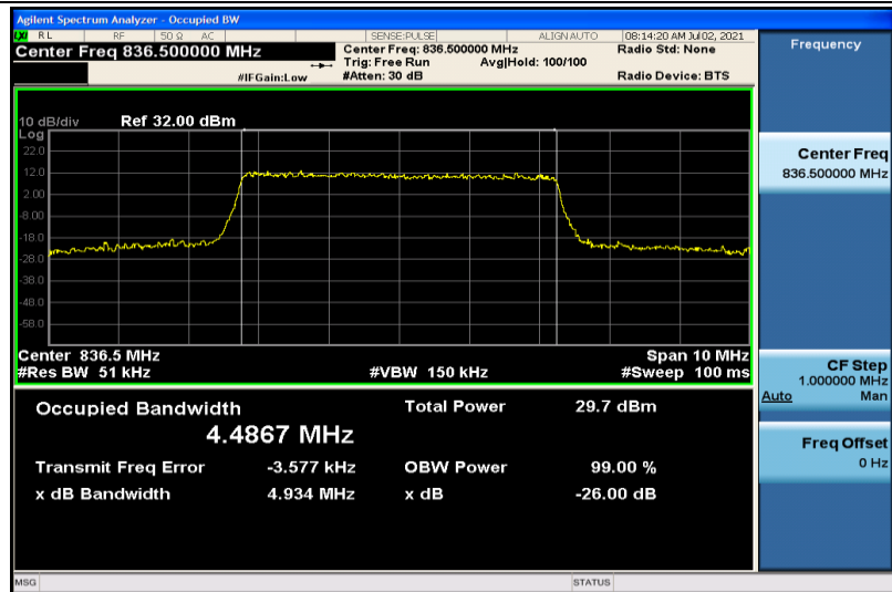
Band26-5MHz-16QAM-26915-25RB#0-4.4867
