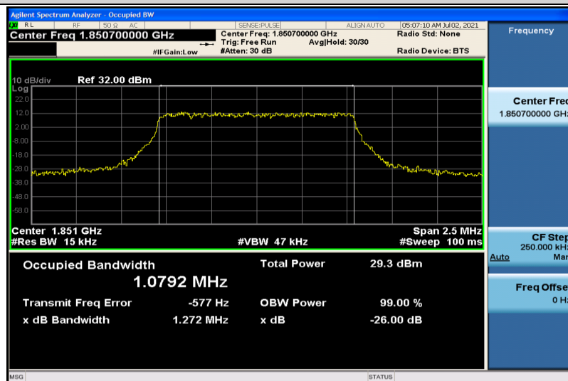
Band25-1.4MHz-QPSK-26047-6RB#0-1.0792
