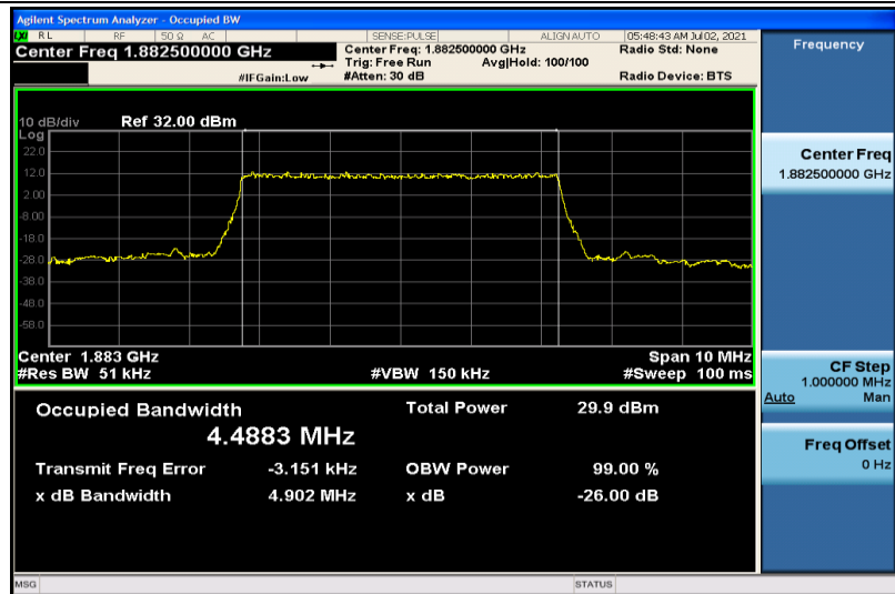
Band25-5MHz-QPSK-26365-25RB#0-4.4883
