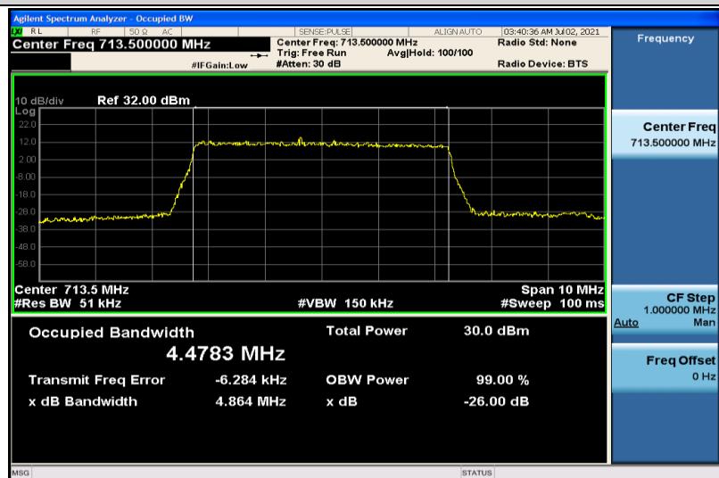
Band12-5MHz-16QAM-23155-25RB#0-4.4783
