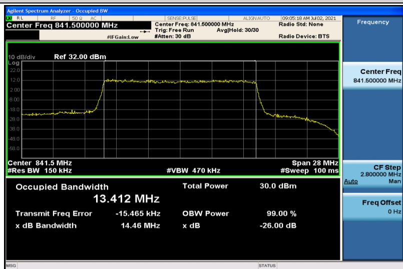
Band26-15MHz-16QAM-26965-75RB#0-13.412
