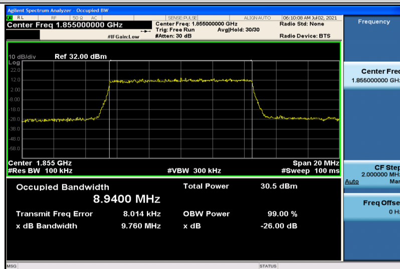
Band25-10MHz-QPSK-26090-50RB#0-8.9400
