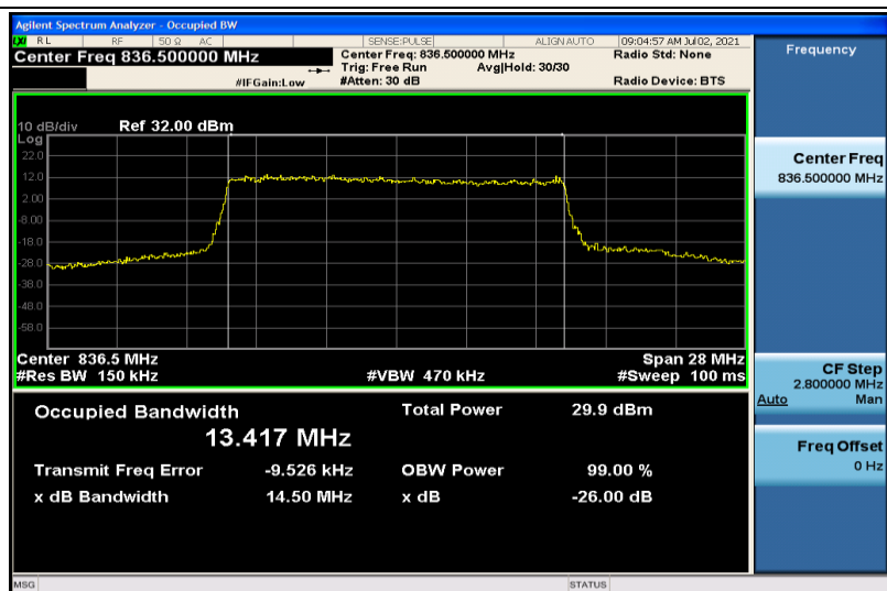
Band26-15MHz-16QAM-26915-75RB#0-13.417
