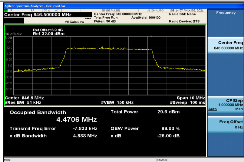
Band26-5MHz-16QAM-27015-25RB#0-4.4706
