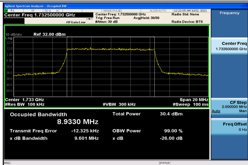
Band4-10MHz-QPSK-20175-50RB#0-8.9330
