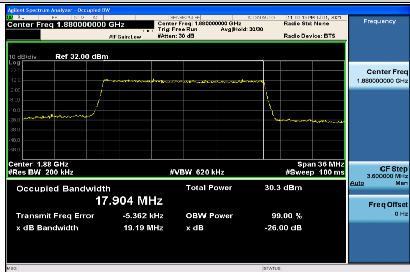
Band2-20MHz-QPSK-18900-100RB#0-17.904
