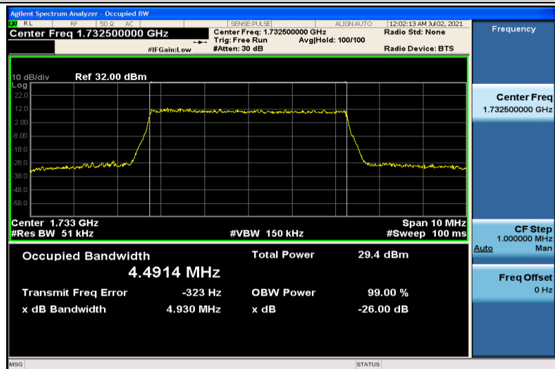
Band4-5MHz-16QAM-20175-25RB#0-4.4914
