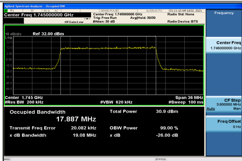
Band4-20MHz-QPSK-20300-100RB#0-17.887
