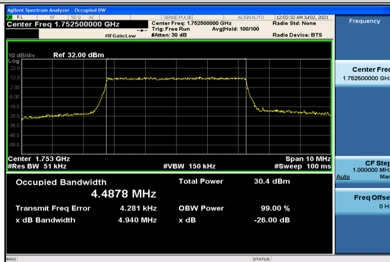
Band4-5MHz-QPSK-20375-25RB#0-4.4878
