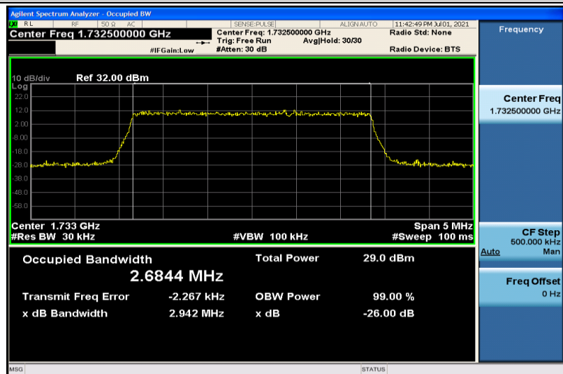
Band4-3MHz-16QAM-20175-15RB#0-2.6844
