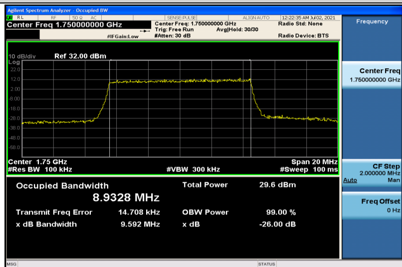
Band4-10MHz-16QAM-20350-50RB#0-8.9328
