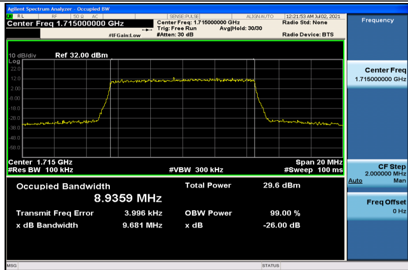
Band4-10MHz-16QAM-20000-50RB#0-8.9359
