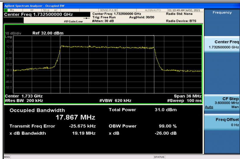
Band4-20MHz-QPSK-20175-100RB#0-17.867
