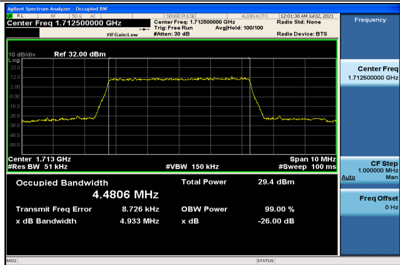
Band4-5MHz-16QAM-19975-25RB#0-4.4806
