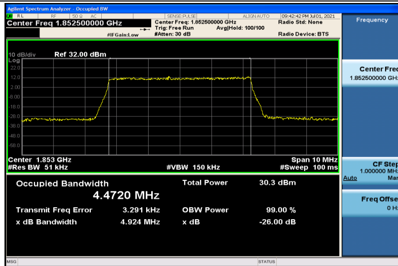
Band2-5MHz-QPSK-18625-25RB#0-4.4720
