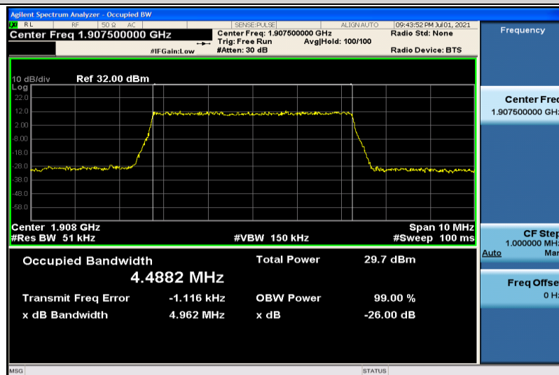
Band2-5MHz-QPSK-19175-25RB#0-4.4882
