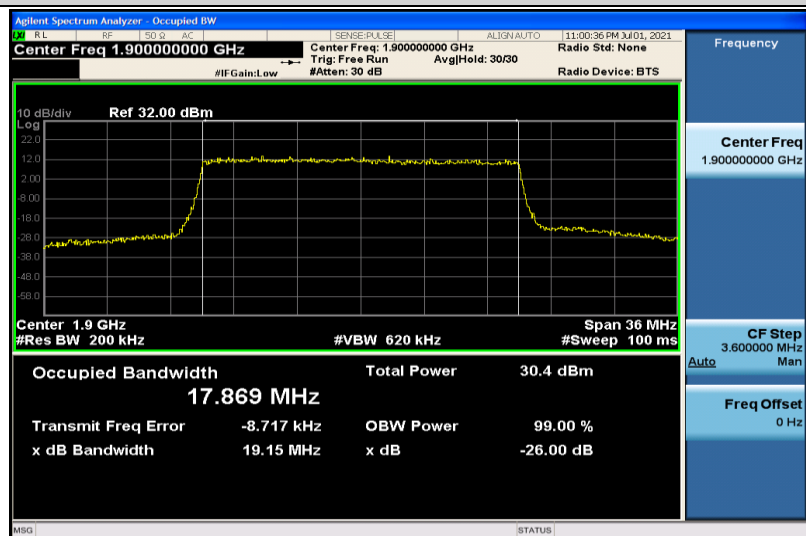
Band2-20MHz-QPSK-19100-100RB#0-17.869
