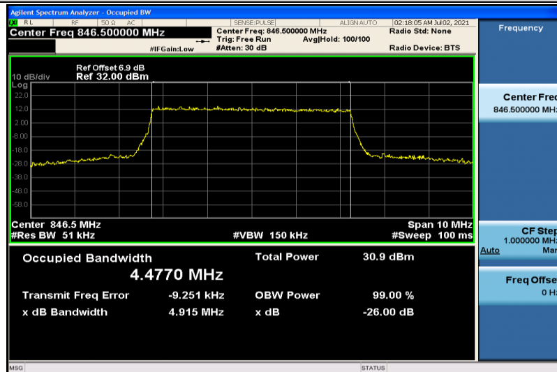
Band5-5MHz-QPSK-20625-25RB#0-4.4770
