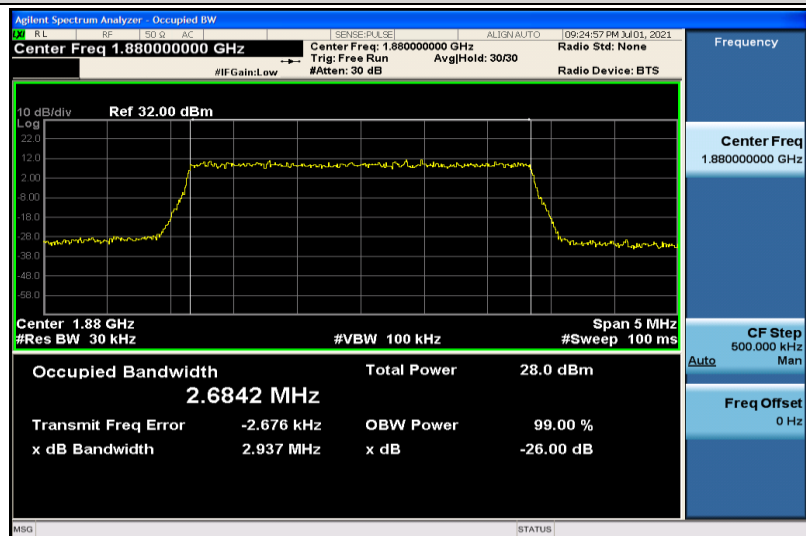
Band2-3MHz-16QAM-18900-15RB#0-2.6842
