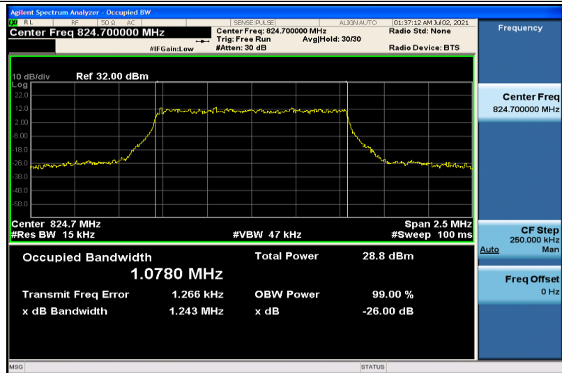
Band5-1.4MHz-16QAM-20407-6RB#0-1.0780
