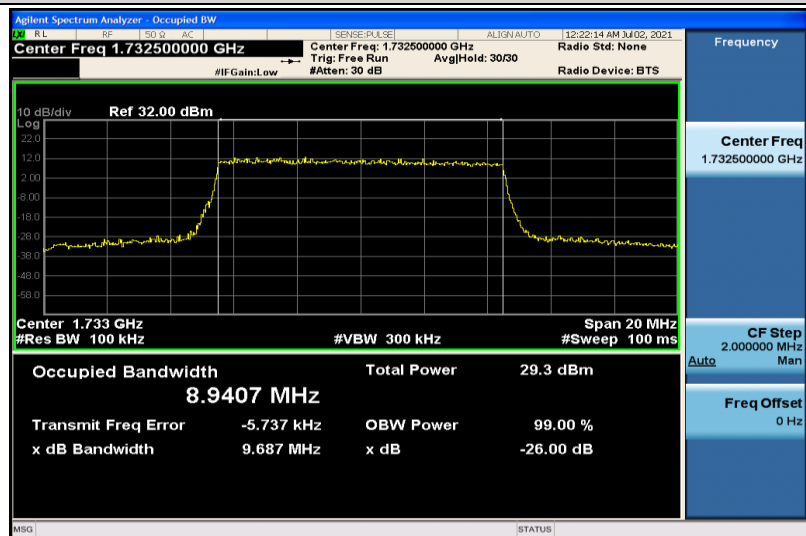
Band4-10MHz-16QAM-20175-50RB#0-8.9407
