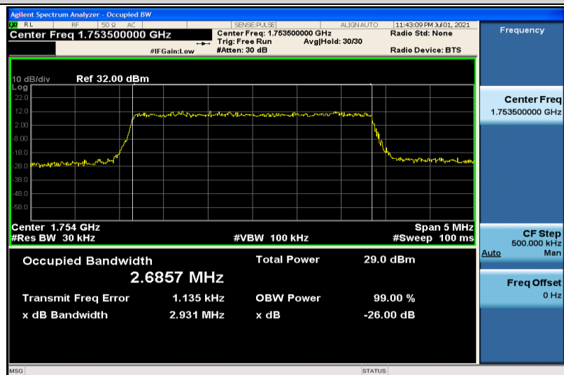
Band4-3MHz-16QAM-20385-15RB#0-2.6857
