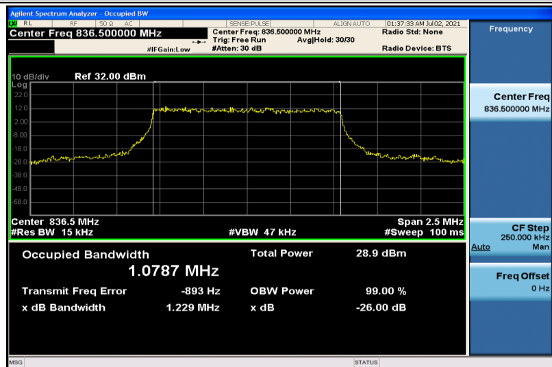
Band5-1.4MHz-16QAM-20525-6RB#0-1.0787
