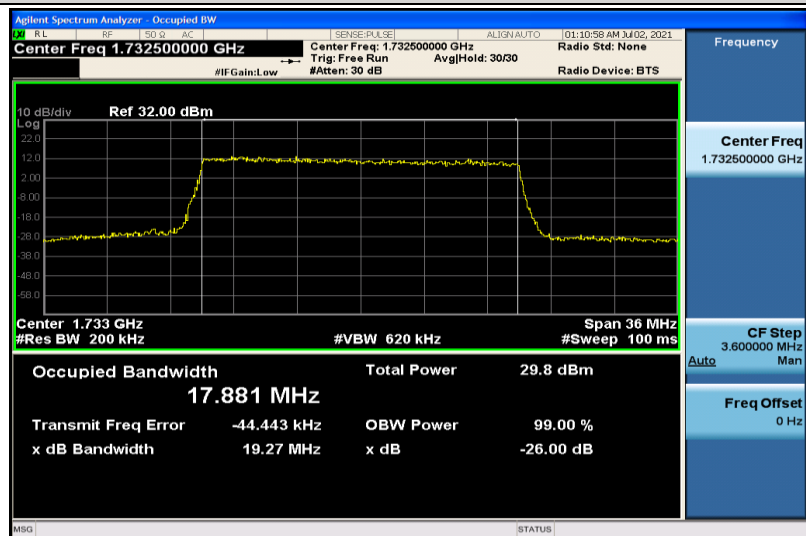
Band4-20MHz-16QAM-20175-100RB#0-17.881
