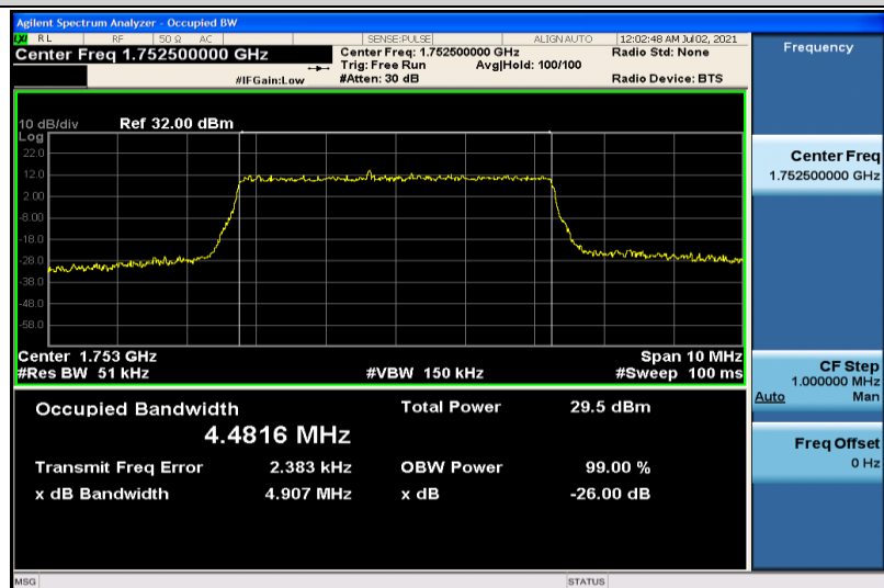
Band4-5MHz-16QAM-20375-25RB#0-4.4816
