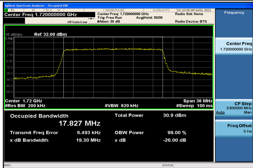
Band4-20MHz-QPSK-20050-100RB#0-17.827
