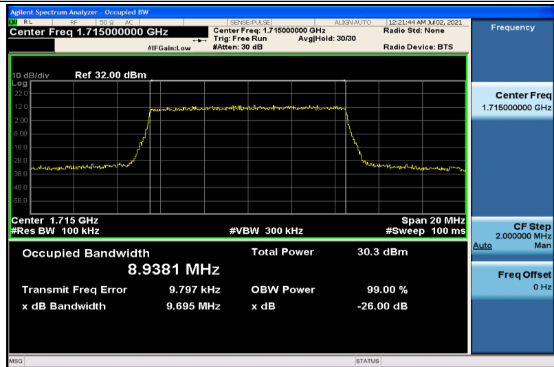
Band4-10MHz-QPSK-20000-50RB#0-8.9381
