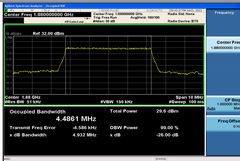
Band2-5MHz-QPSK-18900-25RB#0-4.4861
