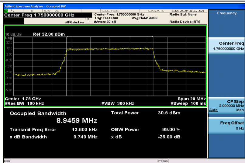
Band4-10MHz-QPSK-20350-50RB#0-8.9459
