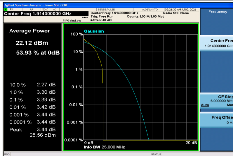
Band25-1.4MHz-QPSK-26683-1RB#0
