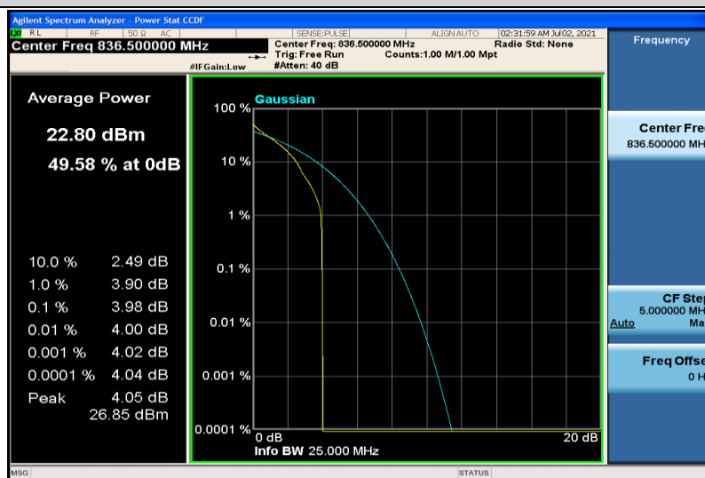
Band5-5MHz-QPSK-20525-1RB#0
