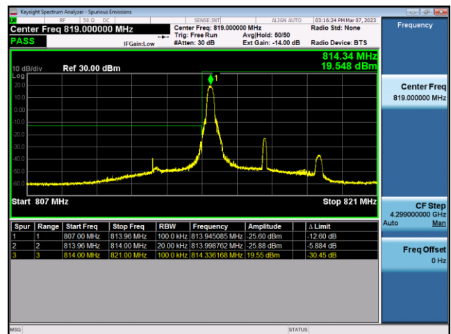
FDD26-Part 90-5MHz-16QAM-LCH-1RB#0
