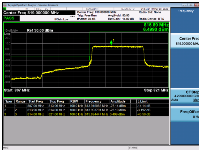
FDD26-Part 90-5MHz-QPSK-HCH-1RB#24
