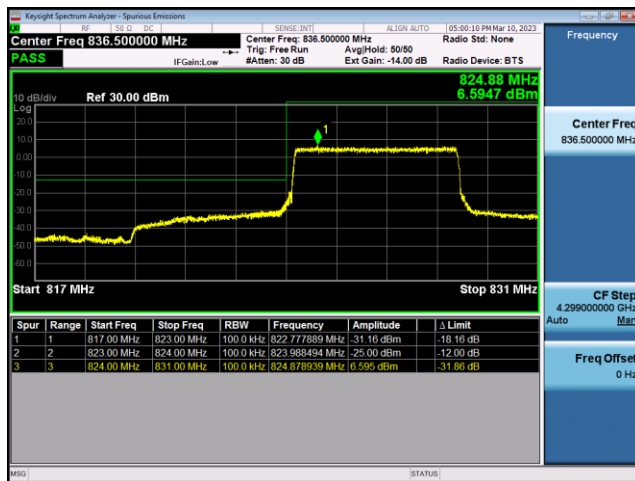
FDD26-Part 22-5MHz-QPSK-HCH-1RB#24
