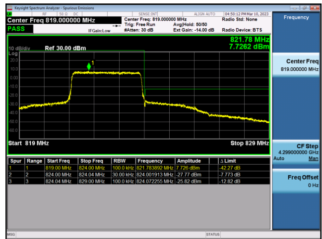
FDD26-Part 90-5MHz-16QAM-LCH-1RB#0
