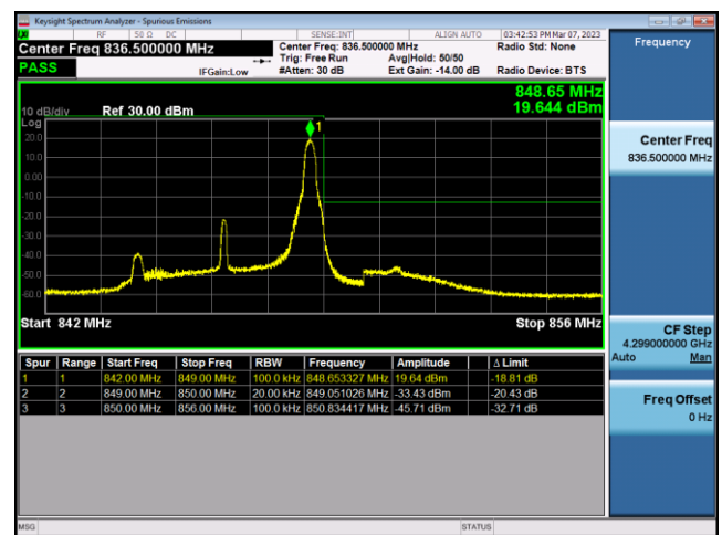
FDD26-Part 22-5MHz-16QAM-HCH-25RB#0
