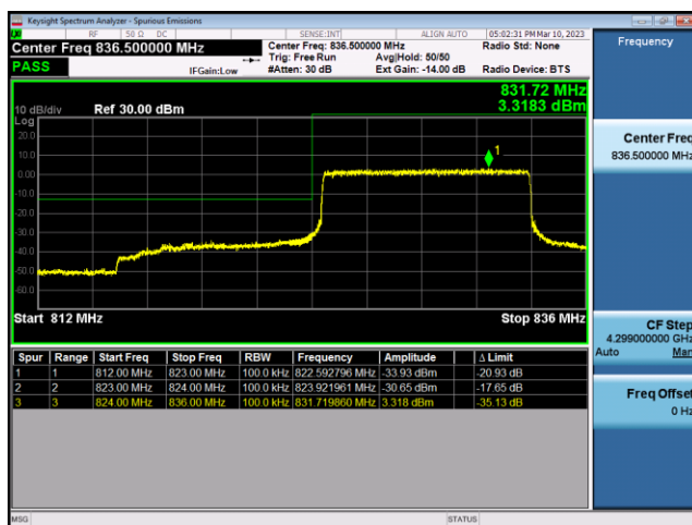
FDD26-Part 22-10MHz-QPSK-HCH-1RB#49
