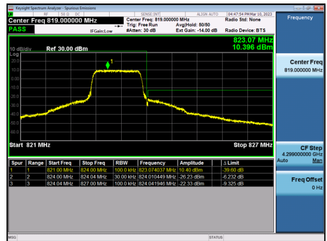
FDD26-Part 90-3MHz-16QAM-LCH-1RB#0
