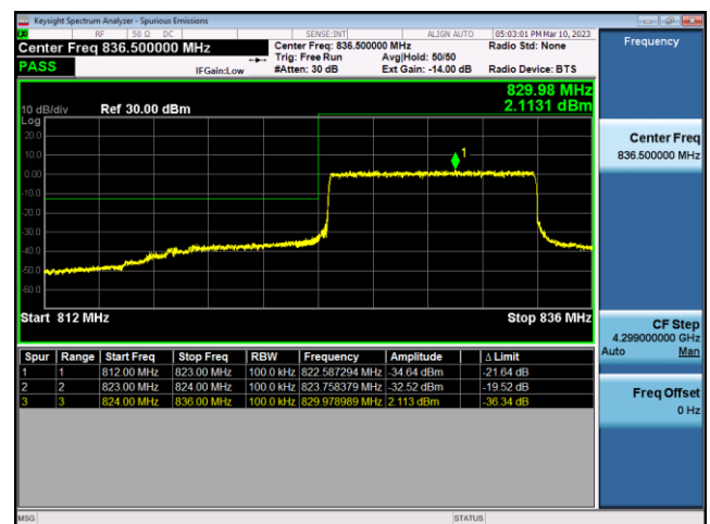
FDD26-Part 22-10MHz-16QAM-HCH-1RB#49
