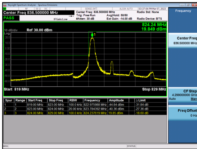
FDD26-Part 22-3MHz-QPSK-LCH-15RB#0
