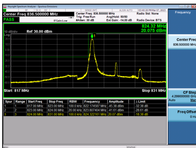
FDD26-Part 22-5MHz-QPSK-LCH-1RB#0
