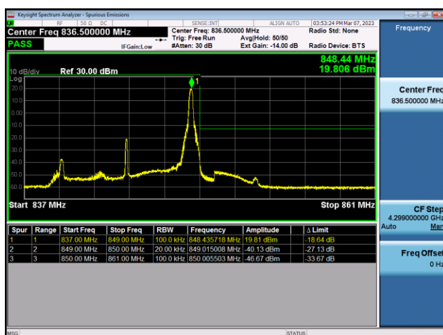
FDD26-Part 22-10MHz-QPSK-HCH-1RB#49
