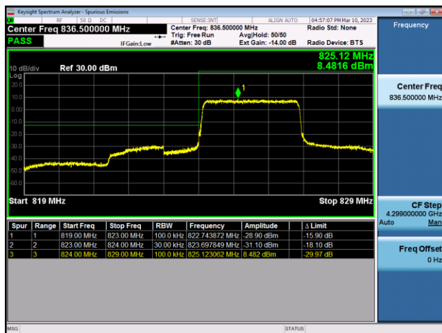
FDD26-Part 22-3MHz-QPSK-LCH-15RB#0
