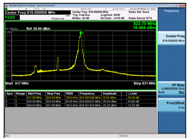
FDD26-Part 90-5MHz-16QAM-HCH-25RB#0
