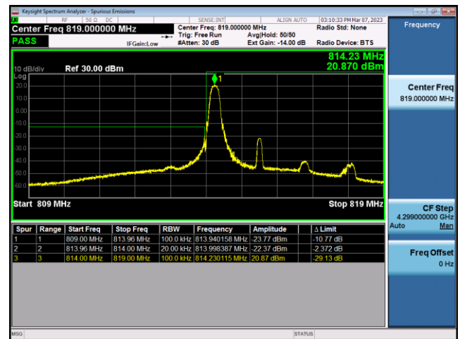
FDD26-Part 90-3MHz-16QAM-LCH-15RB#0
