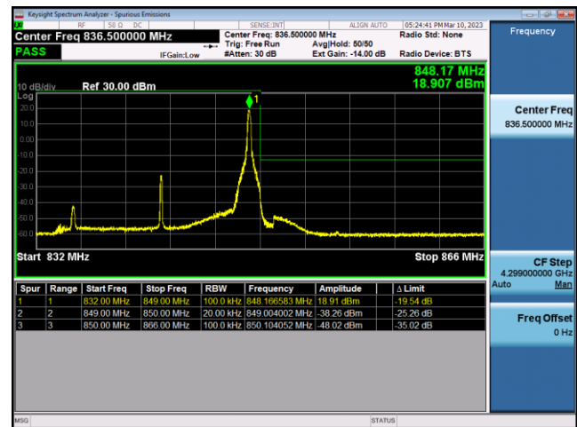
FDD26-Part 22-15MHz-16QAM-HCH-75RB#0
