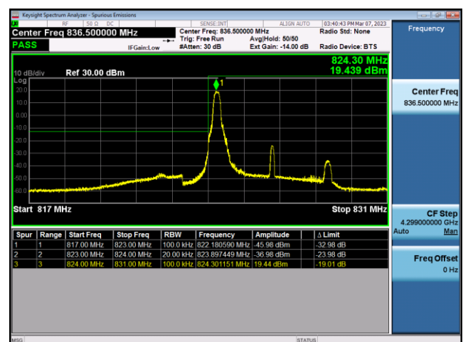
FDD26-Part 22-5MHz-16QAM-LCH-1RB#0
