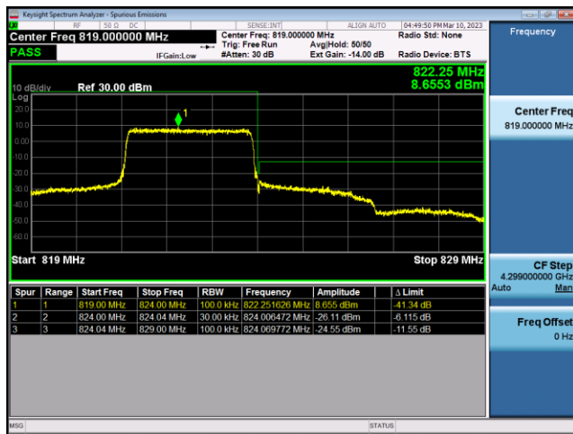
FDD26-Part 90-5MHz-QPSK-LCH-1RB#0
