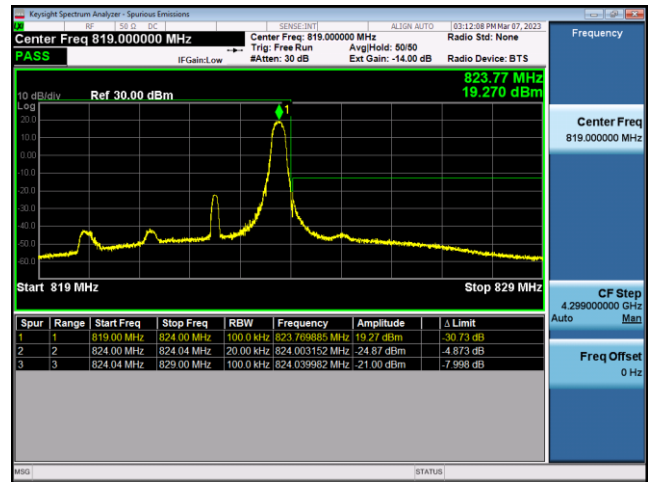
FDD26-Part 90-3MHz-16QAM-HCH-15RB#0
