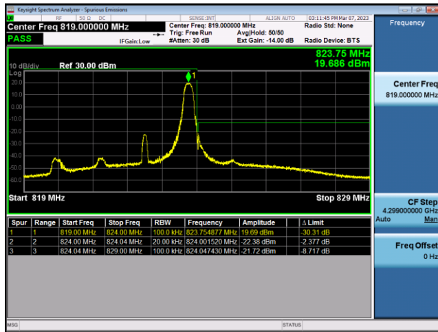
FDD26-Part 90-3MHz-QPSK-HCH-15RB#0
