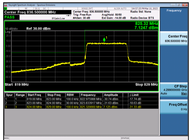
FDD26-Part 22-3MHz-16QAM-LCH-15RB#0
