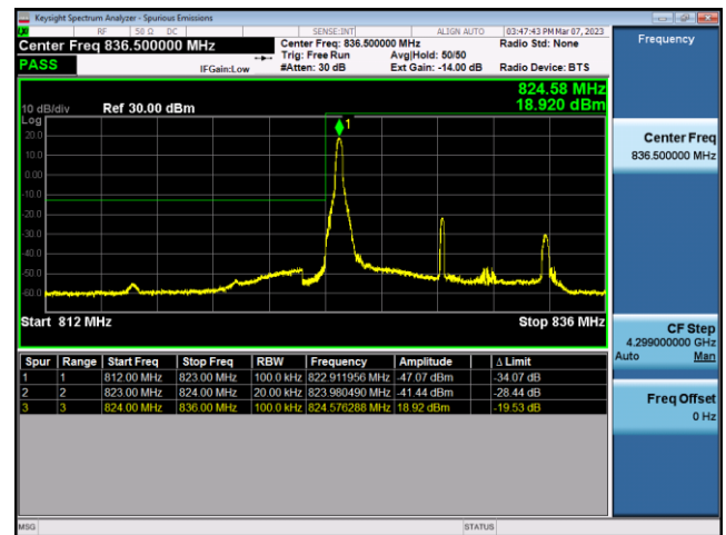
FDD26-Part 22-10MHz-16QAM-LCH-50RB#0
