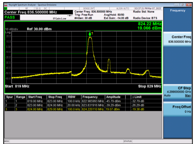
FDD26-Part 22-3MHz-16QAM-LCH-15RB#0
