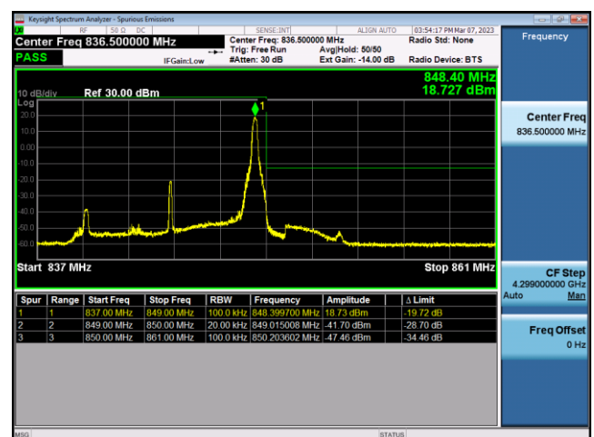
FDD26-Part 22-10MHz-16QAM-HCH-1RB#49
