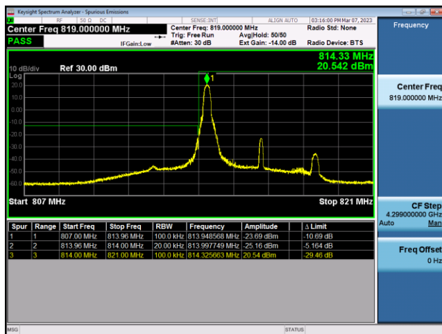
FDD26-Part 90-5MHz-QPSK-LCH-1RB#0
