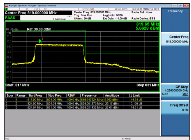
FDD26-Part 90-5MHz-16QAM-HCH-25RB#0
