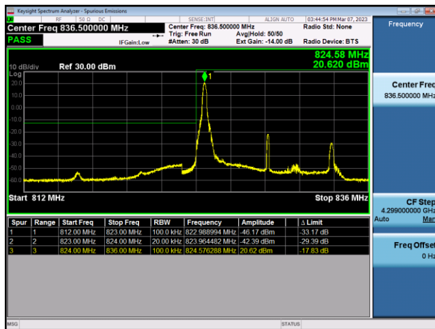
FDD26-Part 22-10MHz-QPSK-LCH-50RB#0
