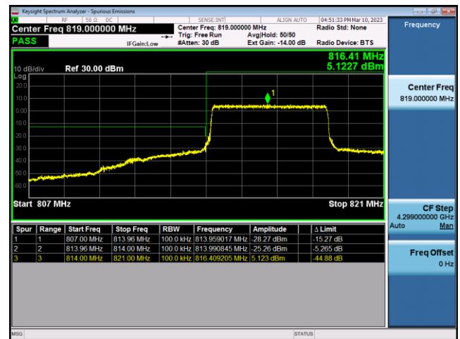
FDD26-Part 90-5MHz-16QAM-HCH-1RB#24
