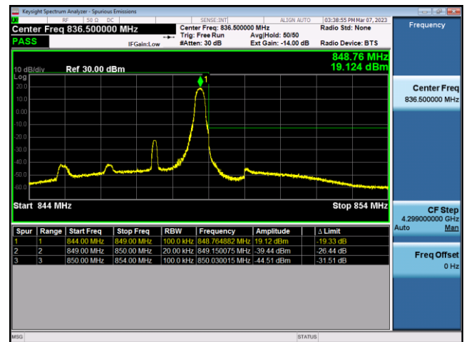
FDD26-Part 22-3MHz-16QAM-HCH-15RB#0
