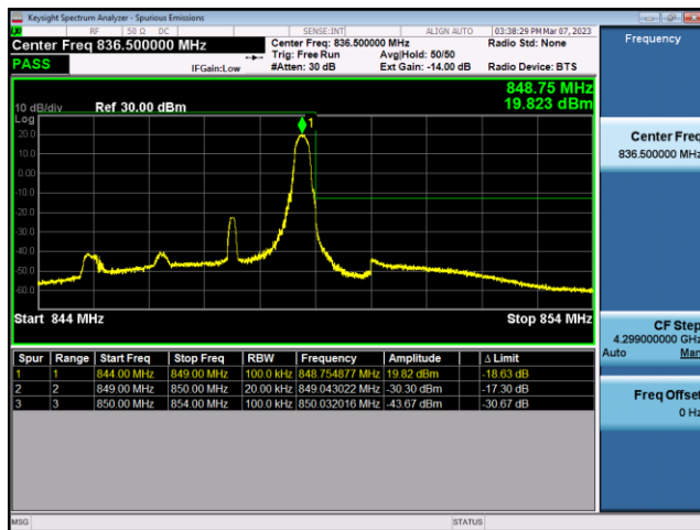
FDD26-Part 22-3MHz-QPSK-HCH-15RB#0
