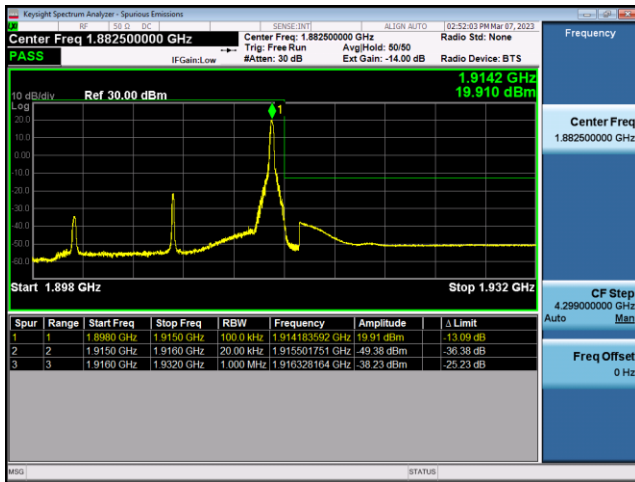
FDD25-15MHz-QPSK-HCH-75RB#0
