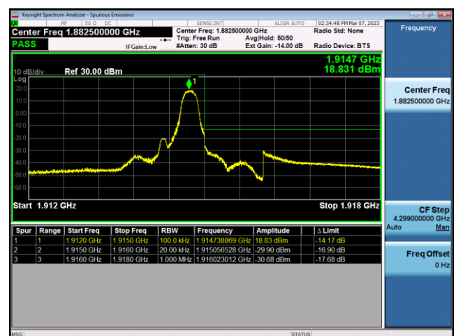
FDD25-1.4MHz-16QAM-HCH-1RB#5
