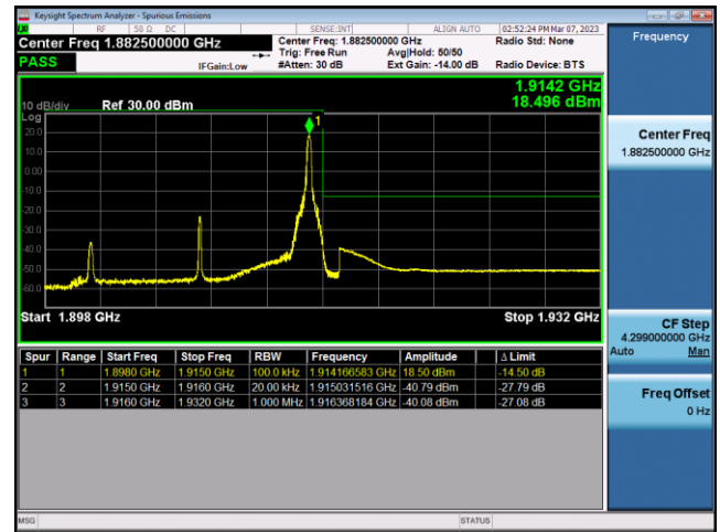
FDD25-15MHz-16QAM-HCH-75RB#0
