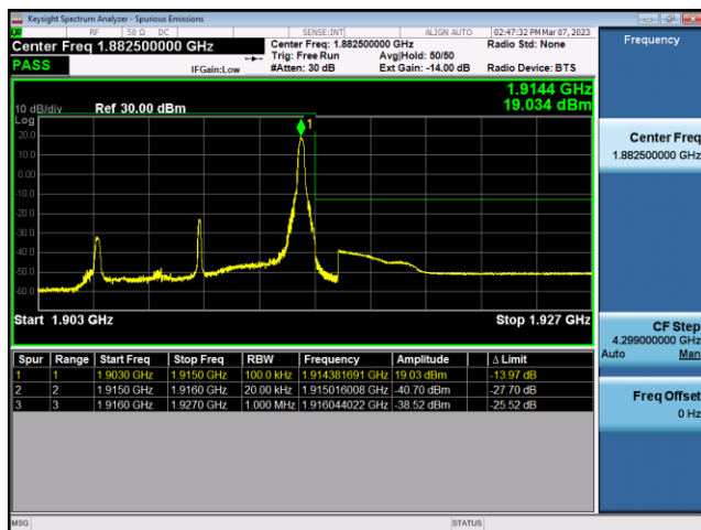
FDD25-10MHz-QPSK-HCH-1RB#49
