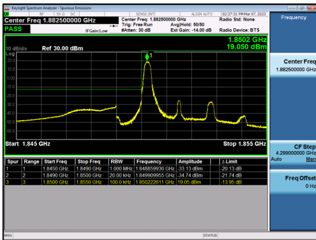
FDD25-3MHz-QPSK-LCH-15RB#0
