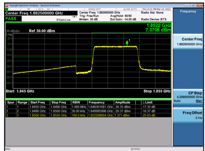
FDD25-3MHz-16QAM-LCH-15RB#0
