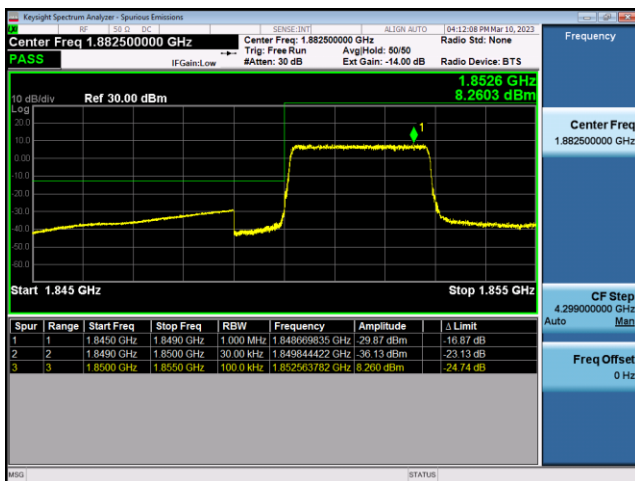
FDD25-3MHz-QPSK-LCH-15RB#0
