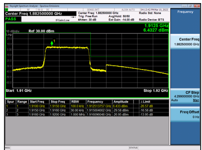
FDD25-5MHz-16QAM-LCH-1RB#0
