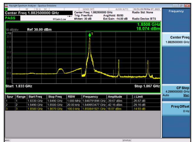
FDD25-15MHz-16QAM-LCH-75RB#0
