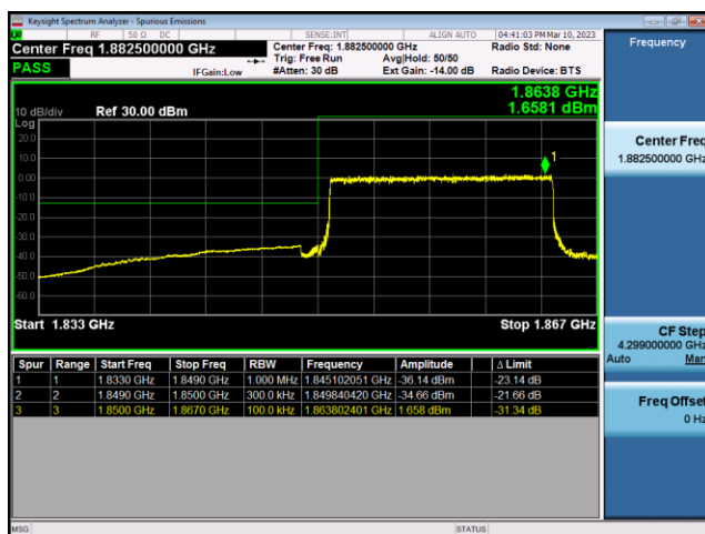
FDD25-15MHz-QPSK-LCH-75RB#0
