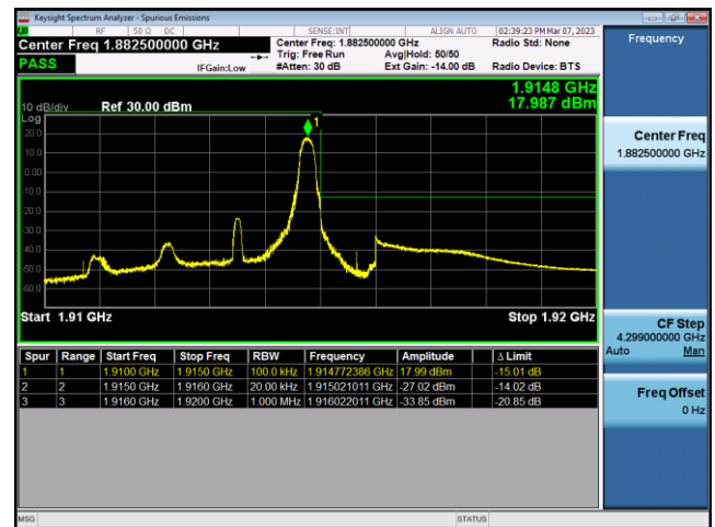
FDD25-3MHz-16QAM-HCH-15RB#0
