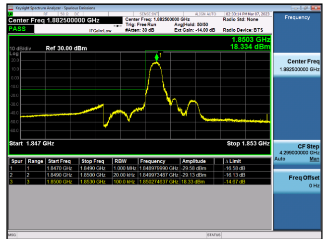
FDD25-1.4MHz-16QAM-LCH-6RB#0
