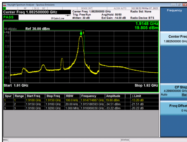
FDD25-3MHz-QPSK-HCH-15RB#0
