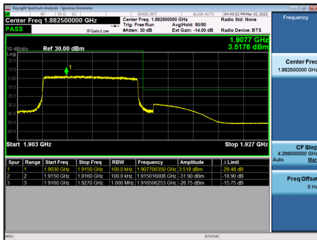
FDD25-15MHz-QPSK-LCH-1RB#0
