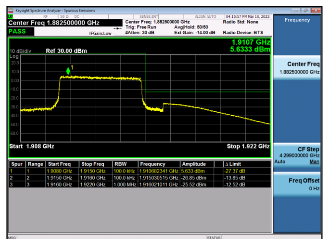
FDD25-5MHz-16QAM-HCH-25RB#0
