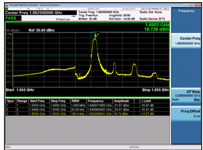
FDD25-3MHz-16QAM-LCH-15RB#0
