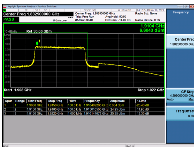
FDD25-5MHz-QPSK-HCH-25RB#0
