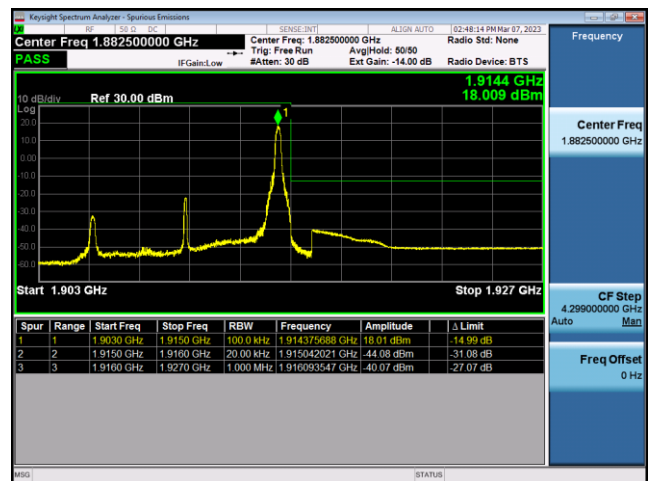
FDD25-10MHz-16QAM-HCH-1RB#49
