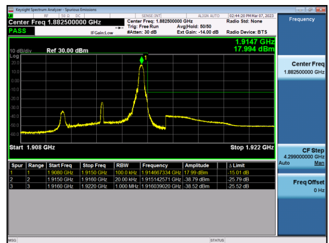
FDD25-5MHz-16QAM-HCH-25RB#0
