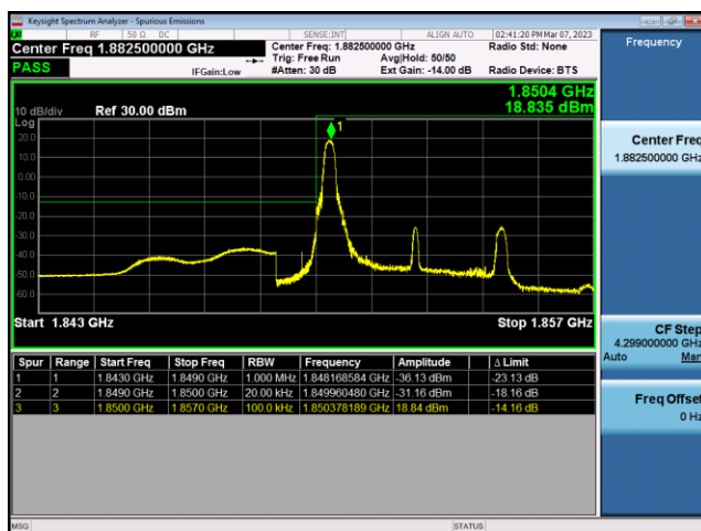
FDD25-5MHz-QPSK-LCH-1RB#0
