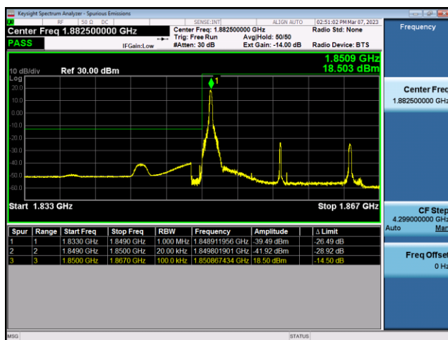
FDD25-15MHz-QPSK-LCH-75RB#0
