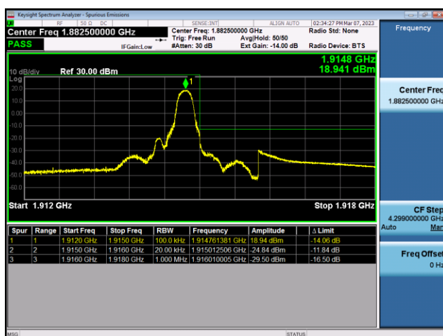
FDD25-1.4MHz-QPSK-HCH-1RB#5
