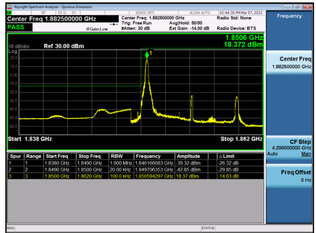
FDD25-10MHz-16QAM-LCH-50RB#0
