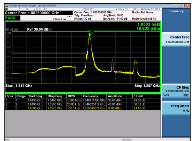
FDD25-5MHz-16QAM-LCH-1RB#0
