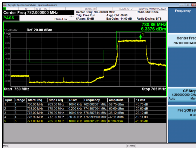
FDD13-5MHz-QPSK-HCH-1RB#24
