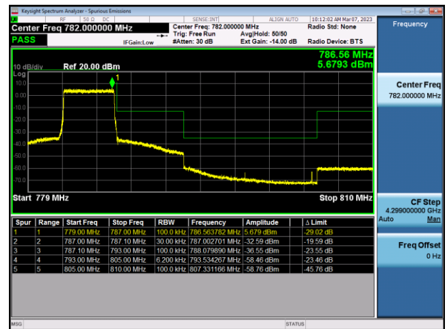
FDD13-10MHz-16QAM-MCH-1RB#0
