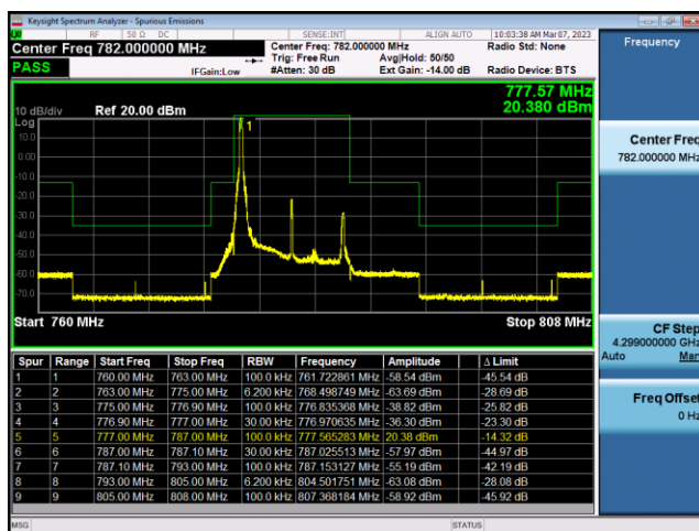
FDD13-10MHz-QPSK-MCH-1RB#49
