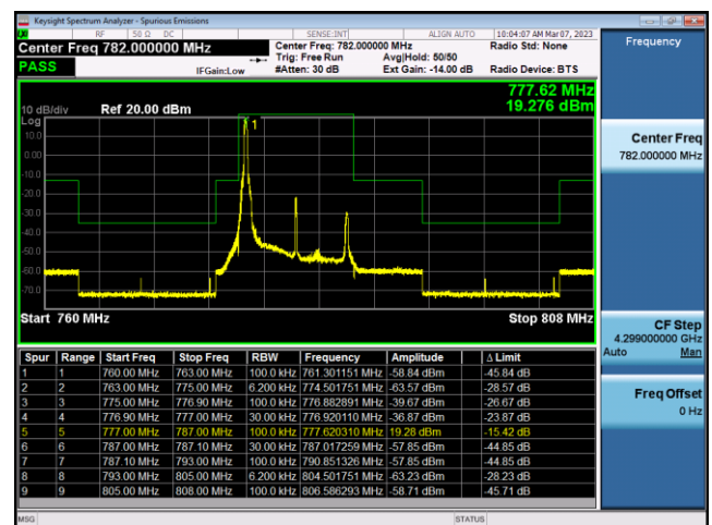
FDD13-10MHz-16QAM-MCH-1RB#49
