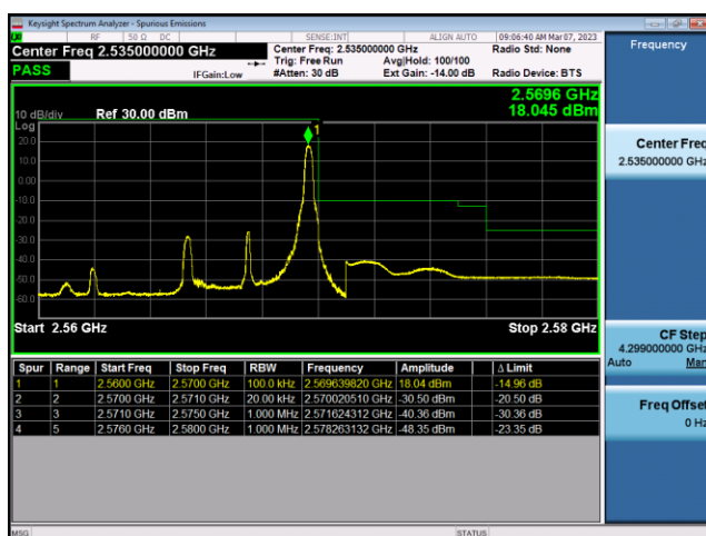
FDD7-5MHz-QPSK-HCH-1RB#24
