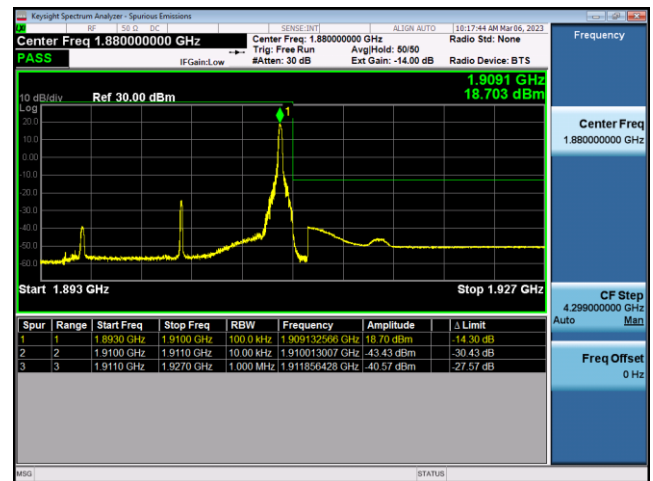
FDD2-15MHz-16QAM-HCH-75RB#0
