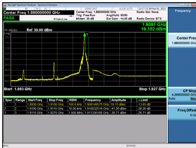
FDD2-15MHz-QPSK-HCH-75RB#0
