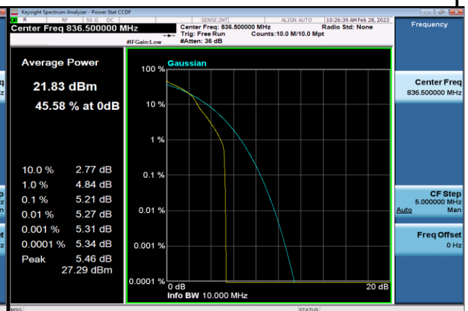
FDD05_MidRange_10MHz_836.5_OneRB _high_Q16
