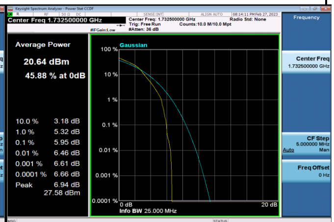
FDD04_MidRange_20MHz_1732.5_OneRB _high_Q16
