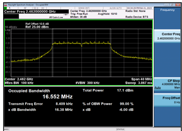
6dB Bandwidth-802.11g,2462MHz,Ant0
