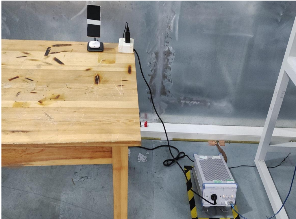
Radiated Emission below 1GHz-AC adapter charge mode
