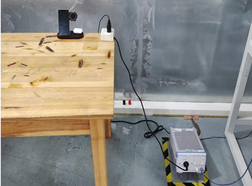
Conducted Emission-AC adapter charge mode
