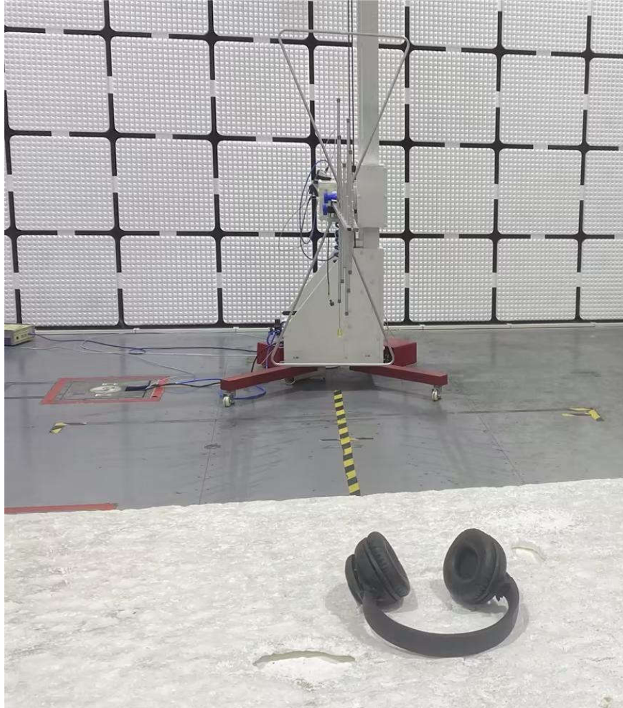
Radiated spurious emission Test Setup-1(Below 1GHz)
