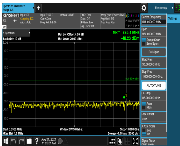
Band41-5MHz-16QAM-41215-1RB#0-Range1:30~1000MHz
