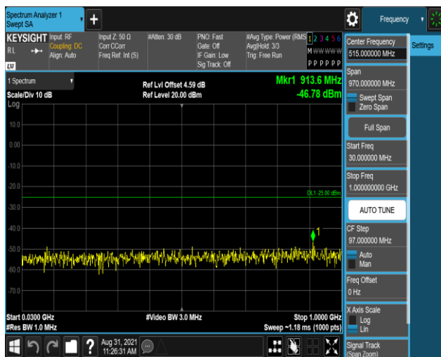
Band41-5MHz-16QAM-41215-1RB#0-Range1:30~1000MHz
