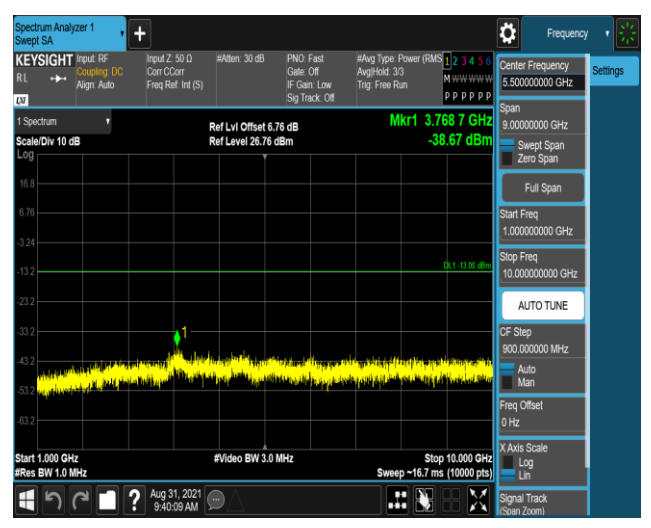
Band26-1.4MHz-16QAM-27033-1RB#0-Range2:1000 ~10000MHz
