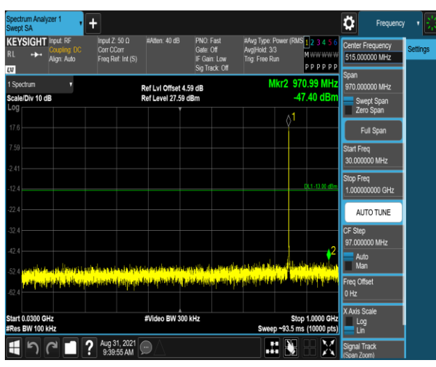
Band26-1.4MHz-16QAM-27033-1RB#0-Range1:30 ~1000MHz
