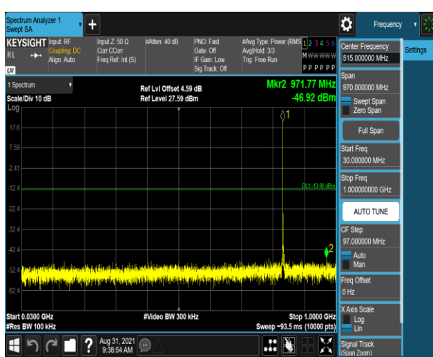
Band26-1.4MHz-16QAM-27033-1RB#0-Range1:30 ~1000MHz
