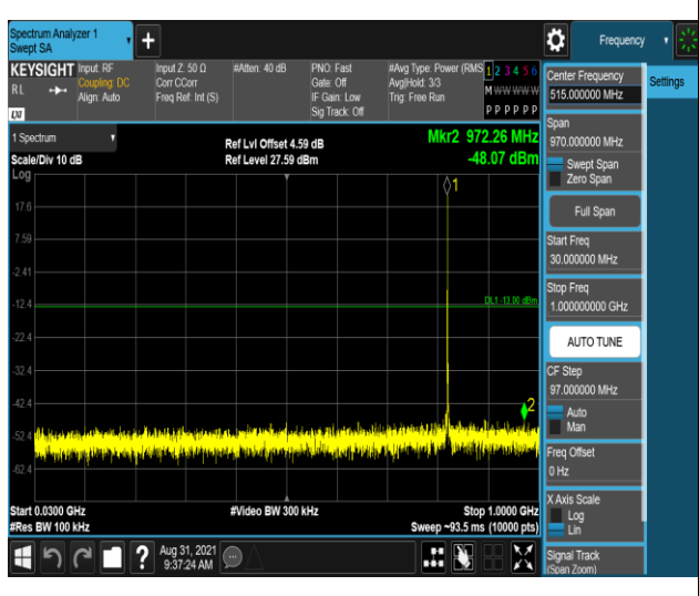
Band26-1.4MHz-QPSK-26797-1RB#0-Range1:30~1000MHz
