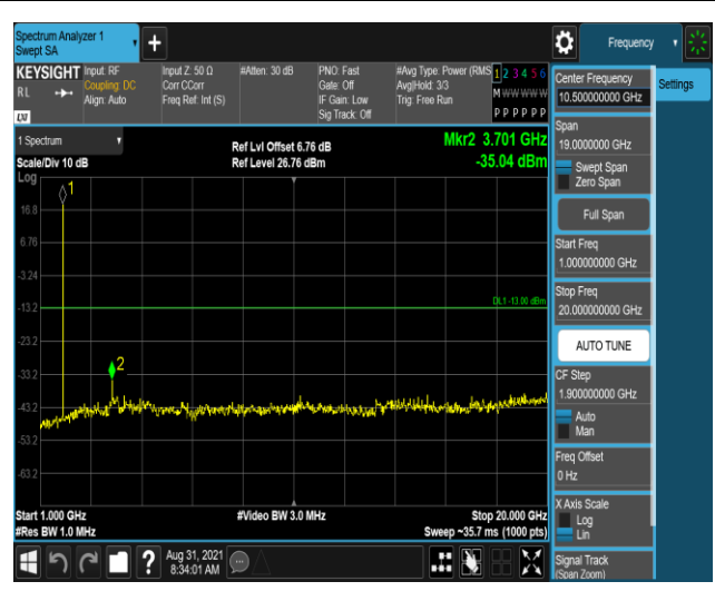
Band25-1.4MHz-16QAM-26047-1RB#0-Range1:30~1000MHz Band25-1.4MHz-16QAM-26047-1RB#0-Range2:1000~20000MHz
