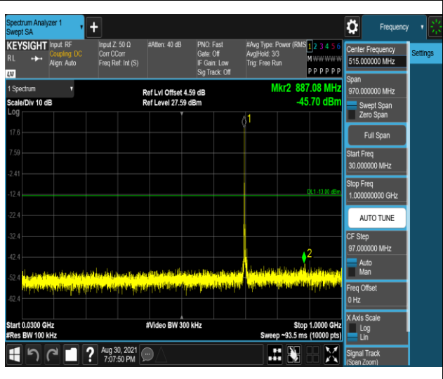
Band17-5MHz-16QAM-23755-1RB#0-Range1:30~1000MHz Band17-5MHz-16QAM-23755-1RB#0-Range2:1000~1000MHz
