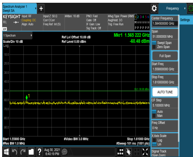
Band13-5MHz-QPSK-23205-1RB#0-Range3:1559~1610MHz 1610MHz
