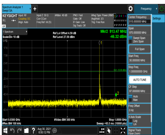
Band13-10MHz-QPSK-23230-1RB#0-Range1:30~1000MHz
