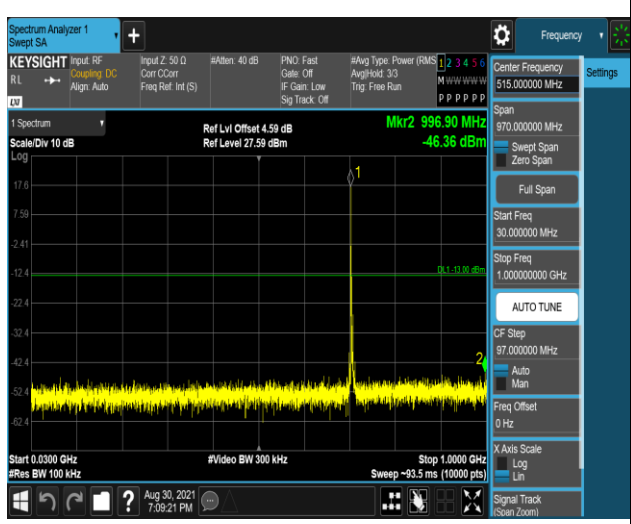
Band17-5MHz-16QAM-23755-1RB#0-Range1:30~1000MHz Band17-5MHz-16QAM-23755-1RB#0-Range2:1000~1000MHz
