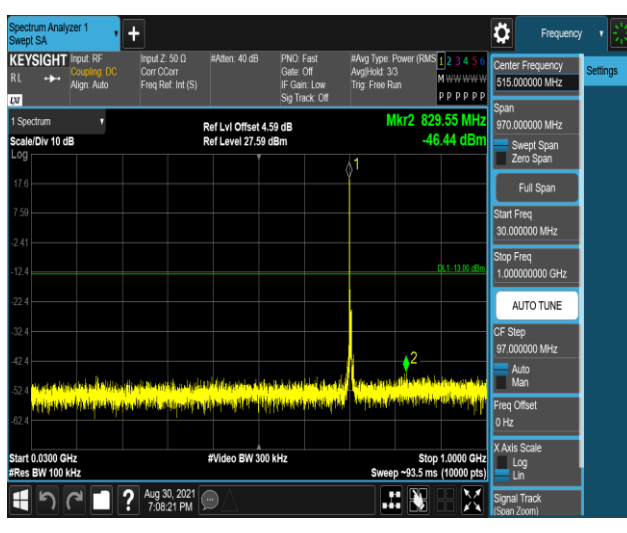
Band17-5MHz-QPSK-23790-1RB#0-Range1:30~1000MHz Band17-5MHz-QPSK-23790-1RB#0-Range2:1000~1000MHz
