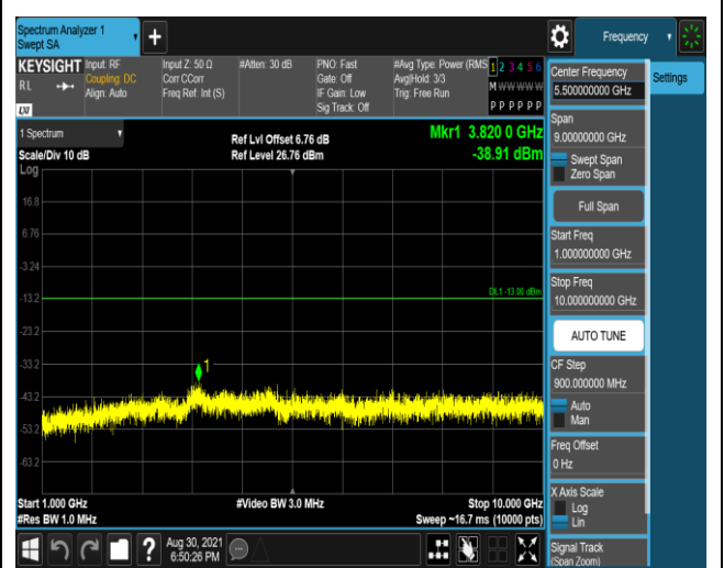
Band13-10MHz-QPSK-23230-1RB#0-Range2:1000~10000MHz
