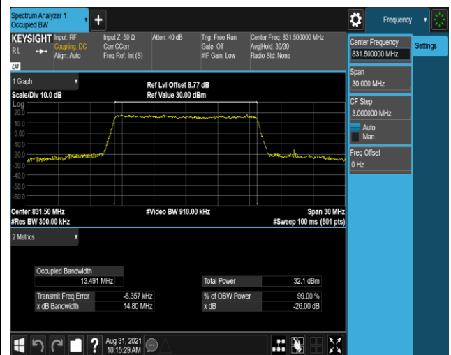
Band26-15MHz-QPSK-26865-75RB#0
