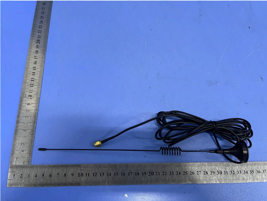
Photo 9 LoRa Antenna 3
